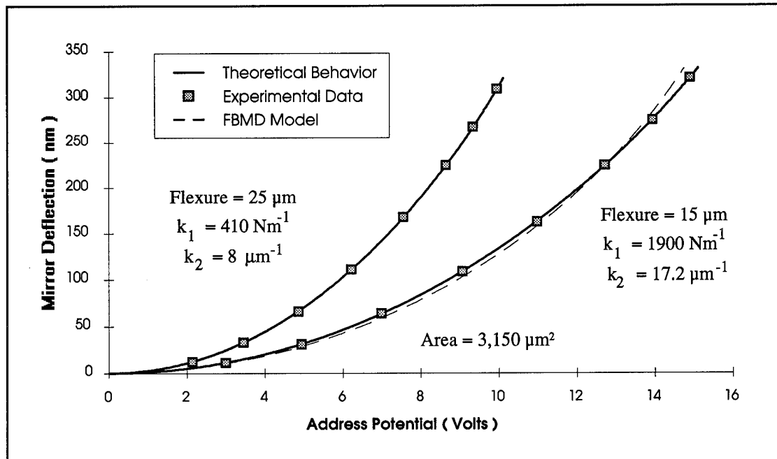
Figure 5-9. Ideal characteristic behavior of two paddle-style Cantilever devices.
