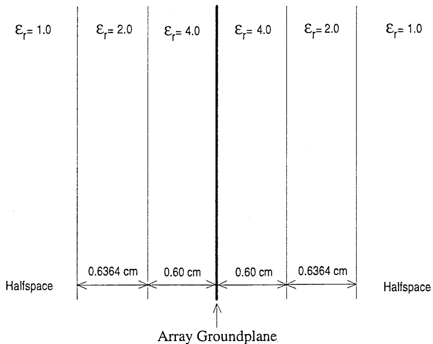
Figure 4.9 Horizontal Slot Geometry: Slot Length=0.75 cm, Slot Width=0.075 cm, D_x=1.125\text{ cm} , D_z=0.675\text{ cm} , Frequency=10 GHz.
