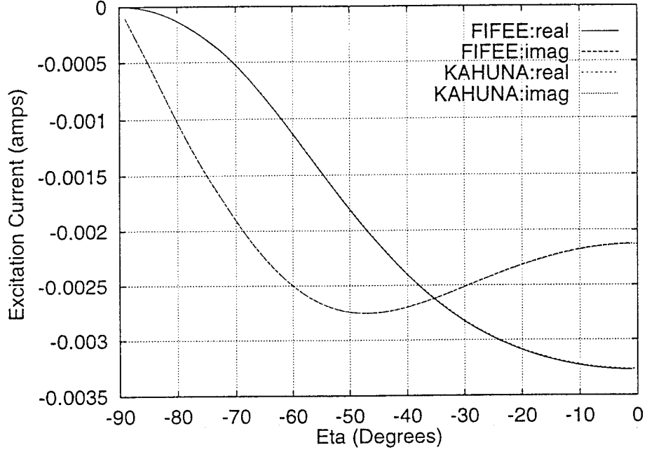
Excitation Current for z-Directed Slot at Origin, 10 GHz, TE z , 2 Slabs in Region I
