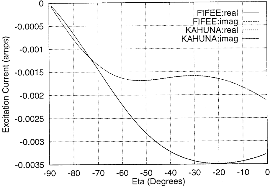
Excitation Current for z-Directed Slot at (x,z)=(0.28,0.0)cm, 10 GHz, TE z , 2 Slabs in Region I
