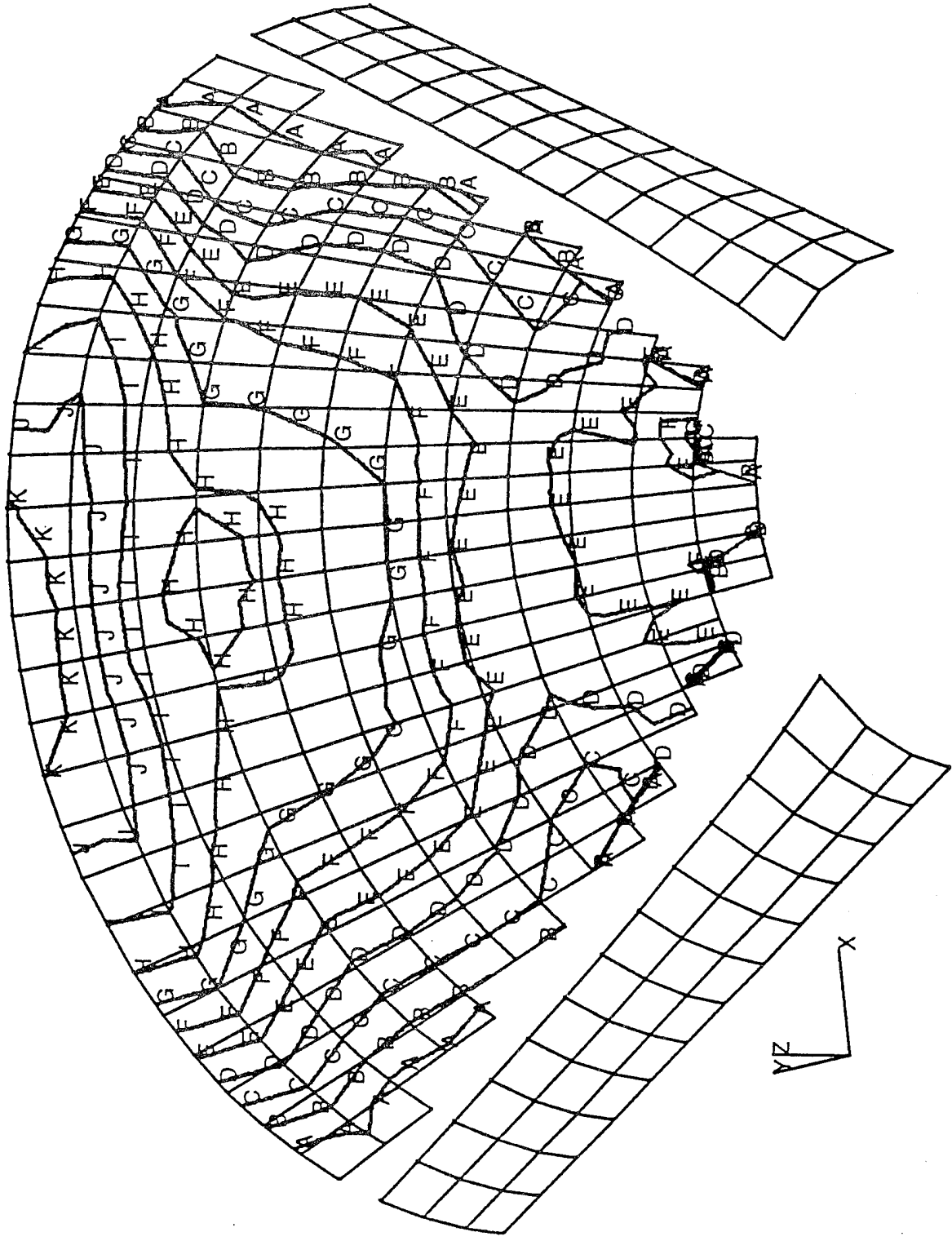
Figure 30. Typical Cone Thickness Results
