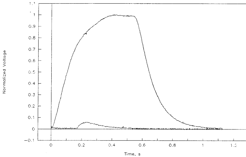
Fig. A-1. Normalized Voltage Versus Time For 10 ms Primary Pulse and 500 ms Secondary Pulse.
