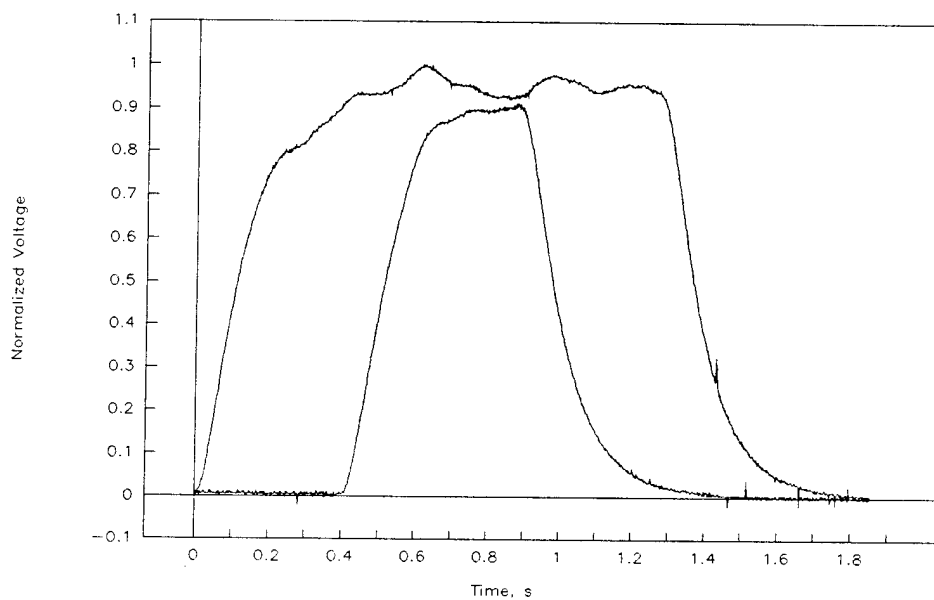
Fig. A-7. Normalized Voltage Vs Time For 500 ms Primary Pulse and 1.30 s Secondary Pulse.
