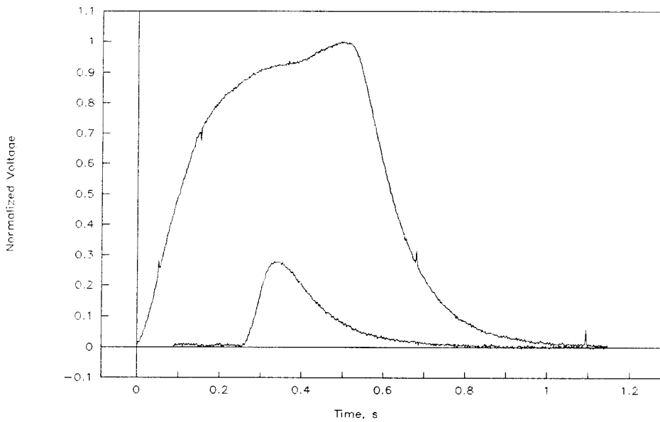
Fig. A-2. Normalized Voltage vs Time For 50 ms Primary Pulse and 500 ms Secondary Pulse.
