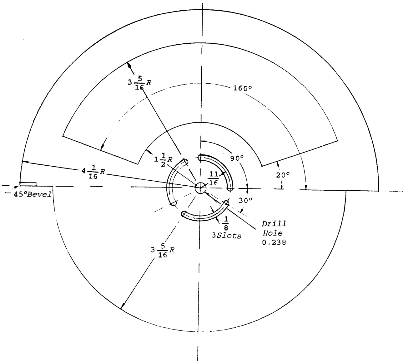
Fig. 3. Balanced Chopper Blade Part A.
