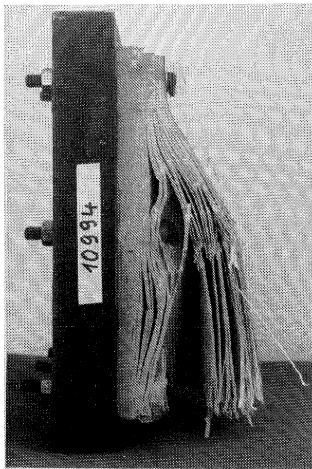
b) Side view, showing the delamination
