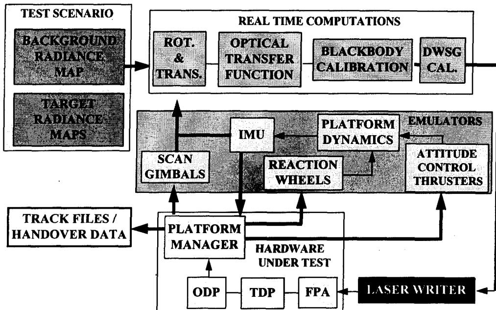
Figure 16. Closed-loop T&E implemented using FPATC.
