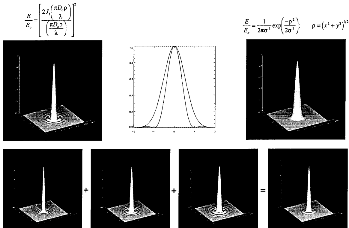
Figure E-14. Illustration of the concept of an effective PSF resulting from a number of contributing sources such as broadband radiation, optical diffraction, deterministic and stochastic jitter and resulting blur, or other sources.
