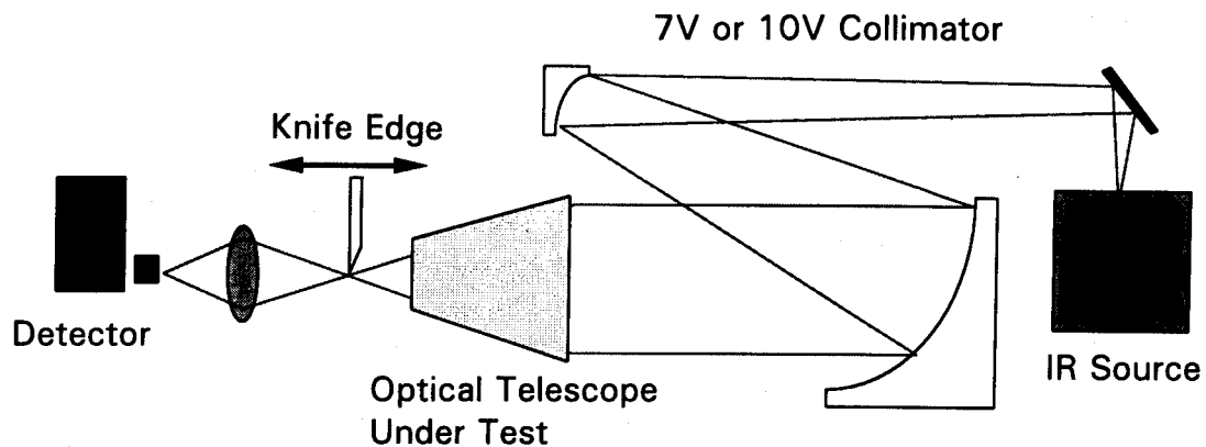
Figure B-1. Schematic of test setup #1.
