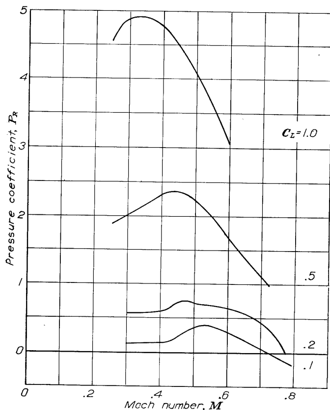
FIGURE 14.—Variation of resultant pressure coefficient, with Mach number for orifice B-3, measured in power-on flight.
