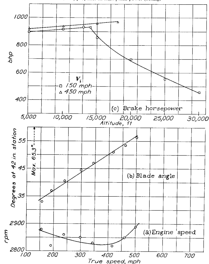
FIGURE 10.—Engine speed, propeller-blade angle, and brake horsepower for a power setting of 39 inches of mercury and 2600 rpm.
