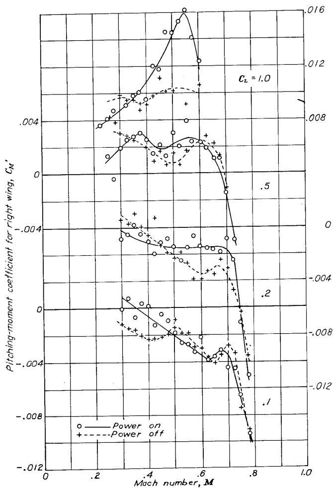
FIGURE 20.—Variation of right-wing-panel pitching-moment coefficient with Mach number.
