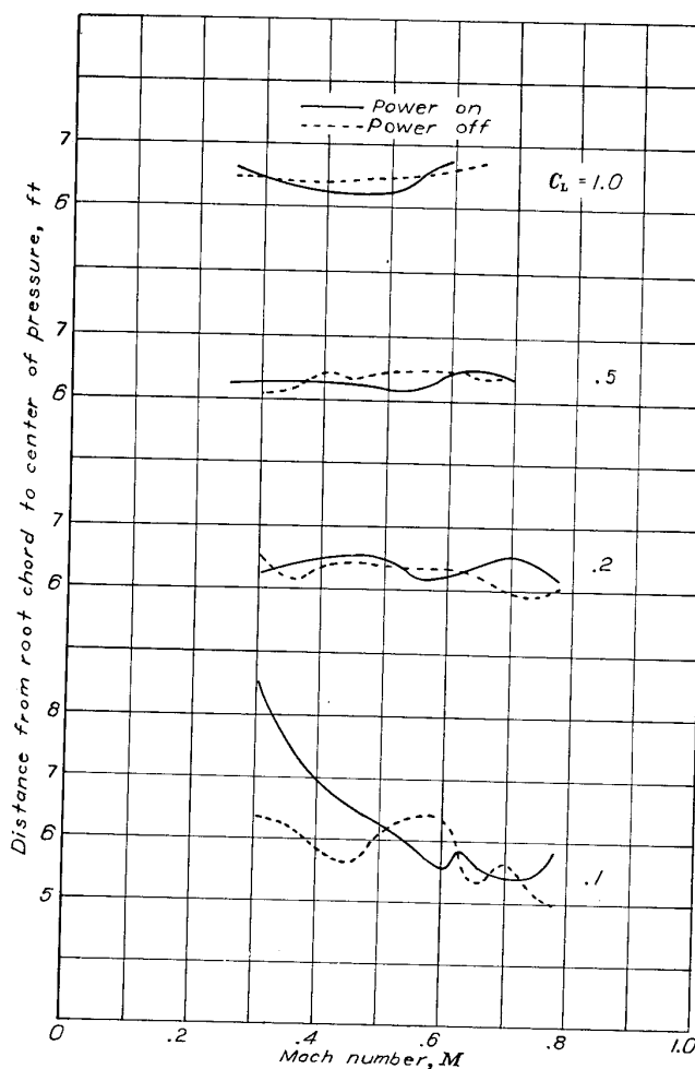
FIGURE 19.—Variation of lateral distance from root chord to center of pressure of right-wing panel with Mach number.
