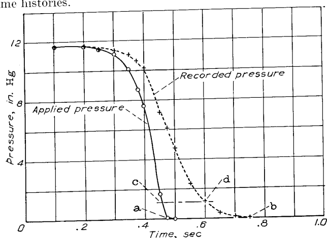
FIGURE 24.—Time history of pressure lag in typical aileron line.
