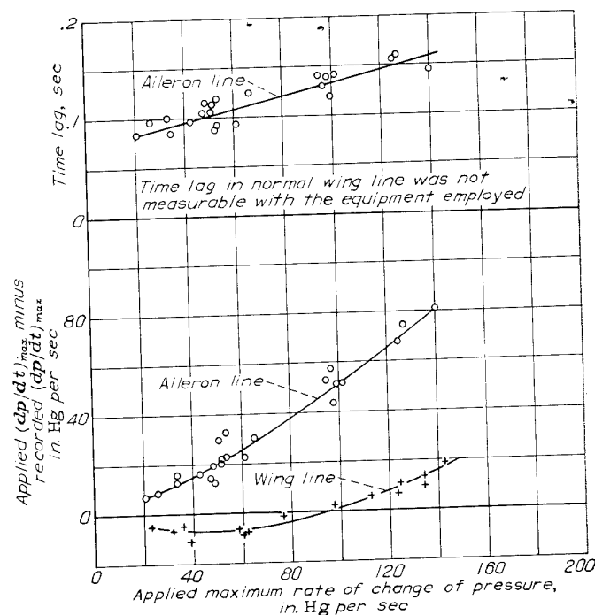
FIGURE 25.—Lag in typical wing pressure lines.
