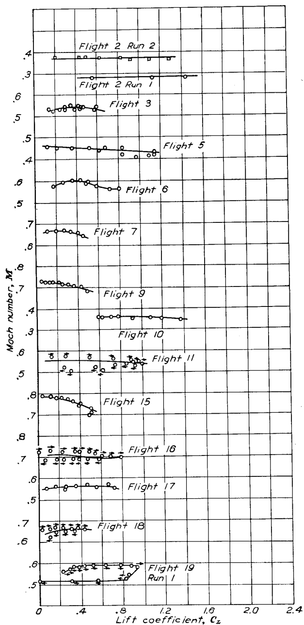
FIGURE 13.—Variation of Mach number with airplane lift coefficient during the power-on test flights.
