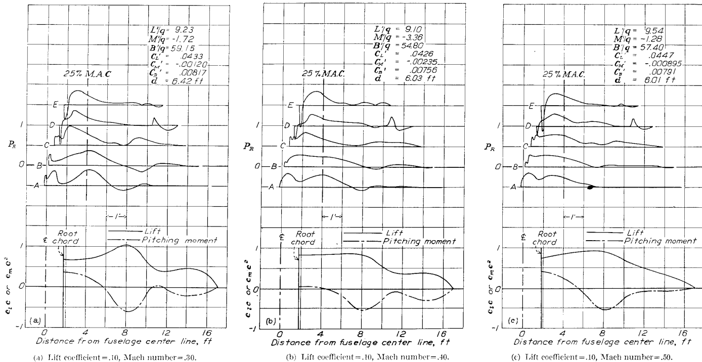
FIGURE 16.—Pressure distribution on the right wing in power-off flight.
