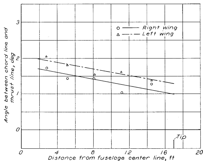
FIGURE 5.—Incidence and geometric twist of the wings.
