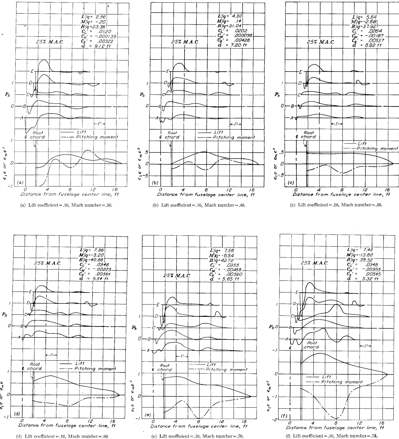
FIGURE 15.—Pressure distribution on the right wing in power-on flight.
