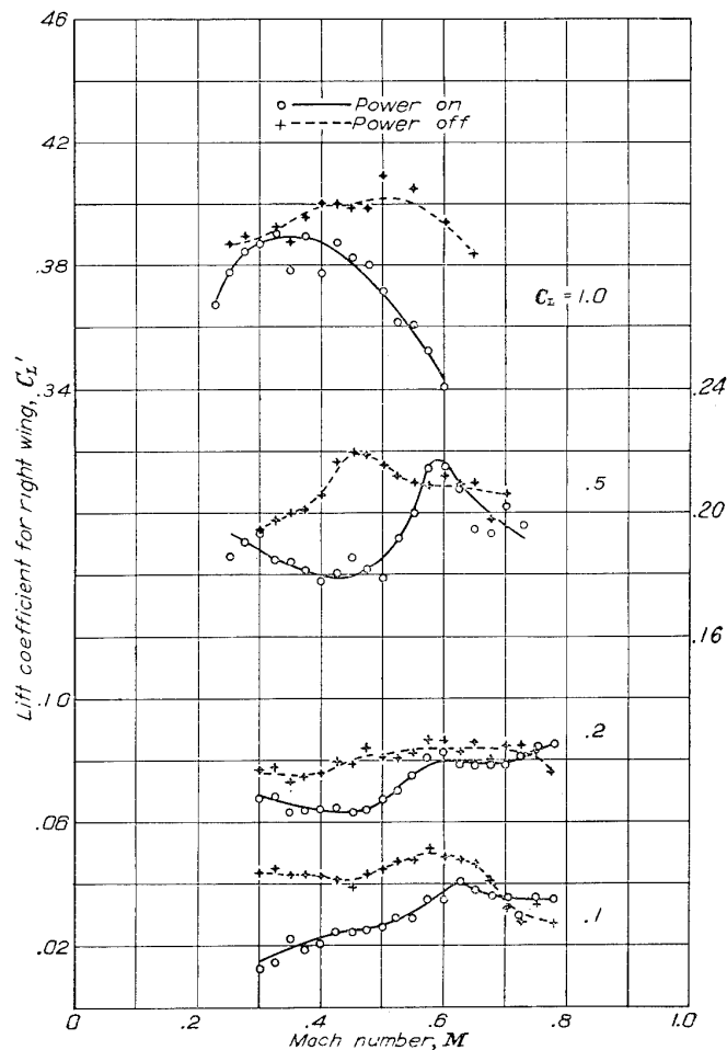
FIGURE 17.—Variation of right-wing-panel lift coefficient with Mach number.
