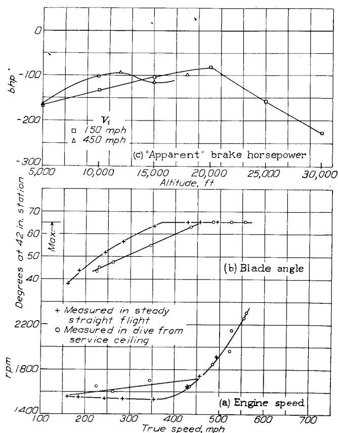
FIGURE 9.—Engine speed, propeller-blade angle, and brake horsepower for the engine-throttled, propeller-in-high-pitch power setting.
