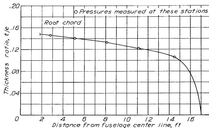
FIGURE 4.—Variation of thickness ratio along span of right wing.
