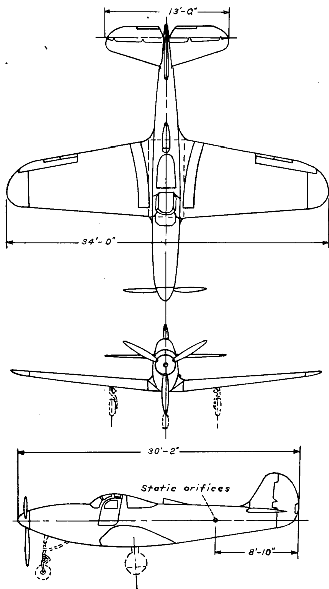
FIGURE 3.—Three-view drawing of the test airplane.
