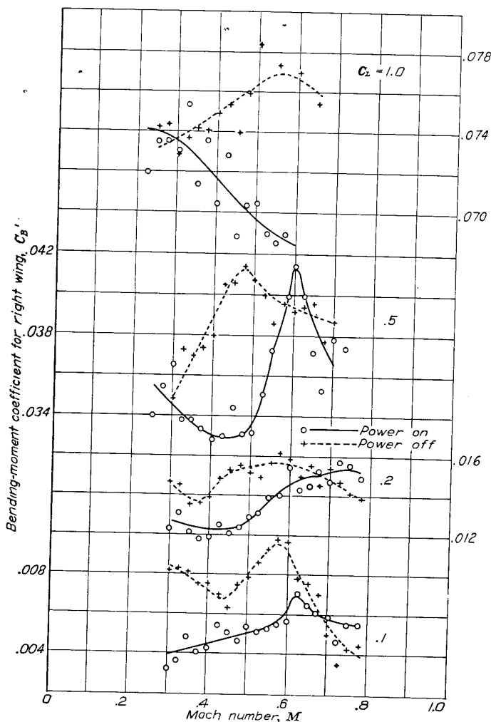
FIGURE 18.—Variation of right-wing-panel bending-moment coefficient with Mach number.
