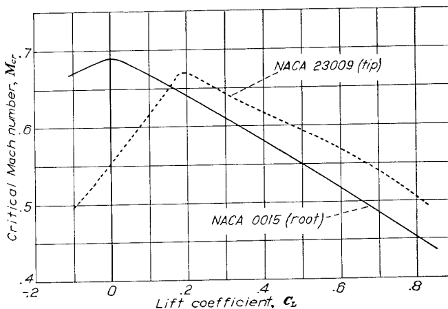
FIGURE 21.—Calculated values of critical Mach number for the specified root and tip wing sections.
