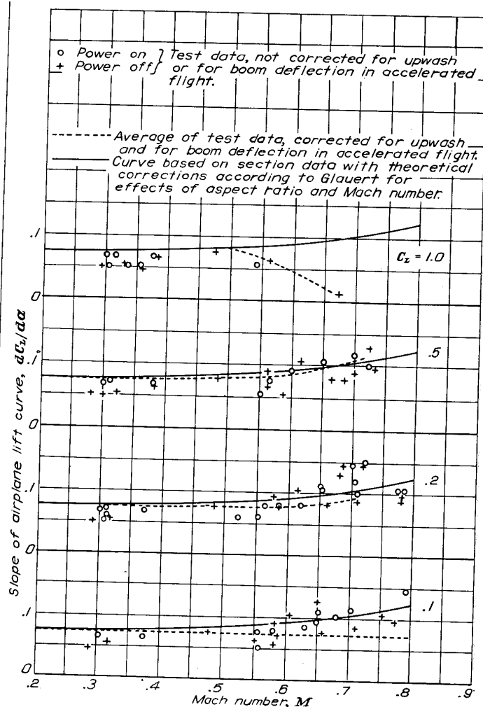
FIGURE 23.—Variation of slope of the airplane lift curve with Mach number.
