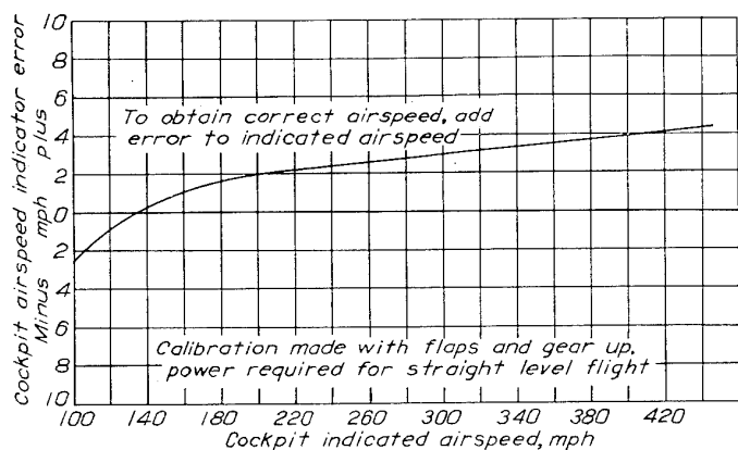
FIGURE 6.—Calibration of service airspeed-measuring system.
