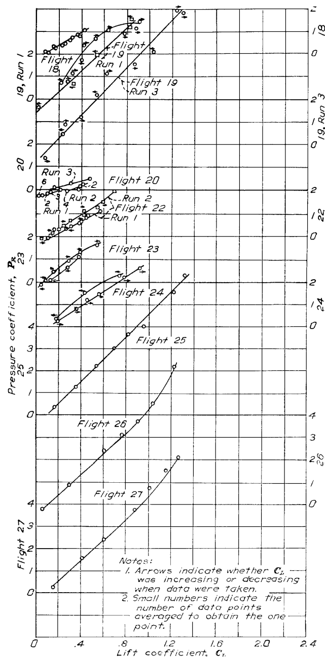
FIGURE 12.—Variation of resultant pressure coefficient for orifice station E-3 with airplane lift coefficient during the power-on test flights.
