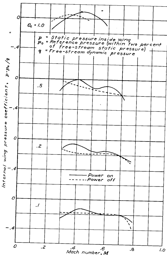
FIGURE 22.—Variation of wing internal-pressure coefficient with Mach number.
