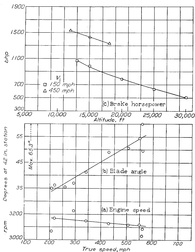
FIGURE 11.—Engine speed, propeller-blade angle, and brake horsepower for a power setting of full throttle and 3000 rpm.
