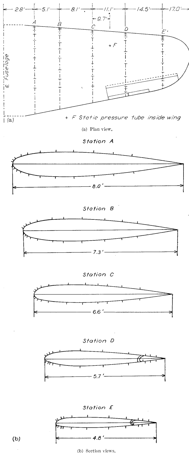
FIGURE 7.—Orifice locations on right wing.
