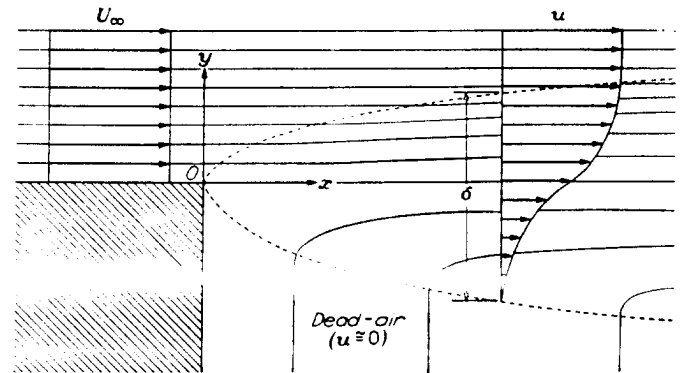
FIGURE 1.—Schematic drawing of the flow.
