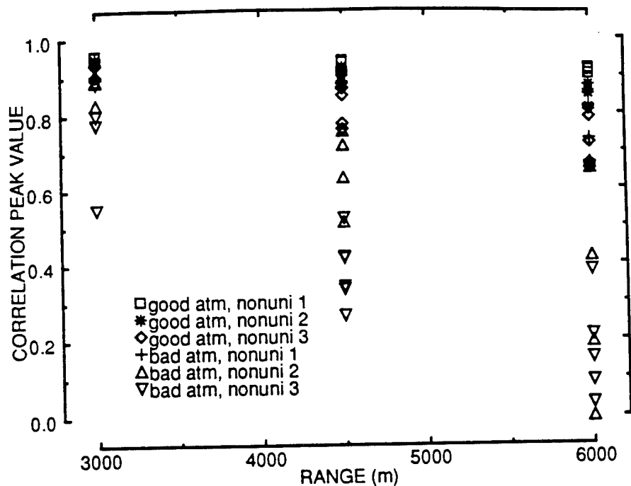
Figure 28. Atmosphere plus nonuniformity
