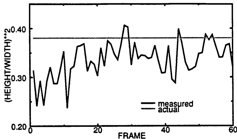
Figure 1. Frame to frame variations of the (height/width) 2 ratio for 60 consecutive frames of first generation FLIR imagery
