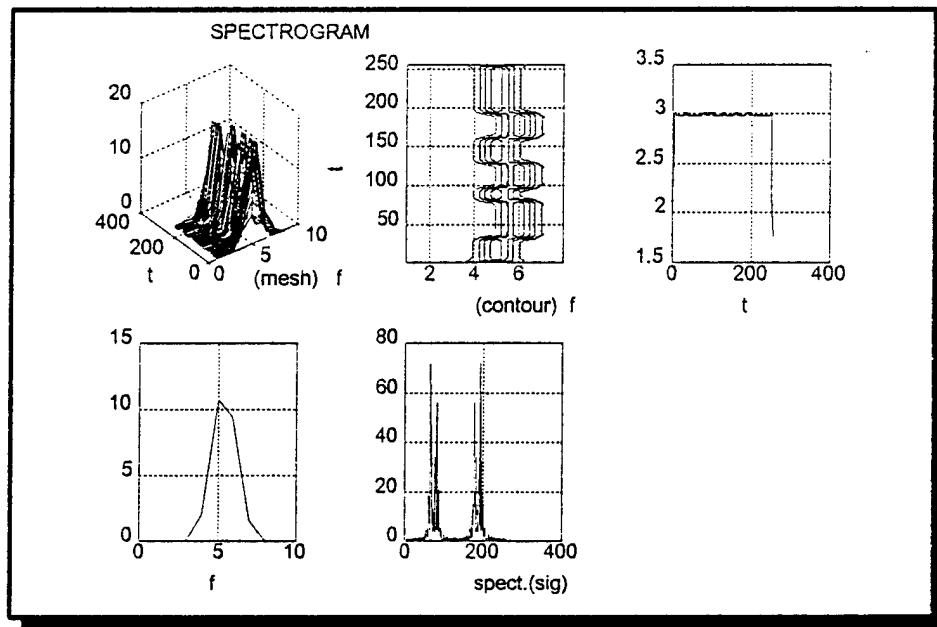
Figure 4.30: FSK Spectrogram (Window Length is 16)
