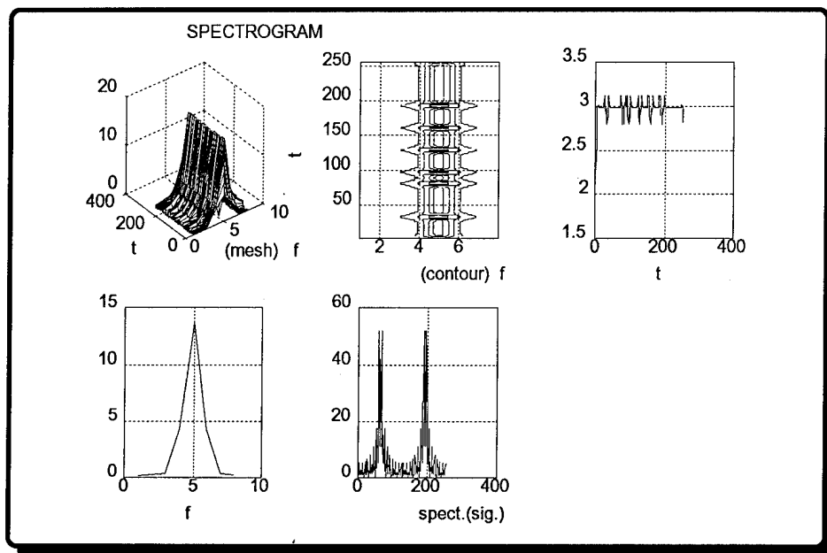
Figure 5.2: BPSK Spectrogram ( Infinite SNR)
