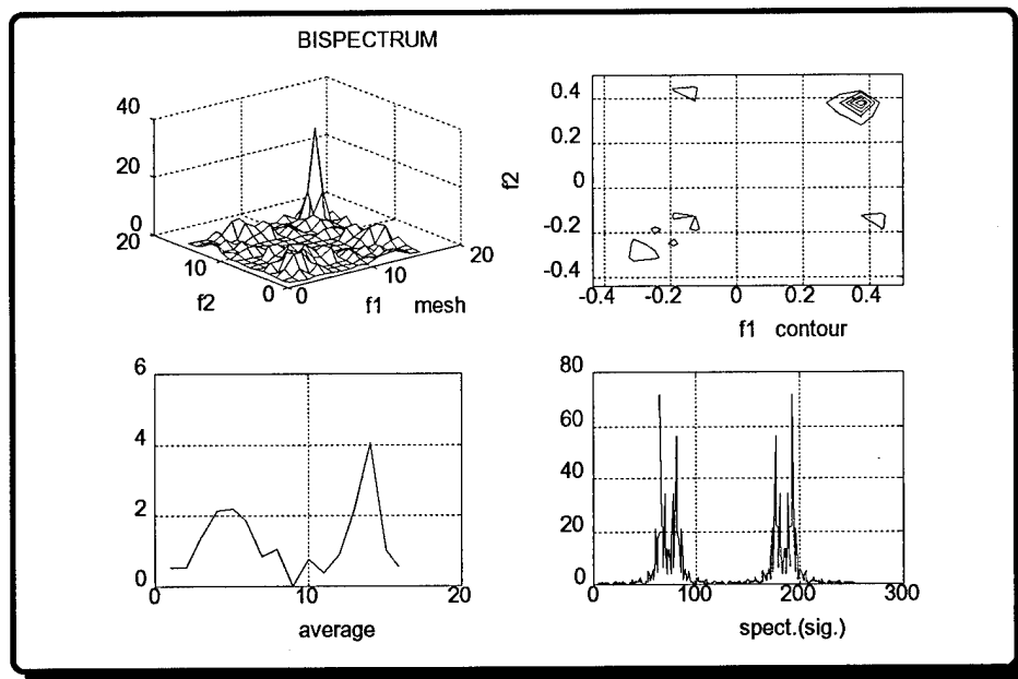
Figure 5.43: FSK Bispectrum (Infinite SNR)
