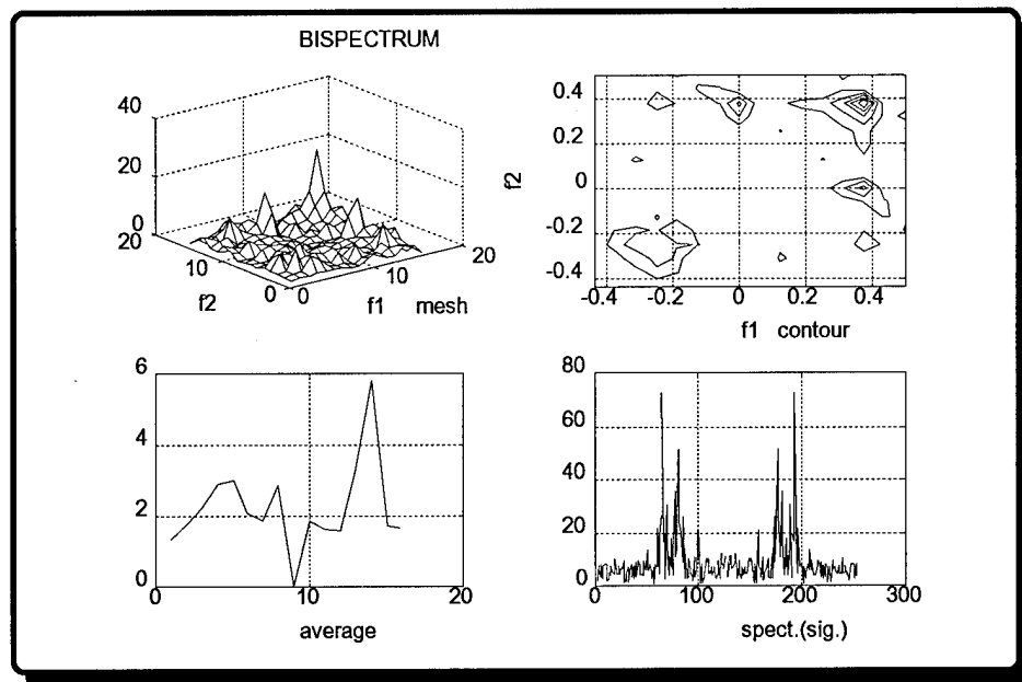
Figure 5.47: FSK Bispectrum (SNR= +5 dB)
