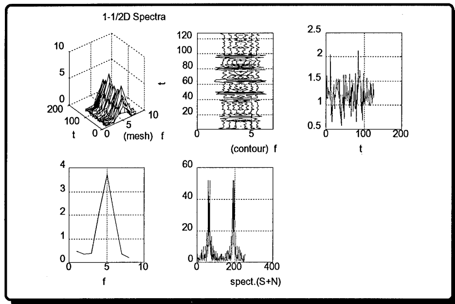
Figure 5.9: BPSK 1-1/2D Spectra (SNR= +20 dB)
