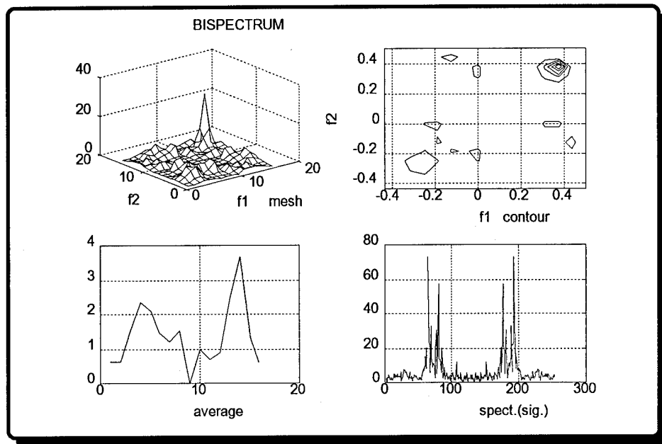
Figure 5.46: FSK Bispectrum (SNR= +10 dB)
