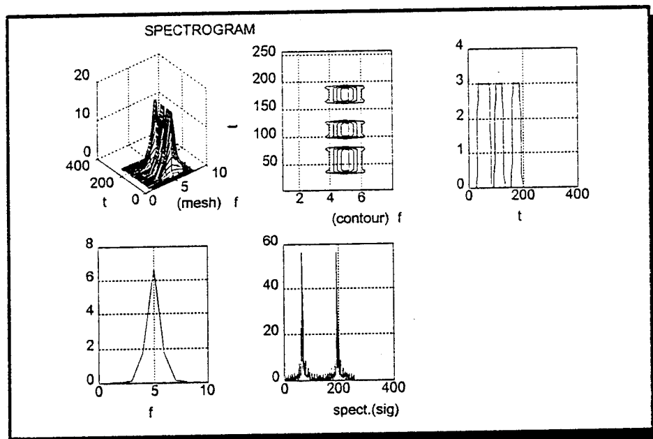
Figure 4.56: OOK Spectrogram (Window Length is 16)
