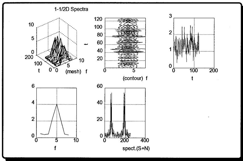
Figure 5.10: BPSK 1-1/2D Spectra (SNR= +15 dB)
