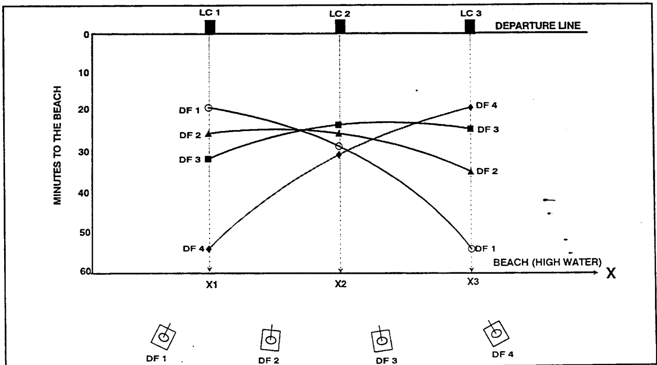
Figure 3-2. DFUs Engagement Diagram
