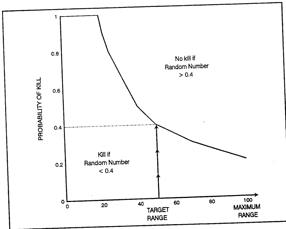
Figure 3-3. Probability of Kill
