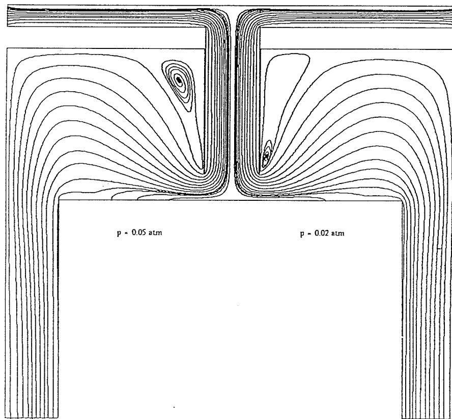
Fig. 19 Flow streamlines in SiC deposition. Left: 0.05 atm. Right: 0.02 atm. See comments on Fig. 18.
