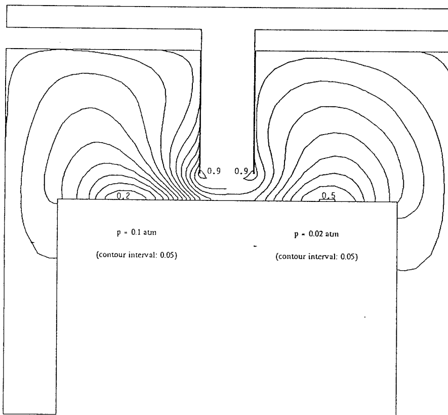
Fig. 21 Mass fraction of MTS in SiC deposition. Left: 0.1 atm. Right: 0.02 atm. Contour interval = 0.05.
