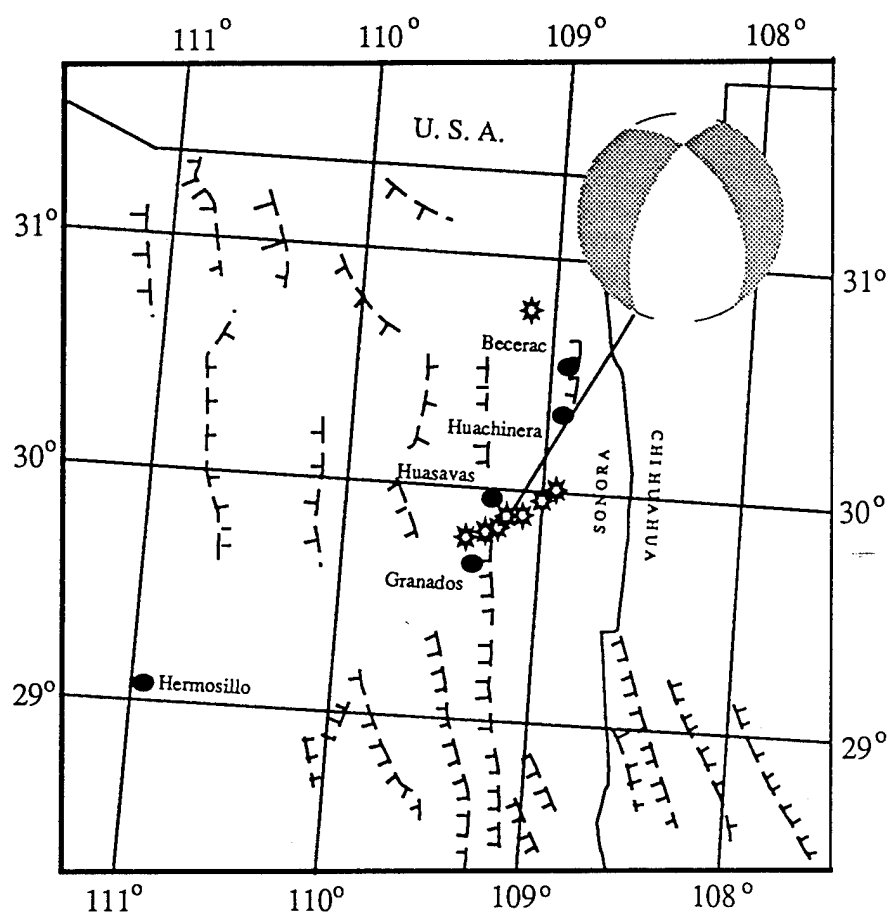
Figure 1. Events of the October 1994 swarm overlaying a simplified tectonic map of Mexico. The events of the swarm are marked with stars. One can see general east - northeast trend of the events. The 1887 Great Sonoran Earthquake is represented by a star north of the swarm. The cities mentioned in the text are marked with black circles.
