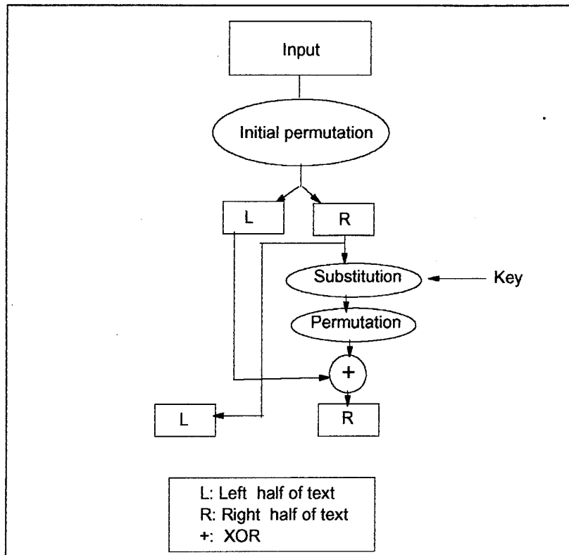
Figure 3.1 Initial Permutation and Round 1 of the DES [Ref. 19]
