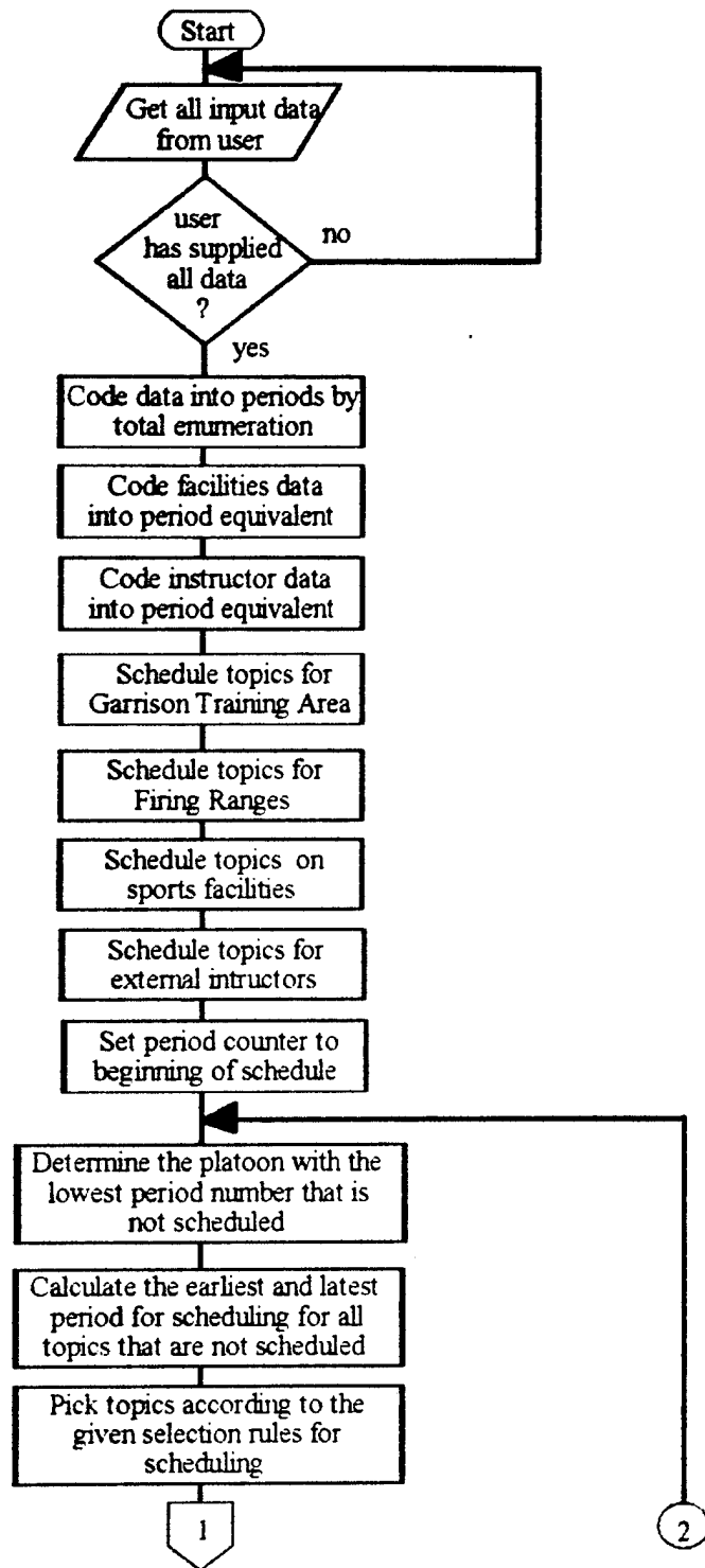
Figure 1a: Flowchart of Complete Scheduling Algorithm
