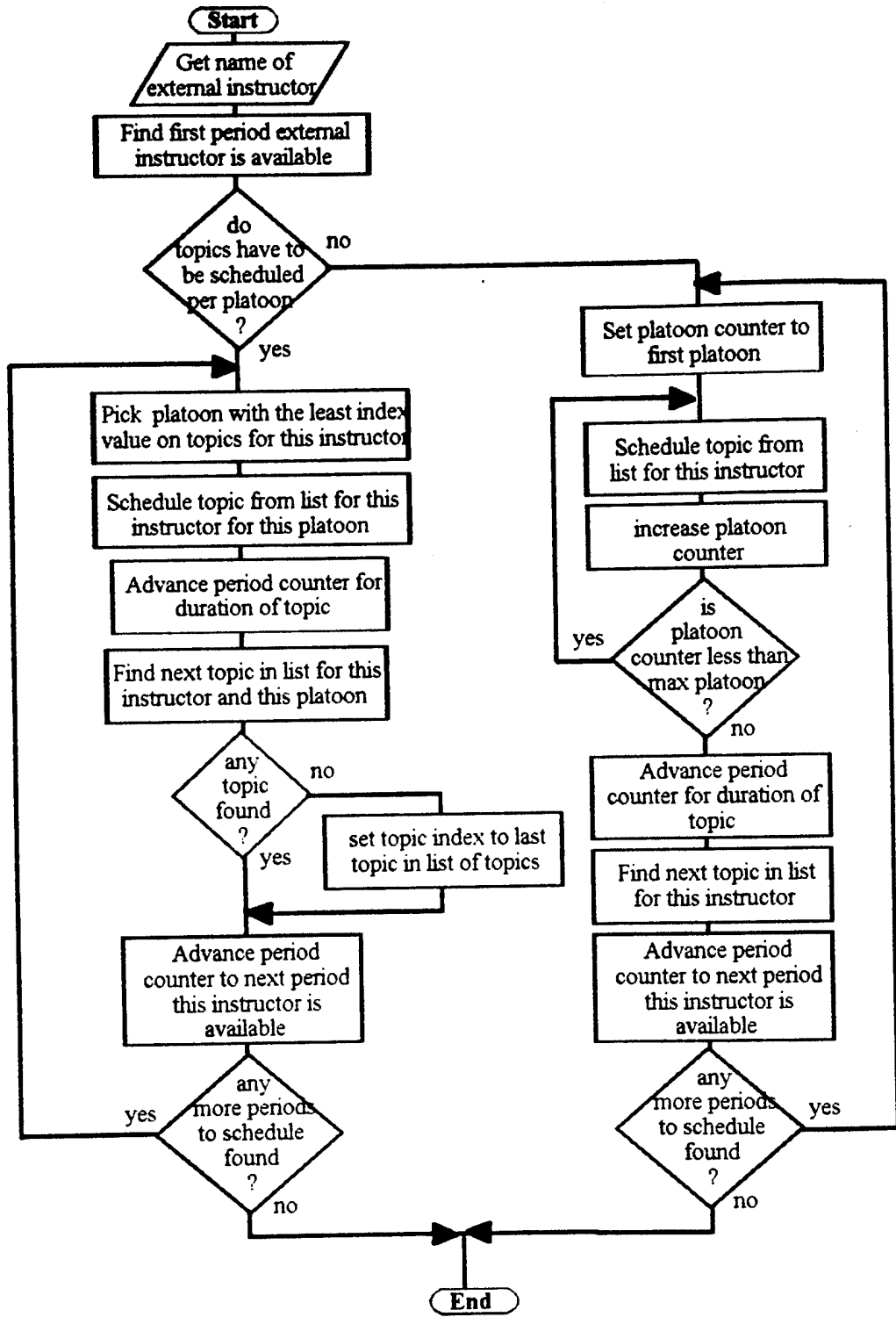
Figure 3: Flowchart for Scheduling Algorithm for External Instructors
