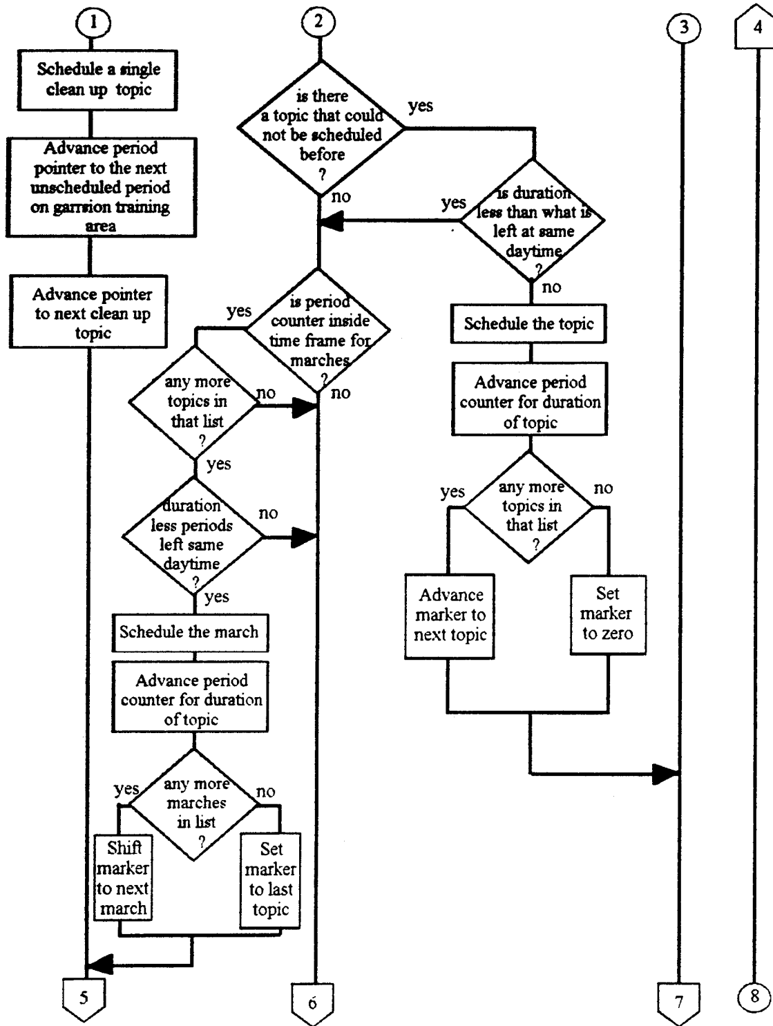
Figure 4b: Flowchart of Scheduling Algorithm For Garrison Training Area (Continued)
