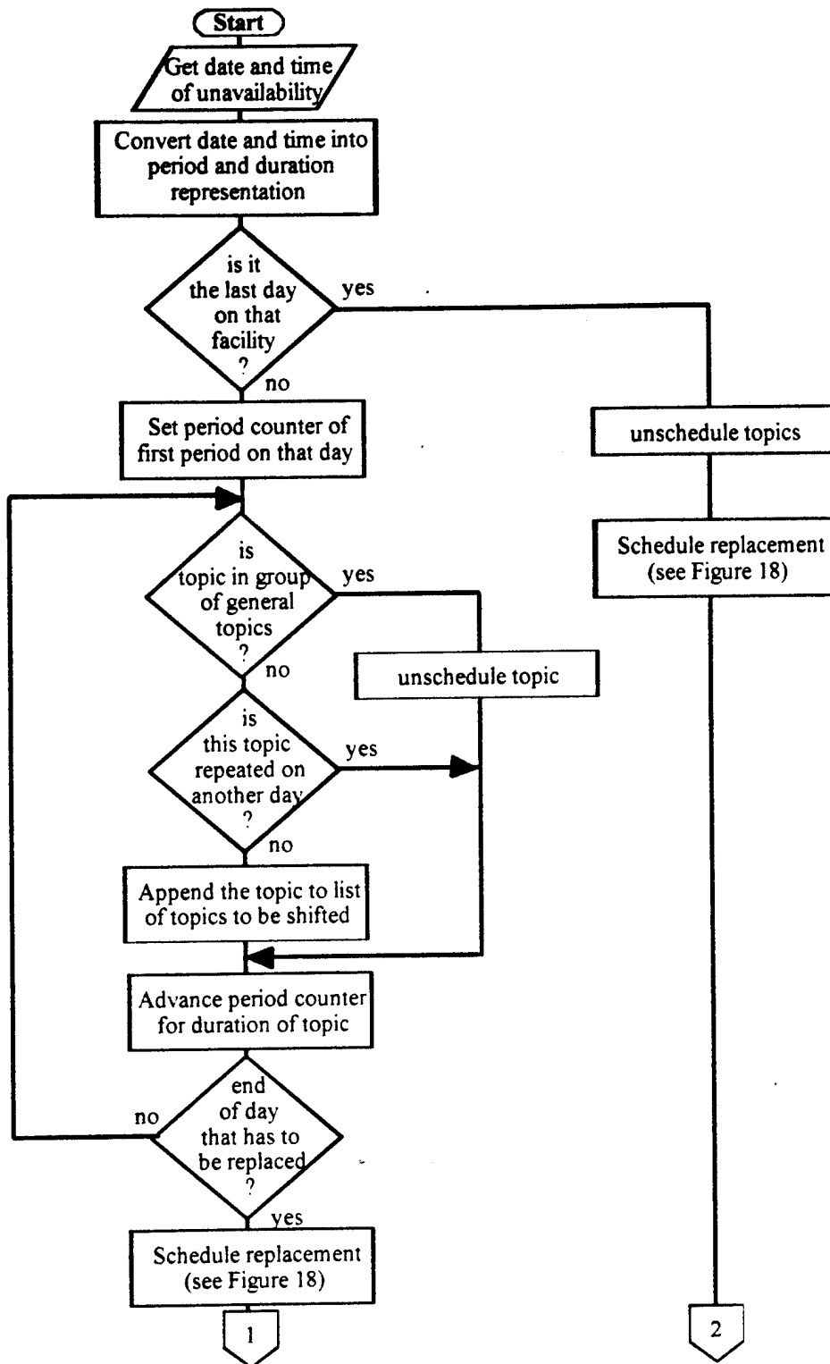
Figure 17a: Flowchart of Algorithm To Handle Facility Unavailability (Garrison Training Area or Firing Range)
