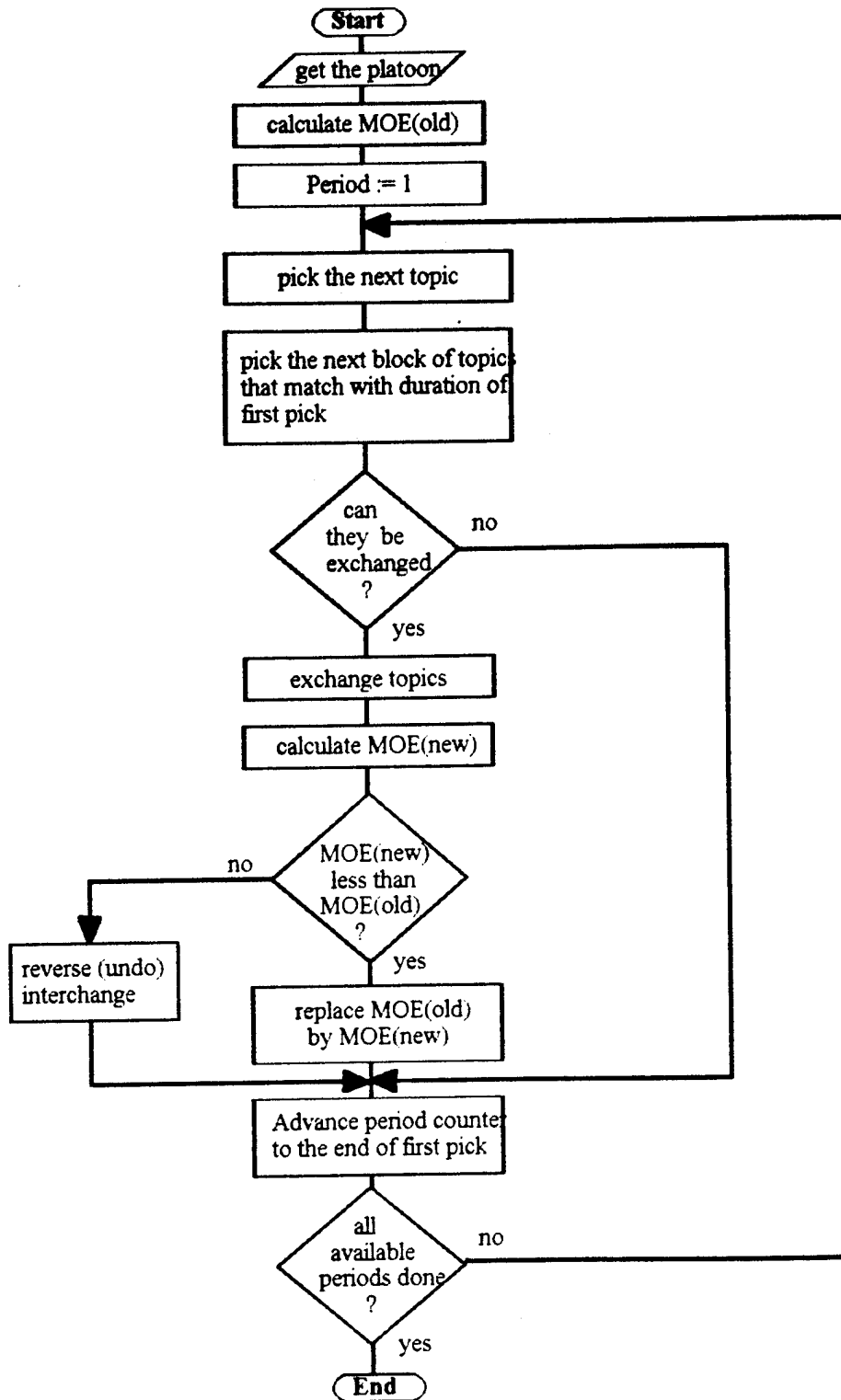
Figure 6: Flowchart of Improvement Algorithm
