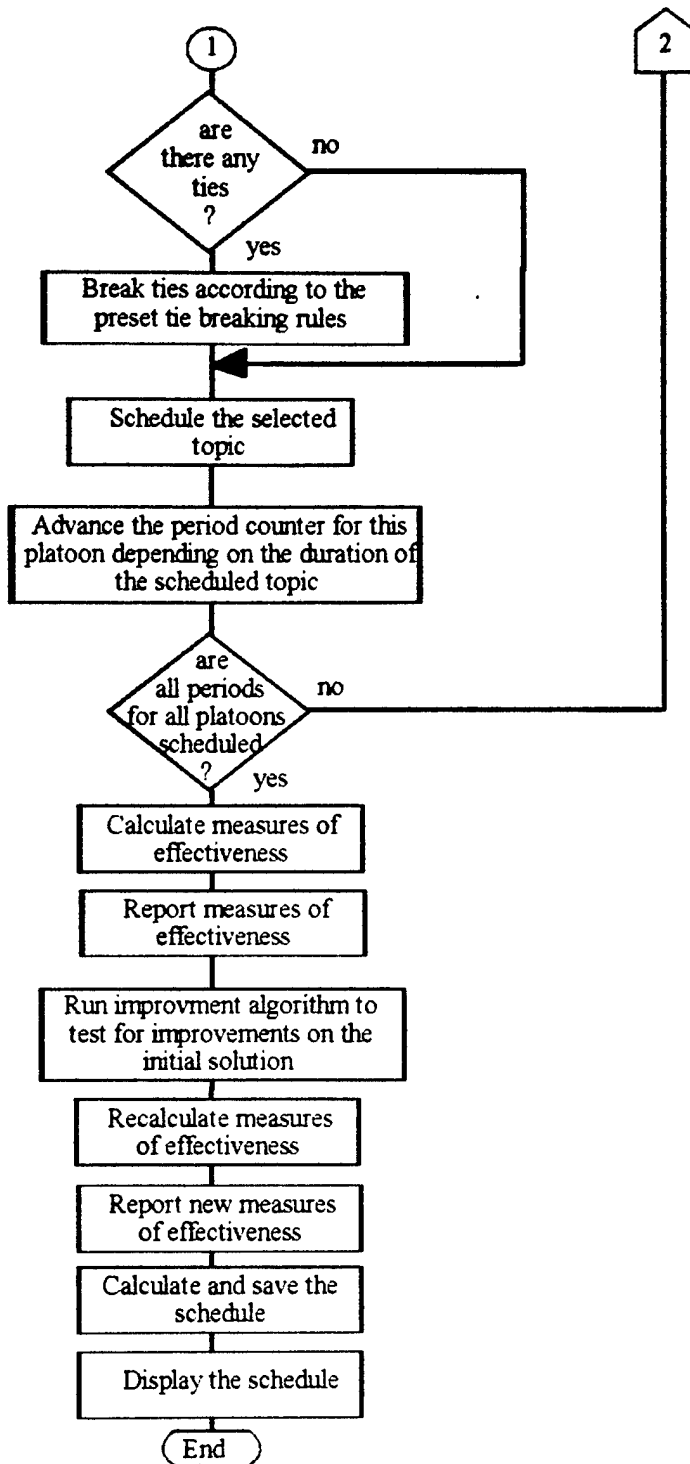
Figure 1b: Flowchart of Complete Scheduling Algorithm (Continued)
