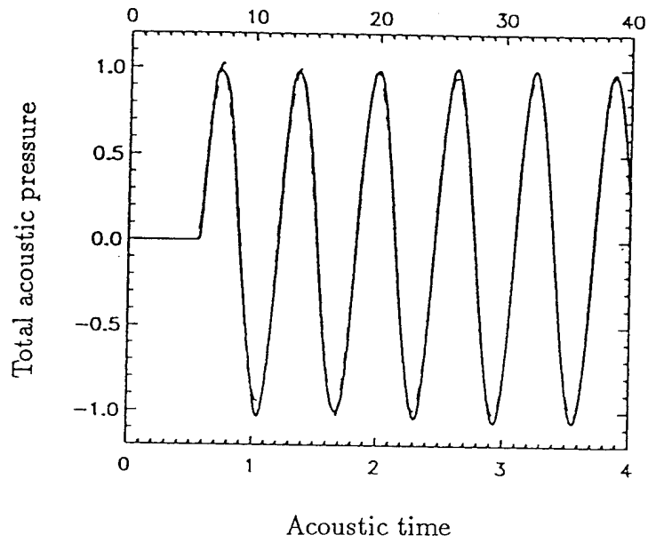
Time scale used by Wang and Kassoy
