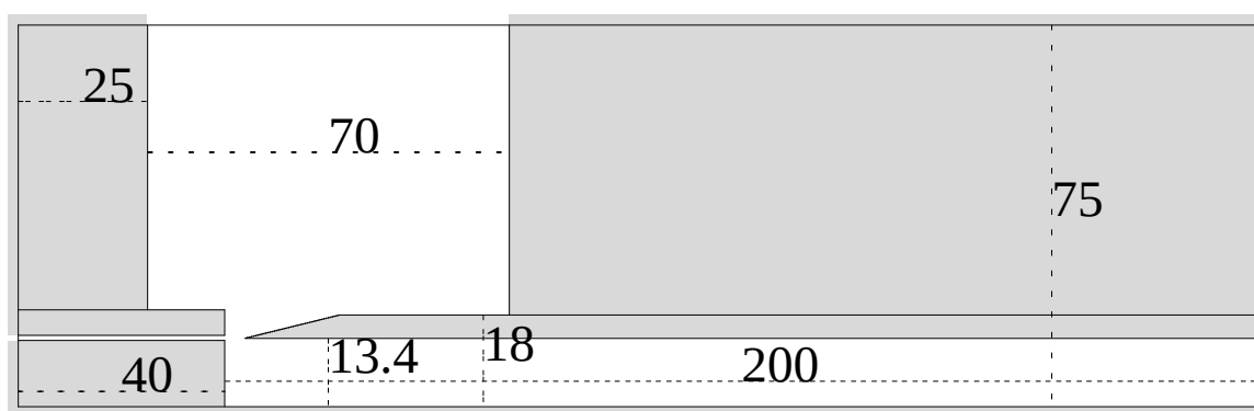
Figure 7-1: Soprano recorder flue, 20 cm closed-end pipe. The numbers shown correspond to millimeters. Inlet is at the left, outlet is at the top of the picture.
