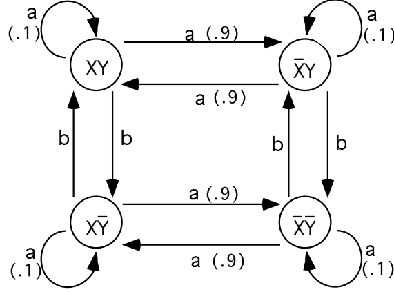
Figure 3-6: A probabilistic environment
