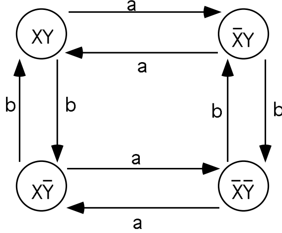
Figure 3-4: A deterministic environment
