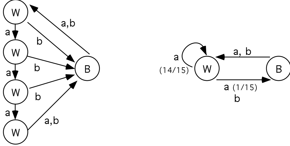
Figure 3-5: An example of a deterministic underlying environment and the corresponding non-deterministic perceived environment
