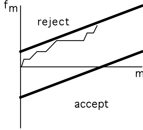
Figure 6-1: A graphical depiction of a typical sequential ratio test
