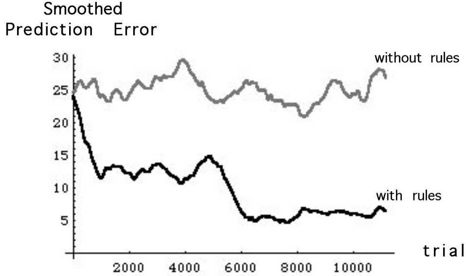
Figure 3-12: A graph of the smoothed error values as the agent learns the OV relation (the black line) compared with the smoothed error for an empty model (the gray line). To make this graph the prediction errors that the agent makes are further smoothed by averaging a window of 1000 trials. The agent is learning NOACTION rules only in the first 5000 trials.
