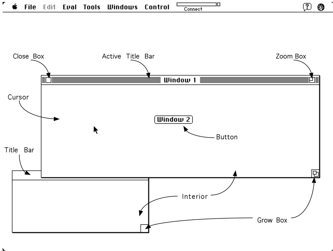
Figure 2-1: A description of a Macintosh screen situation
