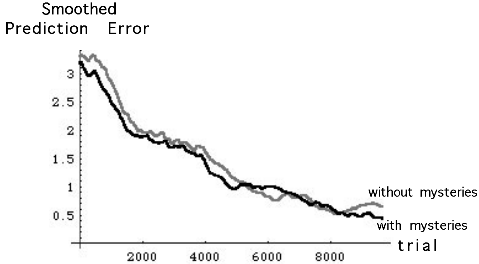
Figure 3-18: A graph of the smoothed error values as the agent learns the EXIST relation with mysteries (the black line) compared with the smoothed error when the error learns without mysteries (the gray line). To make this graph the prediction errors that the agent makes are further smoothed by averaging a window of 1000 trials.
