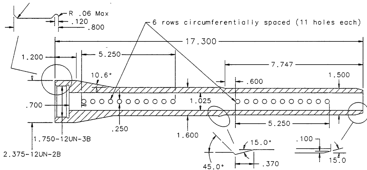
Figure 3. Holed Barrel Extension (Dimensions in Inches).
