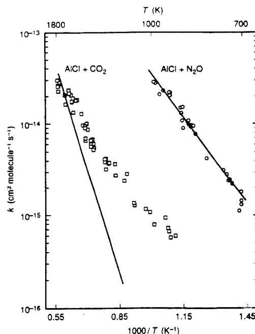
Figure 2. Arrhenius plots of experimental rate coefficients for the AlCl + N 2 O (open circles) and AlCl + CO 2 (open squares) reactions. Rate coefficient expressions for the O atom abstraction channels for these reactions derived using the MTST method are shown as solid lines.
