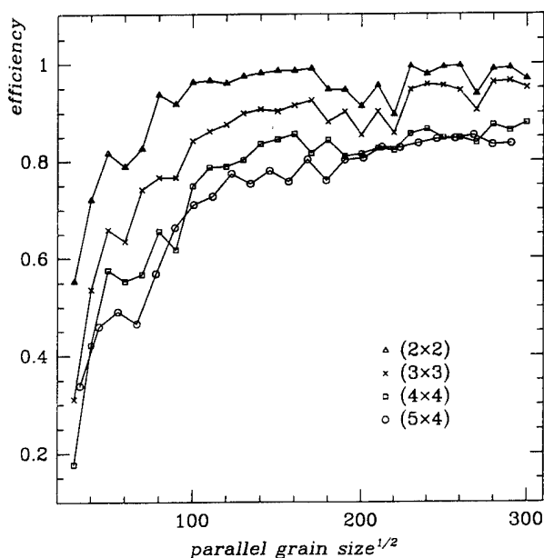
Figure 1: Parallel efficiency of 2D simulations.
