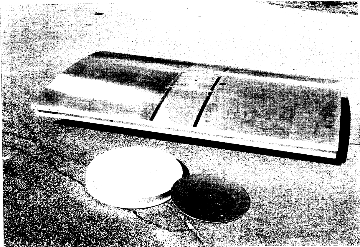
Figure 2. Ground Plane Structures Used: Mock Fuselage, Ground Plane, and Choke Ring.
