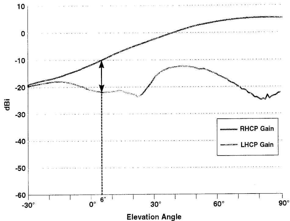
Figure 9. Smallest Minimum Cross Polarization Ratio Determined From Absolute Gain, NovAtel (corner fed patch) Antenna on a Choke Ring; Azimuth Angle = 135 degrees.
