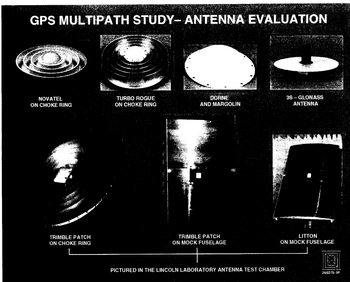
Figure 4. Antennas Tested.
