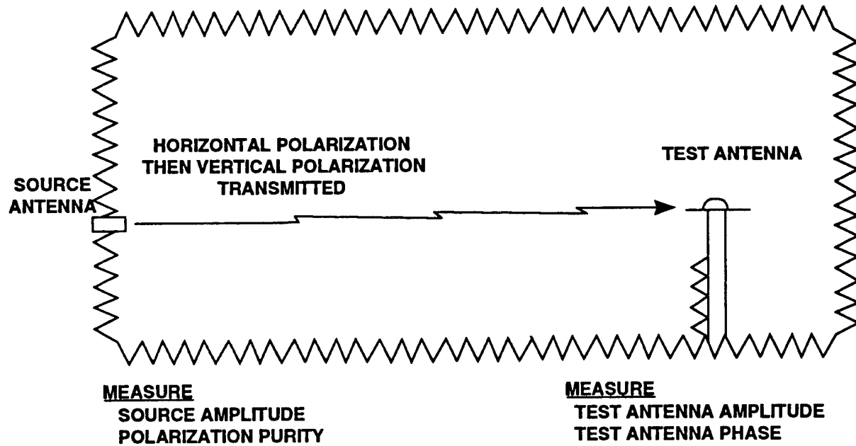
Figure 6. Sketch of Test Setup.
