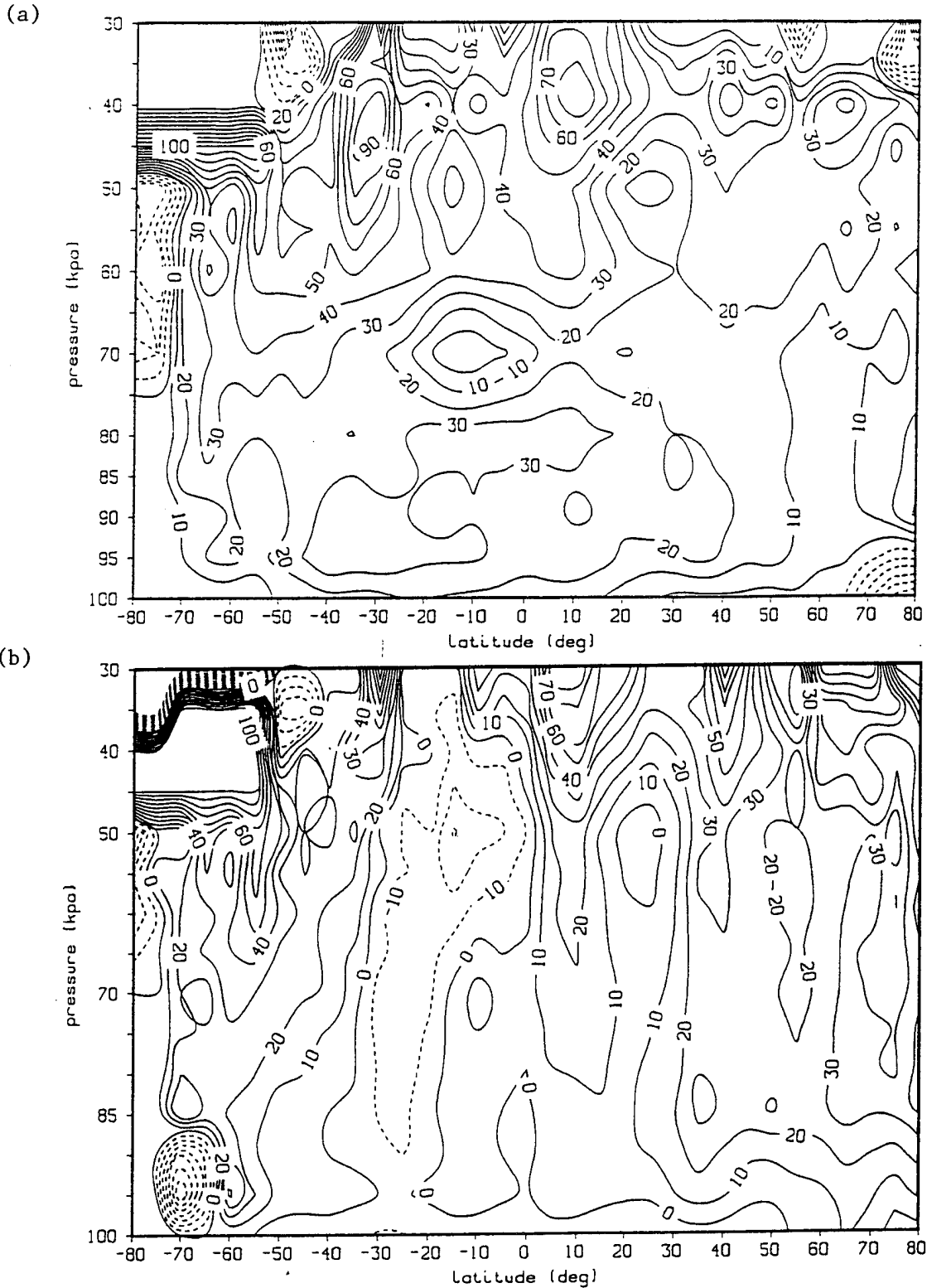
Figure 5. Zonal Cross Sections of Difference (in Percent) Between (a) June 1979 FGGE IIIb Analyses and a RAOB Climatology, and (b) July 1991 ECMWF Analyses and the RAOB Climatology.
