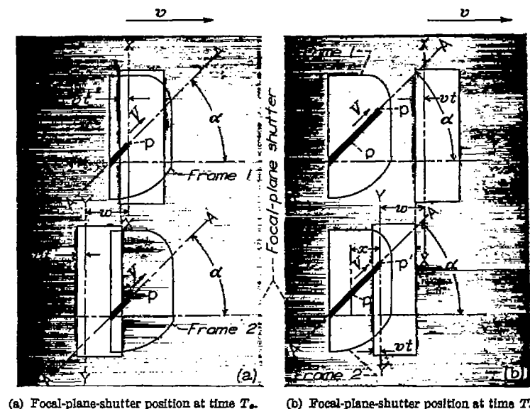
FIGURE 4.—Schematic diagrams of focal-plane-shutter action.
