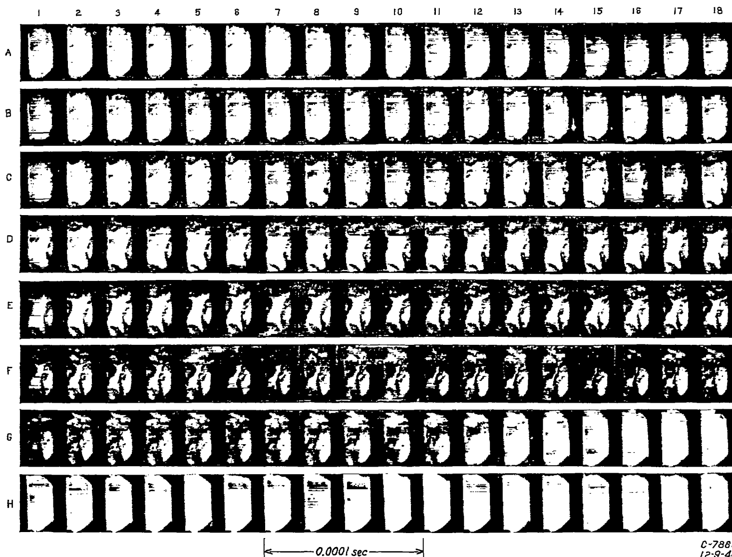
FIGURE 8.—High-speed motion pictures of knocking combustion cycle in engine cylinder showing detonation preceded by diffuse autoignition. M-2 fuel; four spark plugs. (Fig. 7 of reference 7.) (See fig. 9 for enlargement of knocking portion.)
