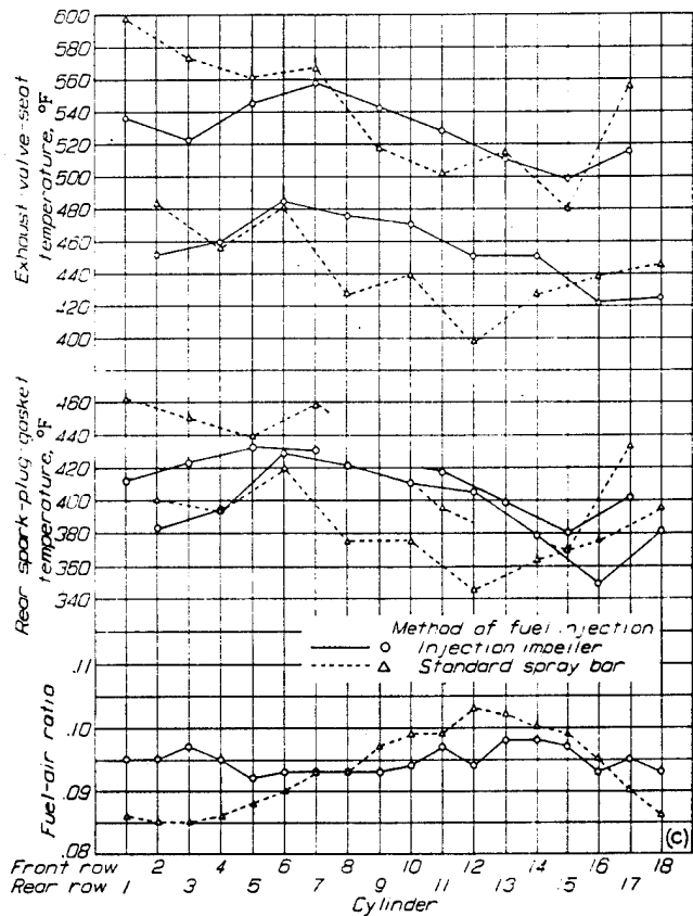
(c) Brake horsepower, 1700; engine speed, 1300 rpm.
