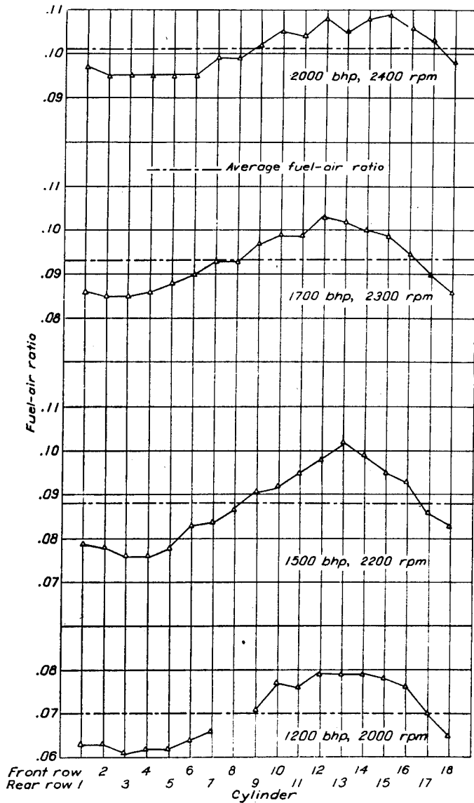
FIGURE 5.—Mixture distribution of engine using standard spray bar at various engine powers and speeds.
