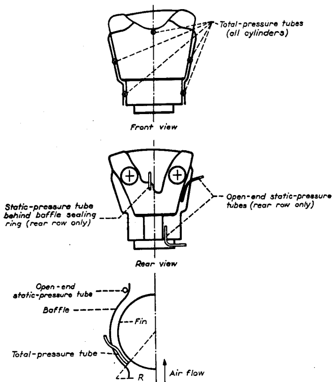
FIGURE 4.—Location of cooling-air pressure tubes.
