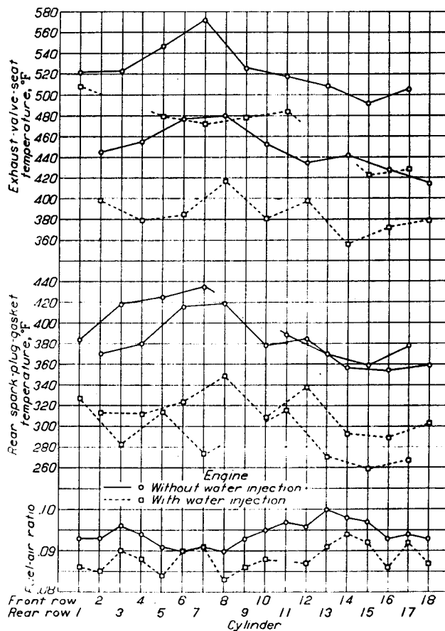
FIGURE 10.—Comparison of temperature distributions for engine modified by use of NACA injection impeller with and without water injection. Brake horsepower, 1700; engine speed, 2300 rpm; water-fuel ratio, 0.5.
