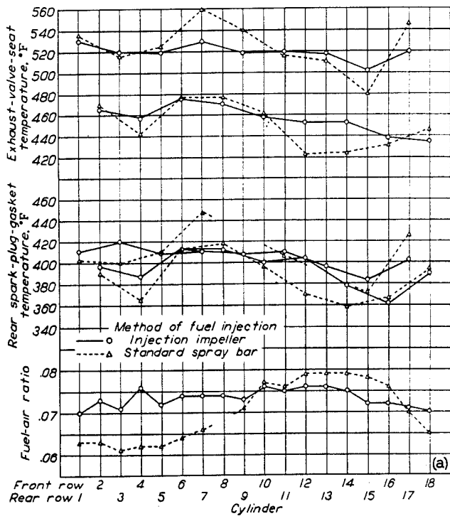
(a) Brake horsepower, 1200; engine speed, 2000 rpm.
