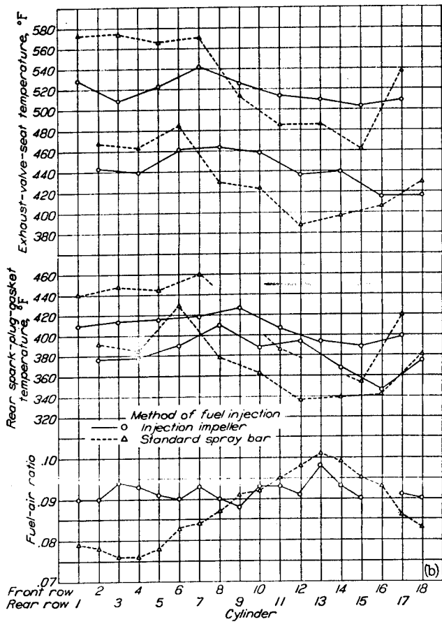
(b) Brake horsepower, 1500; engine speed, 2200 rpm.
