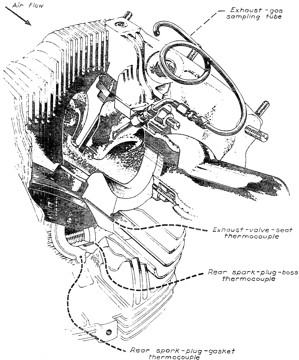
FIGURE 3. Location of thermocouples and exhaust-gas sampling tube.
