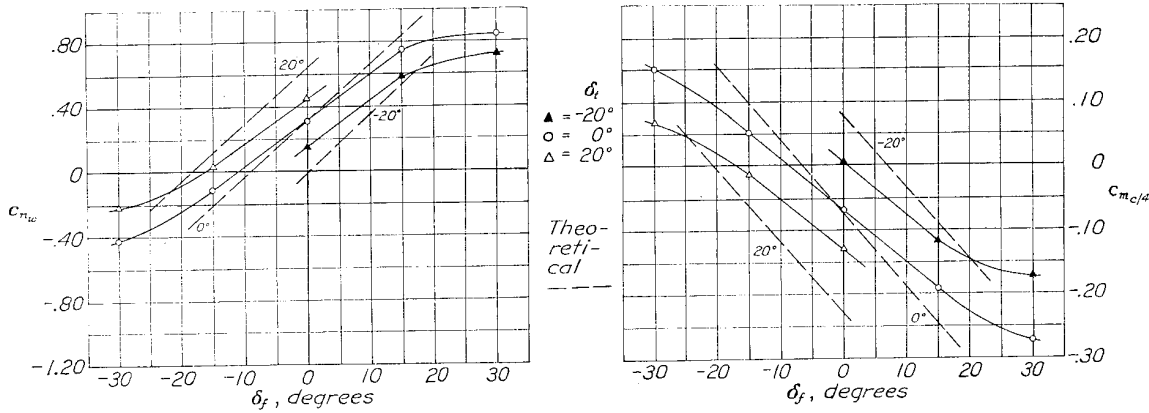
FIGURE 13.—Comparison of theoretical and experimental values of airfoil section normal-force and pitching-moment coefficients. Clark Y section with flap and tab. \alpha = 0^\circ
