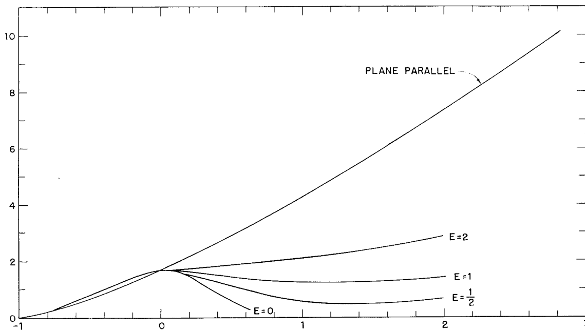
Figure 6a. v_m = 1/2 . For a beam whose minimum section is 1/3 the initial section. Ordinates: G(u) .
