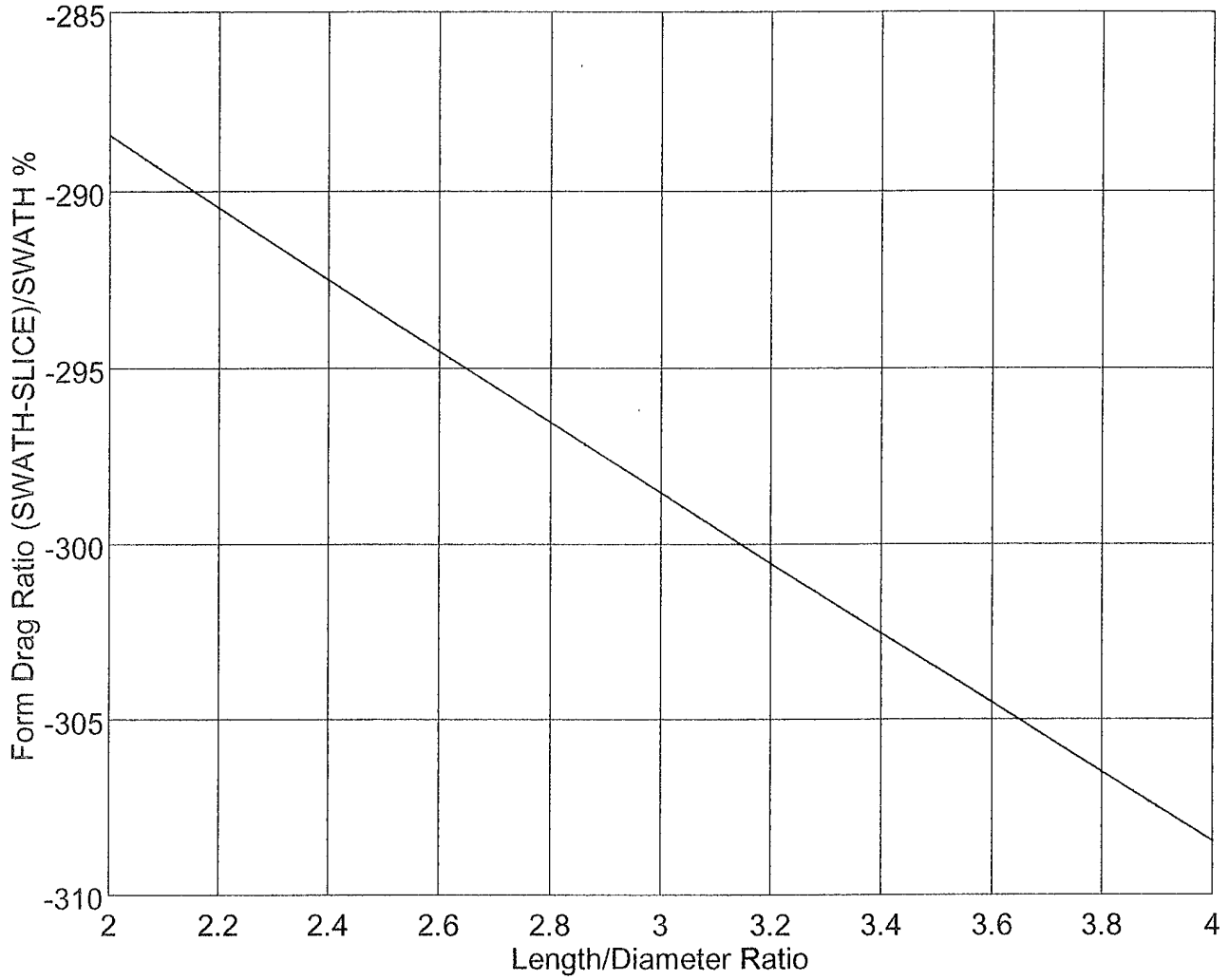
Figure 3.44: Form drag ratio vs. length to diameter ratio for limited diameter.
