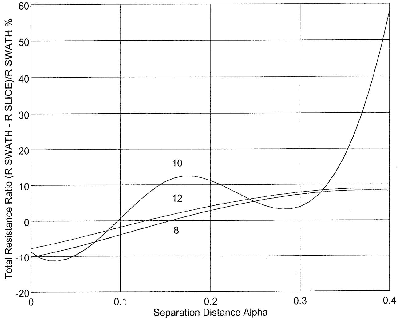
Figure 3.1: Total resistance ratio vs. separation distance alpha for limited length case for different displacement to length ratios.
