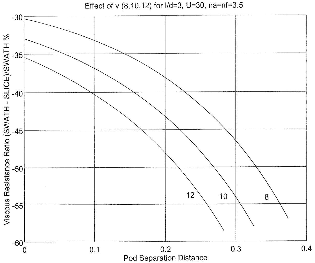
Figure 3.18: Viscous resistance ratio vs. pod separation distance for limited length case for different displacement to length ratios.
