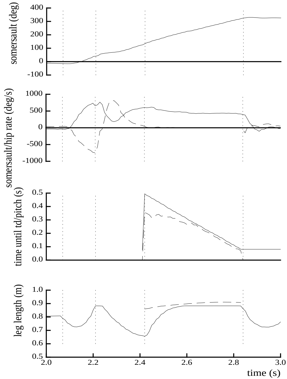
Figure 3-6: Somersault angle, absolute somersault rate (solid) and relative hip rate (dashed). The third graph shows the estimated time until touch down (solid) and estimated time until desired somersault attitude is achieved (dashed). The last graph is the measured leg length (solid) and desired leg length(dashed) for one leg. Vertical lines indicate initiation of flip, lift-off, tuck servo initiation, and landing. Data file B92.181.3.
