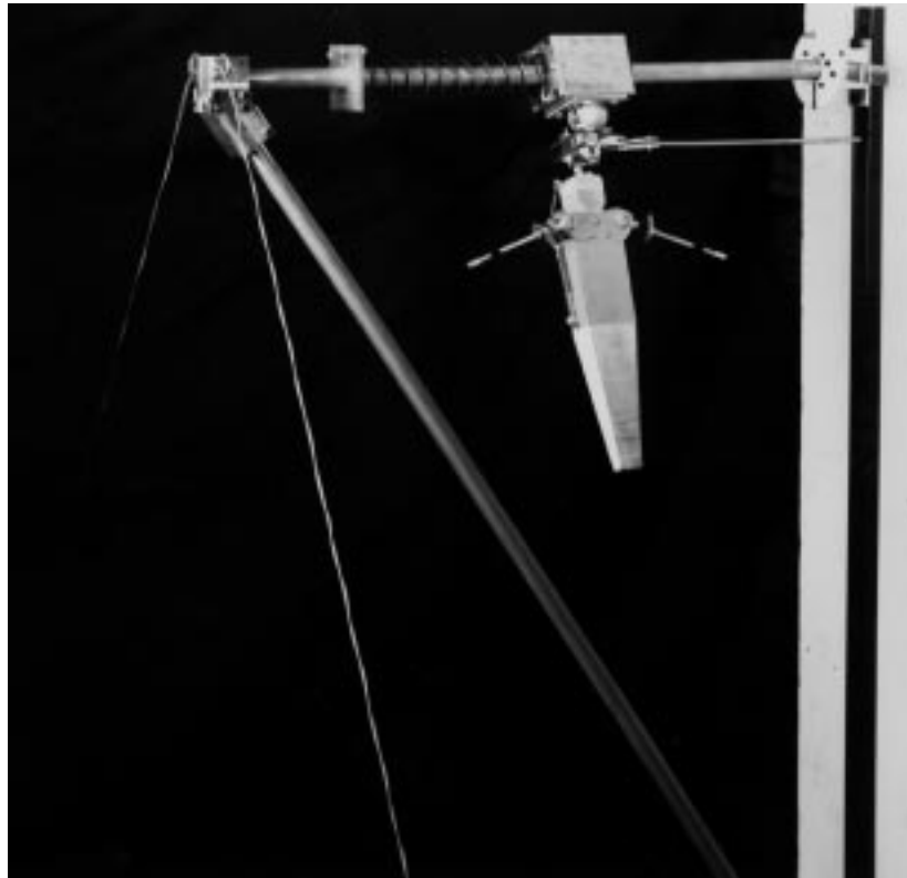
Figure 5-4: Photograph of the mechanical launcher used to initialize the doll somersaults in experiments.
