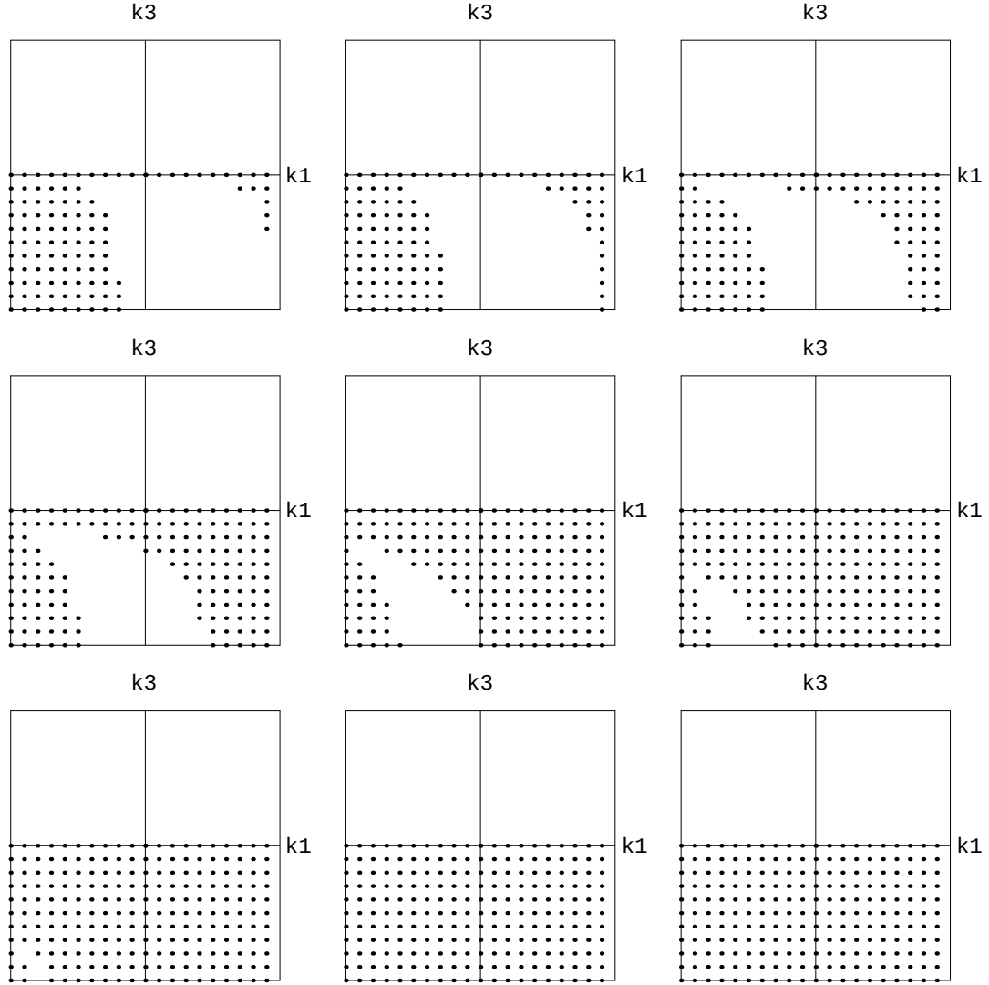
Figure 4-19: These plots show that stabilization gets easier with larger arms. Each dark point represents a stable configuration in k_1 - k_3 space for rotation about a principal axis. kl_1 = -1, K_{sh} = 1.0 . Each plot is for a different value of I_{rel} . I_{rel} = 0.01, 0.02, 0.05, 0.1, 0.2, 0.3, 0.4, 0.5 and 0.6 for plots positioned from left to right and down the page.
