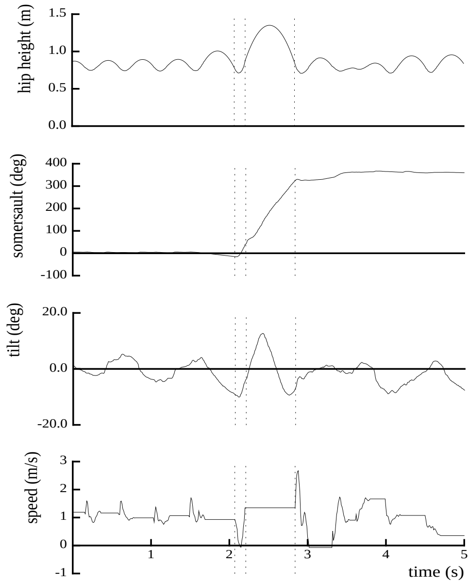
Figure 3-5: Hip height, somersault, and tilt angles, and forward speed of the 3D-Biped during a somersault. Vertical lines indicate initiation of flip, lift-off and landing. Data file B92.181.3
