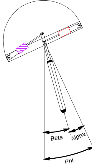
Figure 3-4: In order to maintain balance at landing the leg inclination angle, \beta , must be near the desired value. \beta is the angle the leg makes with the local vertical. It is a function of the the hip angle, \alpha and the body attitude, \Phi .
