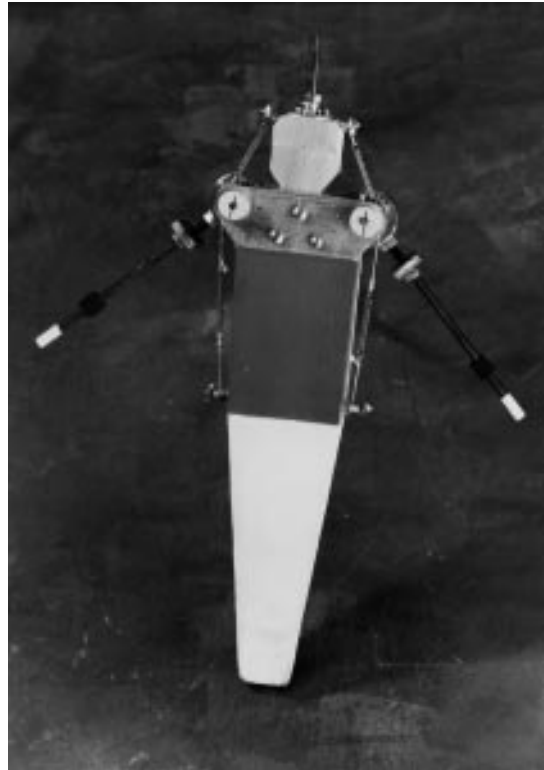
Figure 1-3: Photograph of the mechanical doll used for experiments with layout somersaults. The doll could consistently perform stable, triple layout somersaults.
