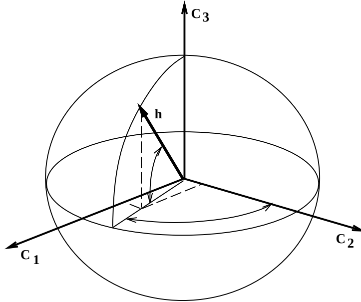
Figure 2-8: The spherical coordinates used to define orientation of the unit angular momentum vector in direction cosine space are the negative of the tilt and twist Euler angles.
