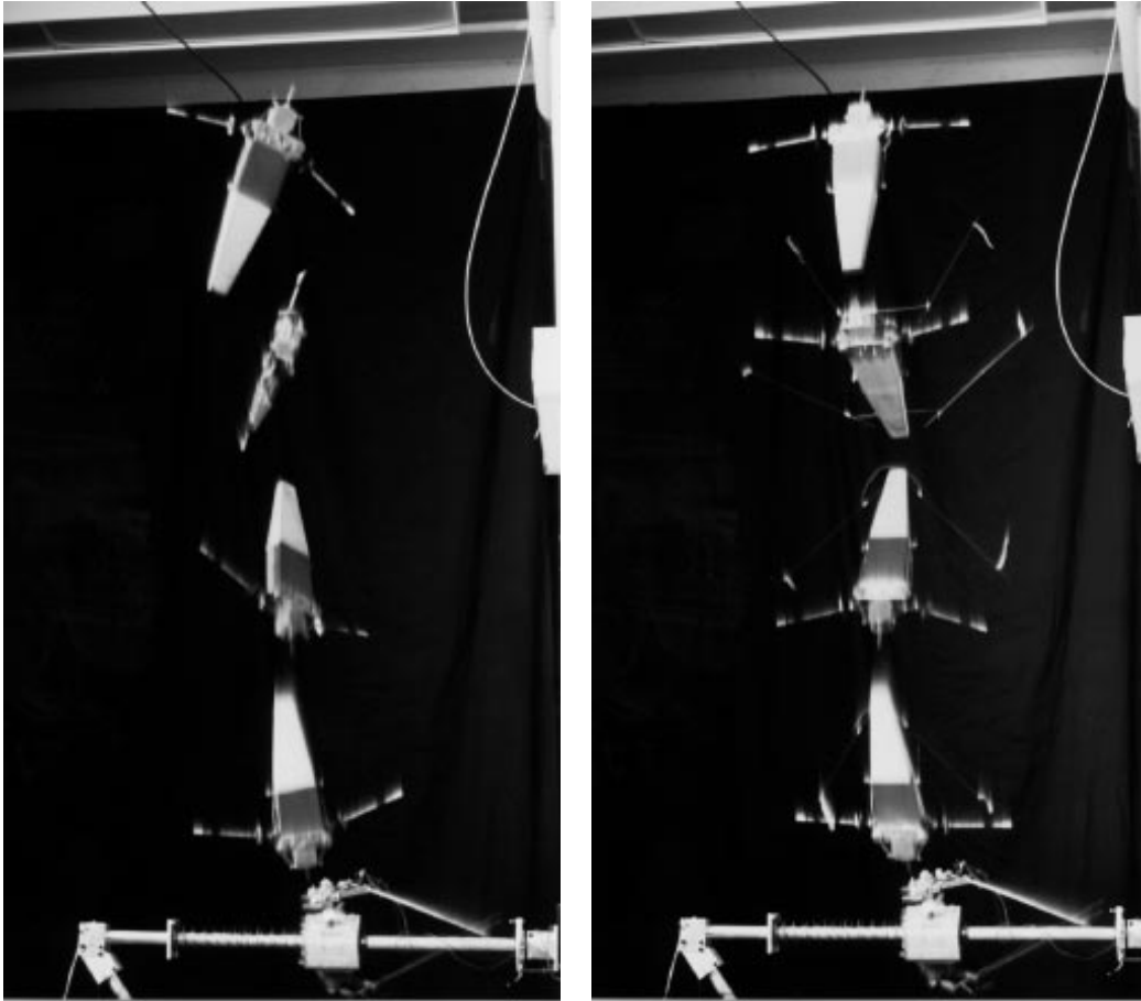
Figure 5-6: The photo on the left show the rigid doll with arms clamped in place. This doll exhibits the twist instability. The photo on the right shows the doll with flexible arms performing a stable layout somersault.
