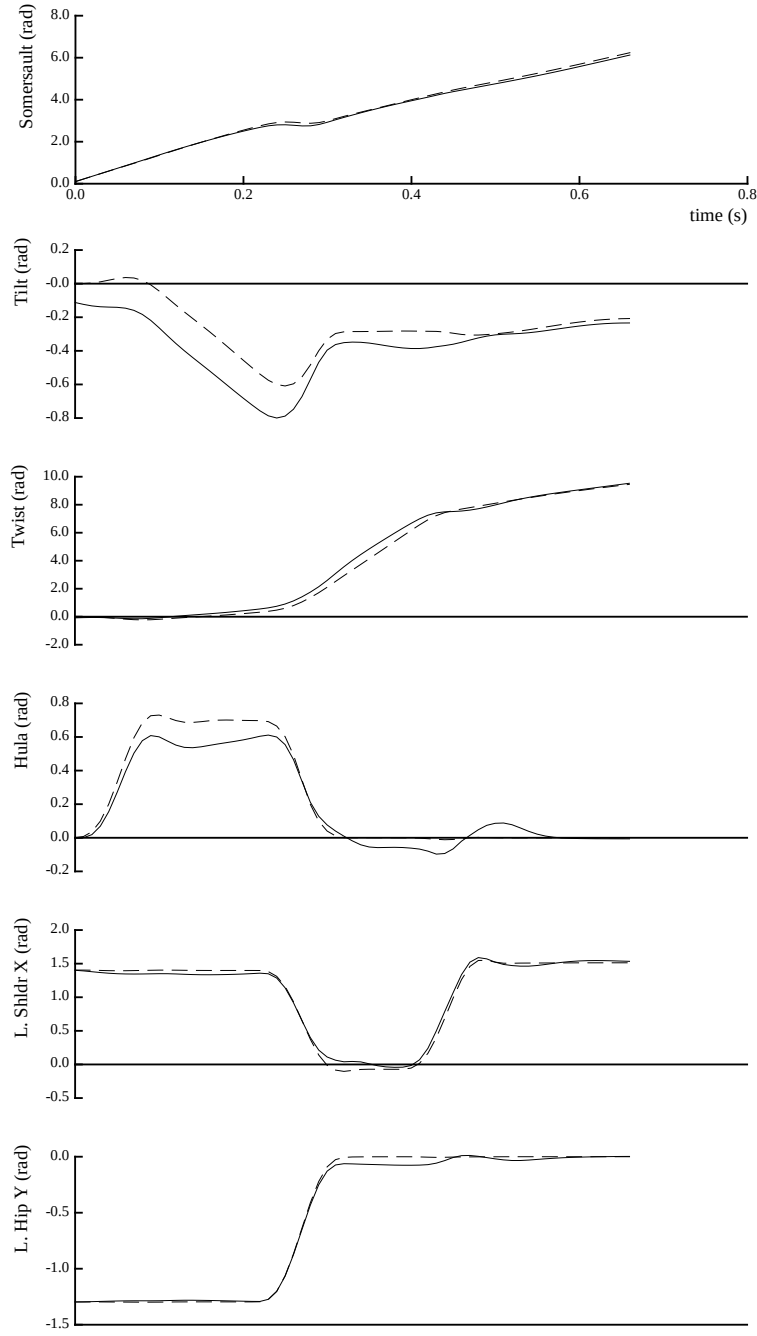
Figure 6-5: Simulation data from a 1 1/2 twisting somersault with \omega_n = 30 , \Theta_0 = -0.1 , and \Psi_0 = -0.1 are shown with solid lines. The desired values of the body attitude and joint angles are shown with dashed lines. Joint angles incur significant tracking errors but the landing attitude closely follows that of the nominal maneuver. (The traces stop at the landing time.)
