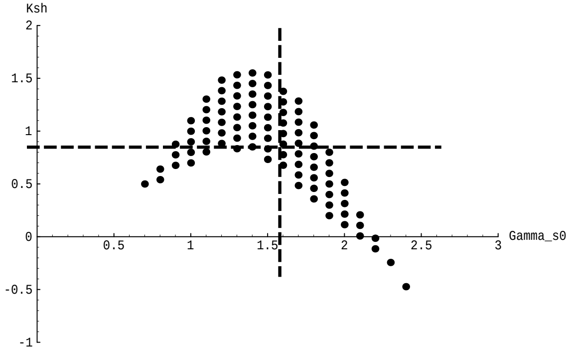
Figure 5-5: The points in this plot indicate the values of K_{sh} that theoretically will stabilize layout somersaults in the doll. The cross-hairs indicate the spring constant that best stabilized the doll during experiments.
