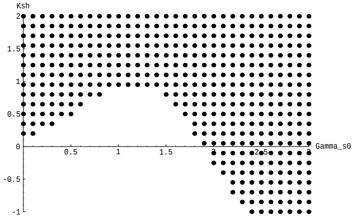
Figure 4-11: Each darkened point in this plot corresponds to a specific choice of K_{sh} and the nominal symmetric arm angle ( \Gamma_{s0} ) that stabilize the two d.o.f. linear system of somersault and symmetric arm movement, b_{sh}/\dot{\Phi} = 0 . Higher values of K_{sh} than are shown on this plot are suspected to also stabilize the system.
