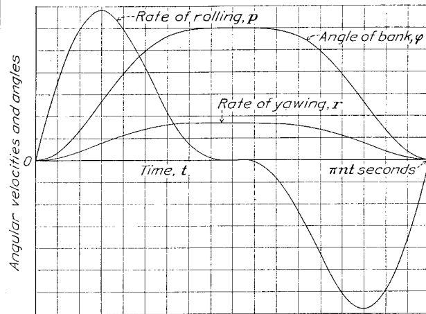
FIGURE 5.—Specifications for a turn maneuver in which the constraints are given by \varphi = \frac{1}{2}A_1 + A_1 \cos nt + \frac{1}{2}A_1 \cos 2nt ; p = \frac{d\varphi}{dt} ; r = \frac{g}{U_0} \varphi .
