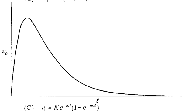
FIGURE 4.—Curves of different formulas for representing gusts.
