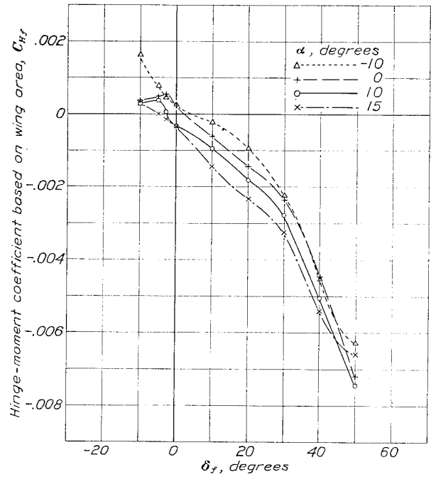
FIGURE 25.—Hinge-moment coefficients of flap. Hinge axis 2. N. A. C. A. 23012 airfoil with 0.20c r N. A. C. A. 23012 external-airfoil flap.
