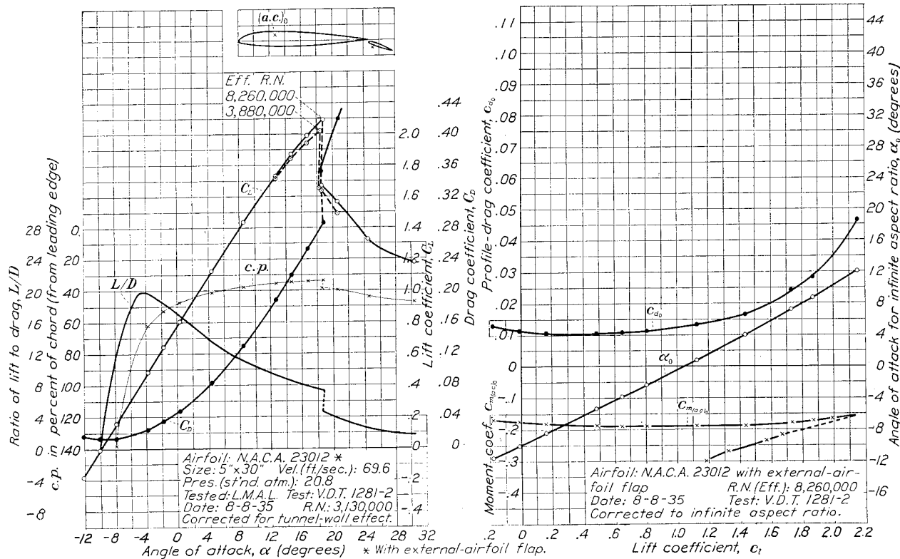
FIGURE 16.—The N. A. C. A. 23012 airfoil with 0.20c w N. A. C. A. 23012 external-airfoil flap. Flap angle, 20°. The airfoil is the same as used for variable-density tunnel test 1273 (fig. 14) except the flap setting. The value of c m(a,c) 0 is computed about the aerodynamic center as determined for test 1273.
