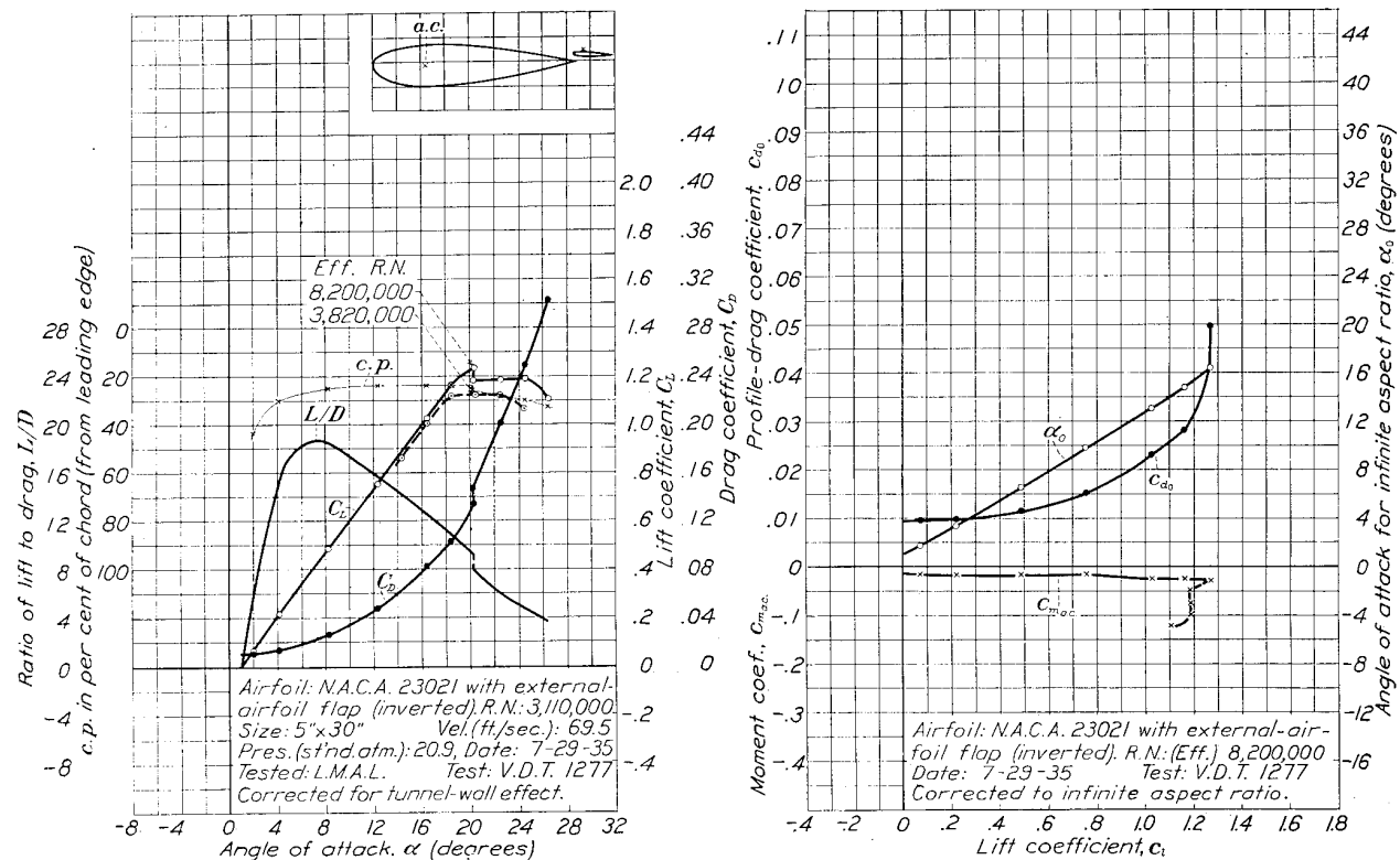
FIGURE 20.—The N. A. C. A. 23021 airfoil with 0.20c N. A. C. A. 23012 external-airfoil flap. Flap angle, -3° (inverted). The airfoil is the same as used for variable-density tunnel test 1274 (fig. 19) except inverted; a. c. from leading edge, 0.217c; a. c. above main wing chord, -0.01c.
