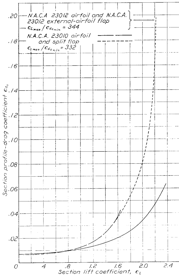
FIGURE 26.—Comparison of N. A. C. A. 23012 airfoil and 0.20c_w N. A. C. A. 23012 external-airfoil flap with N. A. C. A. 23010 airfoil and 0.20c_w split flap. Effective Reynolds Number, 8,200,000.
