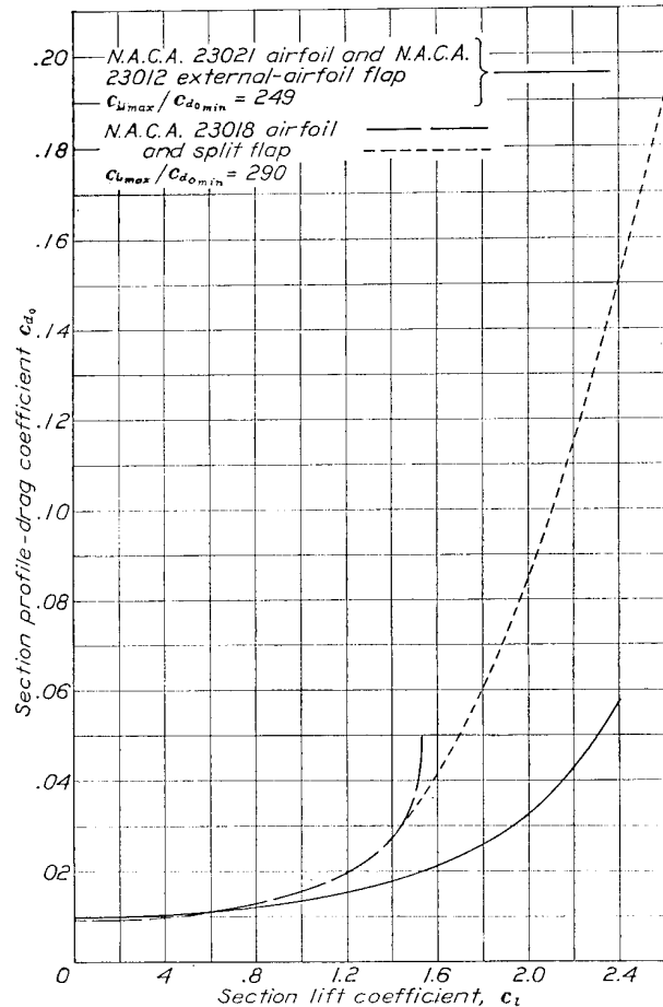
FIGURE 27.—Comparison of N. A. C. A. 23021 airfoil and 0.20c_w N. A. C. A. 23012 external-airfoil flap with N. A. C. A. 23018 airfoil and 0.20c_w split flap. Effective Reynolds Number, 8,200,000.
