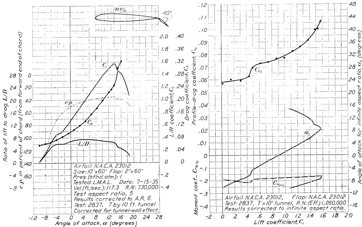
FIGURE 12.—The N. A. C. A. 23012 airfoil with 0.20c w N. A. C. A. 23012 external-airfoil flap. Flap angle, 40°. The airfoil is the same as used for test 2831-a (fig. 6) except the flap setting. The value of C m(a,c) 0 is computed about the aerodynamic center used for test 2831-a.
