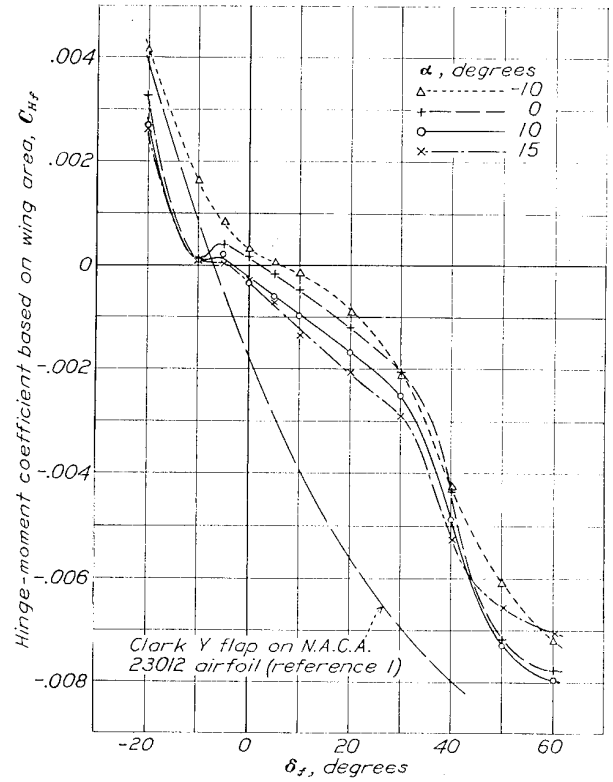
FIGURE 24.—Hinge-moment coefficients of flap. Hinge axis 1. N. A. C. A. 23012 airfoil with 0.20c r N. A. C. A. 23012 external-airfoil flap.
