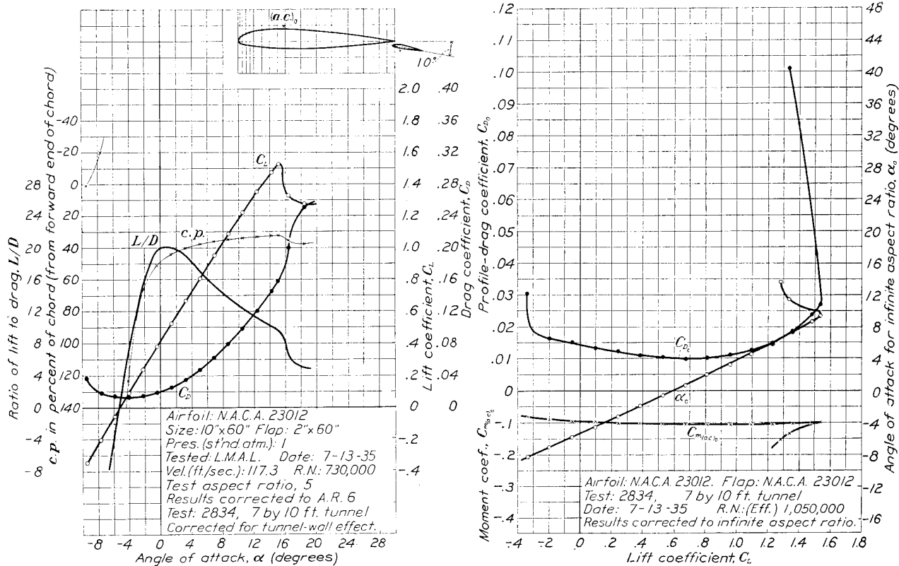
FIGURE 9.—The N. A. C. A. 23012 airfoil with 0.20c w N. A. C. A. 23012 external-airfoil flap. Flap angle, 10°. The airfoil is the same as used for test 2831-a (fig. 6), except the flap setting. The value of C_{m(a,c)_0} is computed about the aerodynamic center used for test 2831-a.
