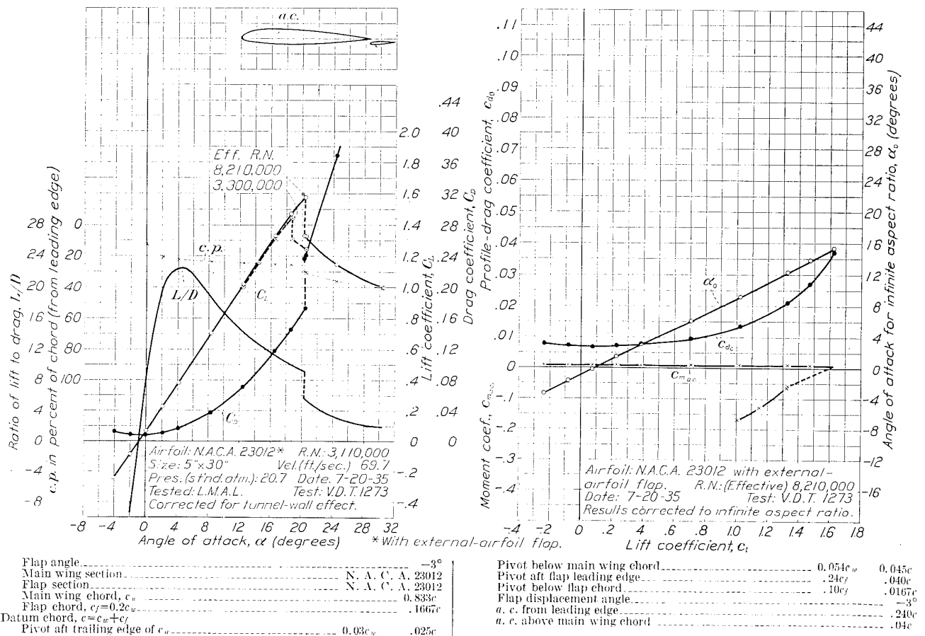
FIGURE 14.—The N. A. C. A. 23012 airfoil with 0.20c w N. A. C. A. 23012 external-airfoil flap.
