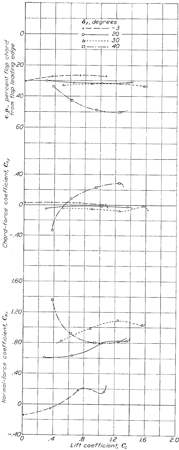
FIGURE 23.—Variation of air loads on flap with wing lift coefficient. N. A. C. A. 23012 airfoil with 0.20c r N. A. C. A. 23012 external-airfoil flap.
