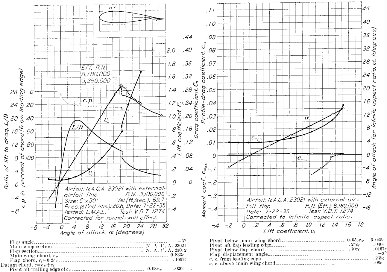
FIGURE 19.—The N. A. C. A. 23021 airfoil until 0.20c N. A. C. A. 23012 external-airfoil flap.
