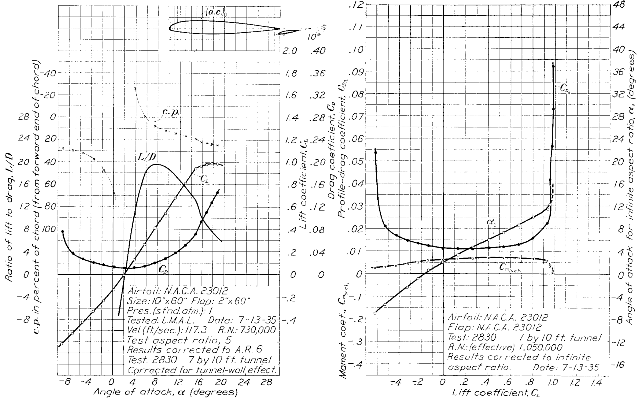
FIGURE 5.—The N. A. C. A. 23012 airfoil with 0.20c N. A. C. A. 23012 external-airfoil flap. Flap angle, -10^\circ . The airfoil is the same as used for test 2831-a (fig. 6), except the flap setting. The value of C_{m(a.c.)_0} is computed about the aerodynamic center used for test 2831-a.
