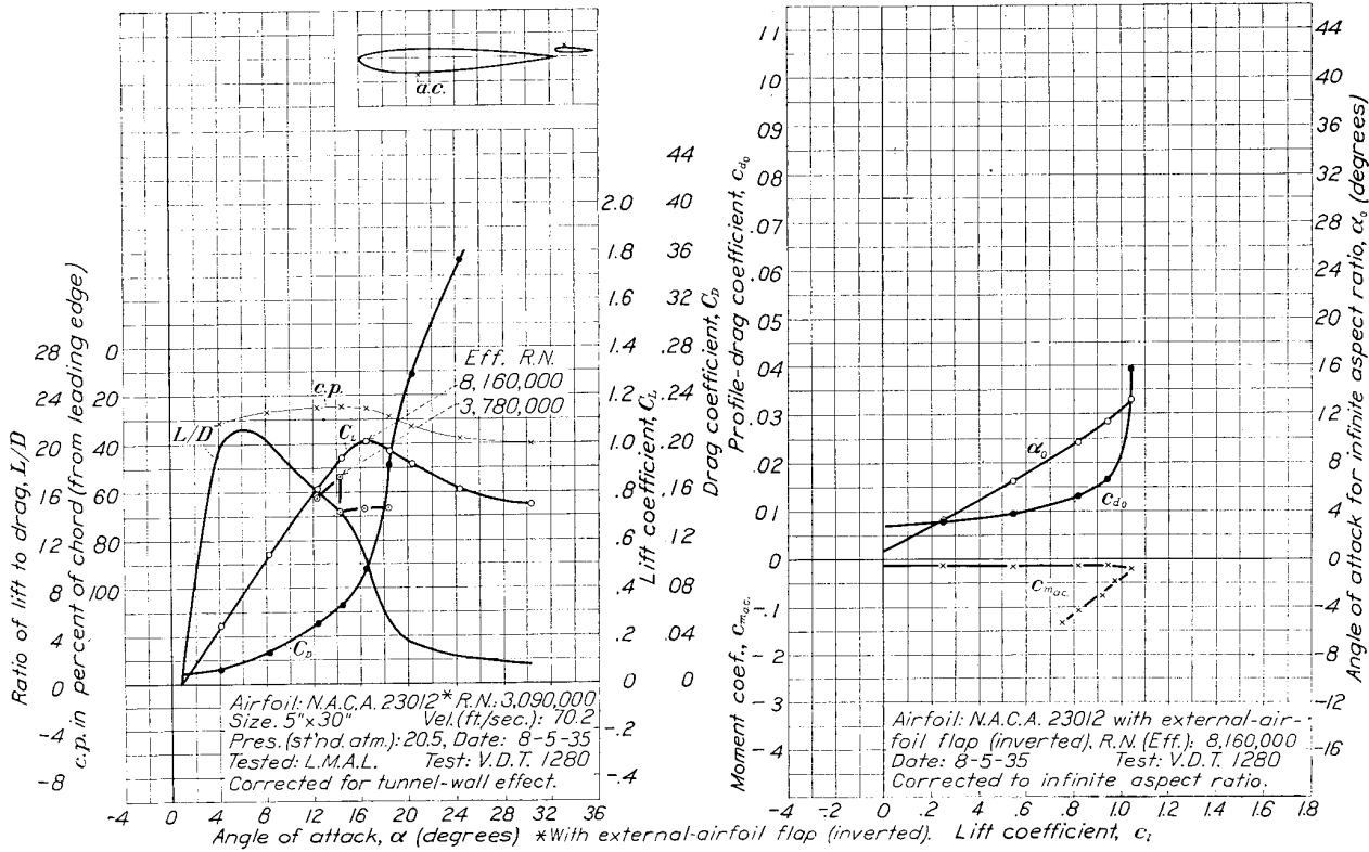
FIGURE 15.—The N. A. C. A. 23012 airfoil with 0.20c w N. A. C. A. 23012 external-airfoil flap. Flap angle, -3° (inverted). The airfoil is the same as used for variable-density tunnel test 1273 (fig. 14) except inverted; a. c. from leading edge, 0.252c; a. c. above main wing chord, -0.07c.
