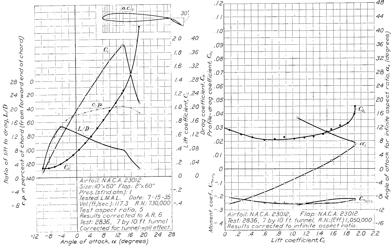
FIGURE 11.—The N. A. C. A. 23012 airfoil with 0.20c w N. A. C. A. 23012 external-airfoil flap. Flap angle, 30°. The airfoil is the same as used for test 2831-a (fig. 6) except the flap setting. The value of C m(a,c) 0 is computed about the aerodynamic center used for test 2831-a.
