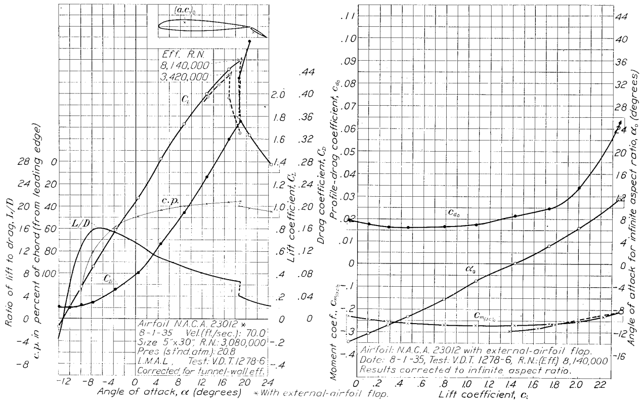
FIGURE 17.—The N. A. C. A. 23012 airfoil with 0.20c w N. A. C. A. 23012 external-airfoil flap. Flap angle, 30°. The airfoil is the same as used for variable-density tunnel test 1273 (fig. 14) except the flap setting. The value of c_{m(a,c)_0} is computed about the aerodynamic center as determined for test 1273.
