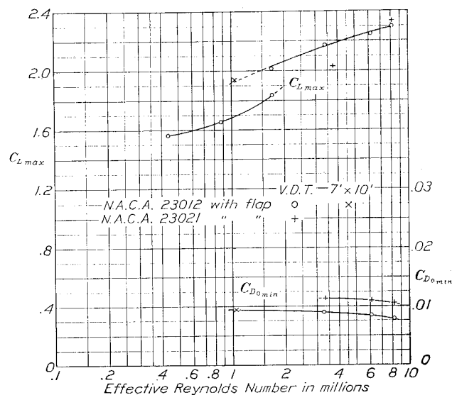
FIGURE 22. Scale effect on N. A. C. A. 23012 and N. A. C. A. 23021 airfoils with 0.20c_w N. A. C. A. 23012 external-airfoil flap. All values uncorrected for hinge fares and for effects of rectangular tips.
