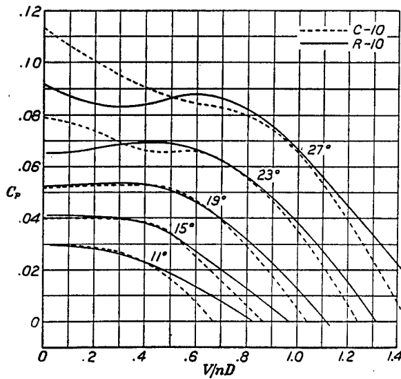
FIGURE 15b.—Power coefficients
