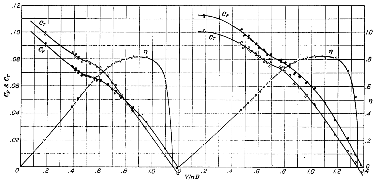
FIGURE 8.—Characteristics of propeller C-6; 23° at 42"
