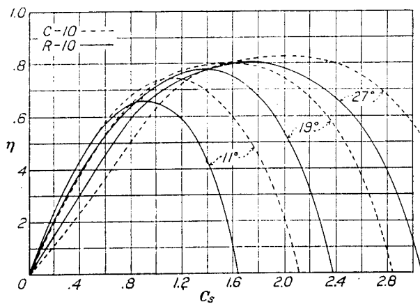
FIGURE 12.—Efficiency vs. speed power coefficient
