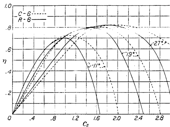
FIGURE 10.—Efficiency vs. speed power coefficient
