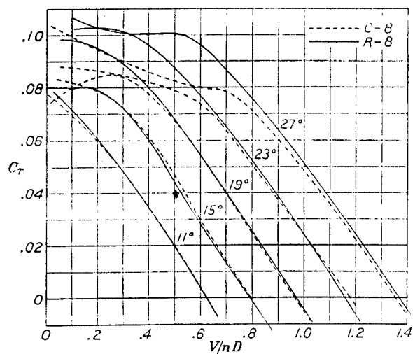
FIGURE 14a.—Thrust coefficients
