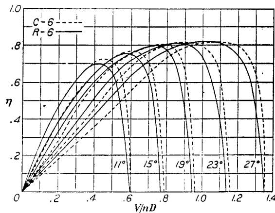
FIGURE 13c.—Efficiency
