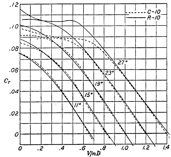
FIGURE 15a.—Thrust coefficients
