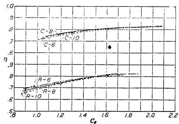
FIGURE 17.—Maximum efficiency vs. speed power coefficients
