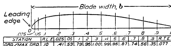
Standard propeller section based on R.A.F.-6
