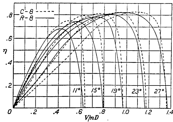
FIGURE 14c.—Efficiency
