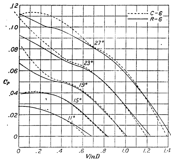
FIGURE 13b.—Power coefficients
