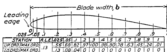
Propeller section based on Clark-Y
