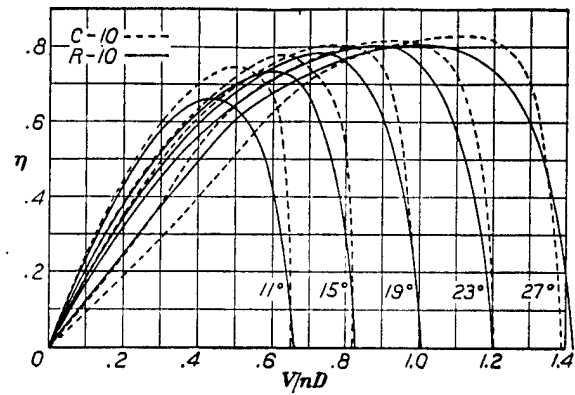
FIGURE 15c.—Efficiency
