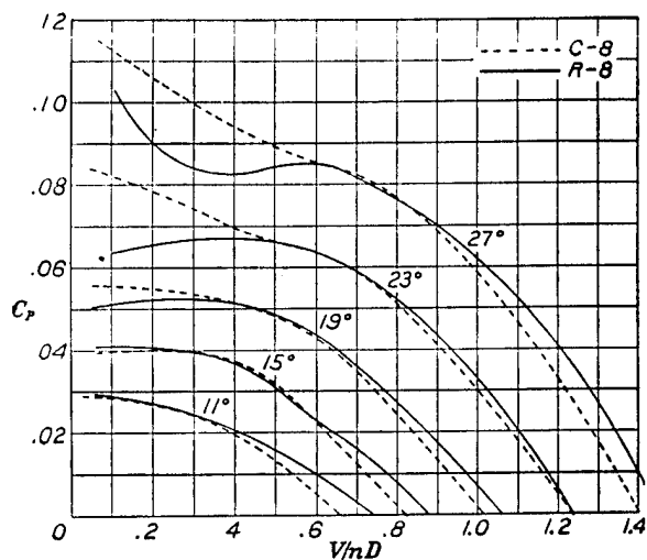
FIGURE 14b.—Power coefficients
