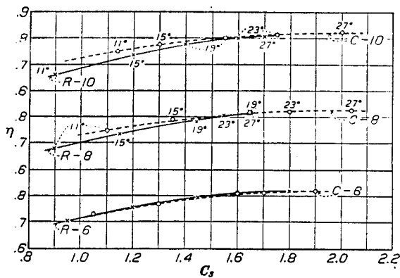
FIGURE 16.—Maximum efficiency vs. speed power coefficients
