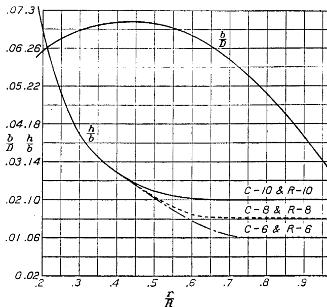
FIGURE 3.—Blade form curves; b =blade width, D =propeller diameter, h =maximum blade thickness, r =section radius, R =propeller radius
