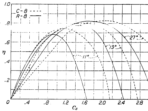
FIGURE 11.—Efficiency vs. speed power coefficient
