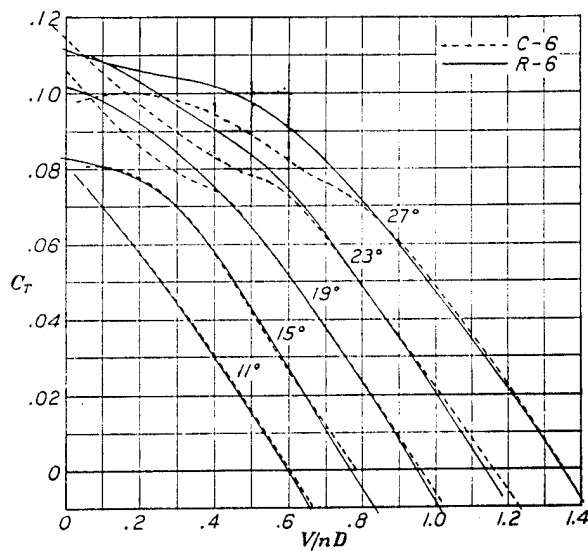
FIGURE 13a.—Thrust coefficients
