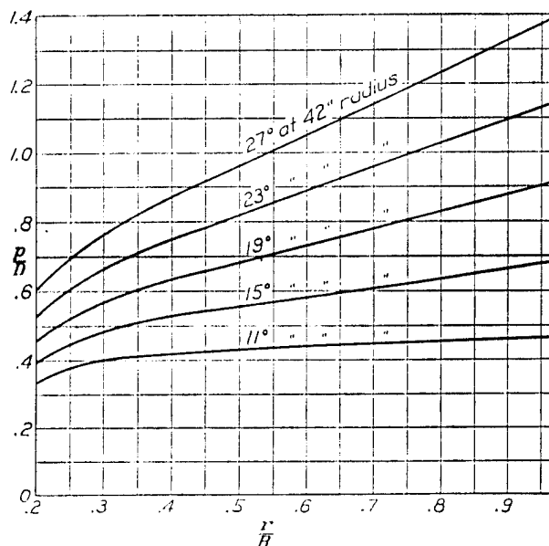
FIGURE 4.—Pitch distribution
