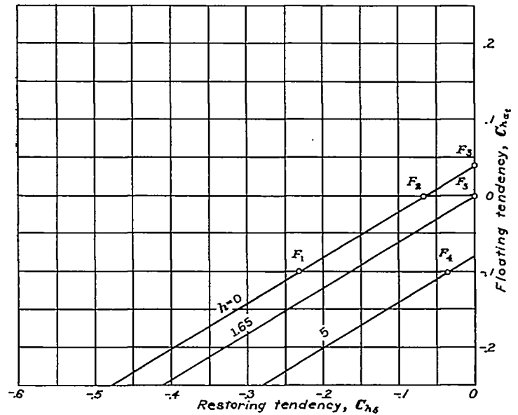
FIGURE 2.—Lines of constant stick-force gradient showing combinations of hinge-moment parameters used. F_n=5 pounds per g ; x_{a.c.}=0.075c .
