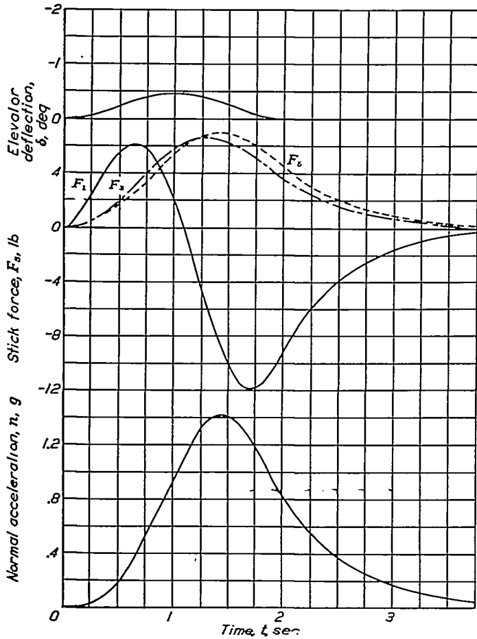
FIGURE 8.—Stick force and normal acceleration due to rapid elevator motion. T=2 seconds; V=400 miles per hour; x_{e.a.}=0.01c .
