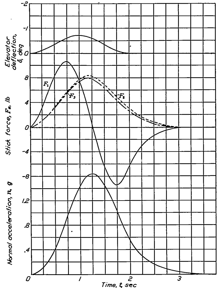
FIGURE 7.—Stick force and normal acceleration due to rapid elevator motion. T=2 seconds; V=400 miles per hour; x_{a.a.}=0.042c .
