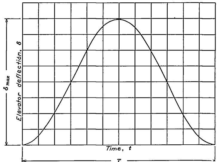
FIGURE 1.—Shape of curve of elevator deflection against time assumed in the analysis.
