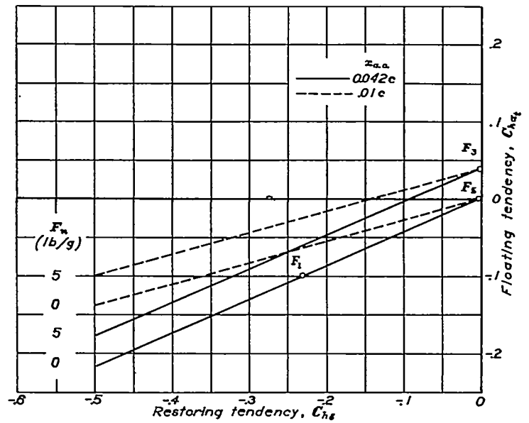
FIGURE 6.—Lines of constant stick-force gradient. F_m=0 and 5 pounds per g .
