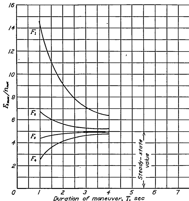
FIGURE 10.—Maximum stick force per unit maximum acceleration against duration of maneuver. x_{a.s.} = 0.075c .
