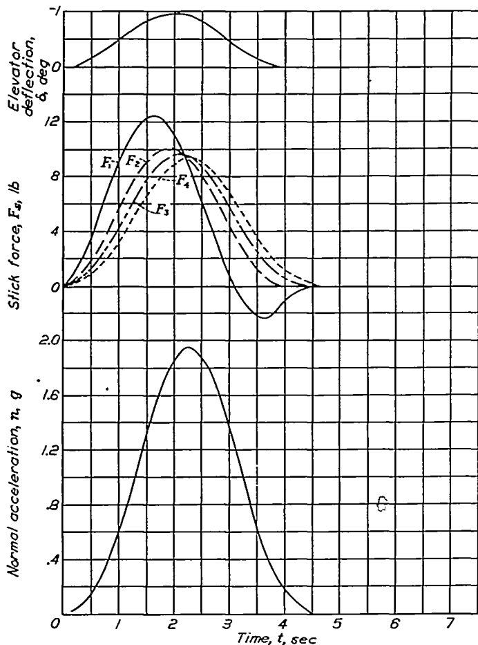
FIGURE 3.—Stick force and normal acceleration due to rapid elevator motion. T=4 seconds V=400 miles per hour; x_{c.g.}=0.075c .
