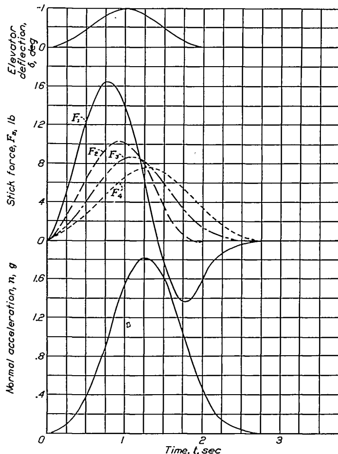
FIGURE 4.—Stick force and normal acceleration due to rapid elevator motion. T=2 seconds; V=400 miles per hour; x_{c.g.}=0.075c .
