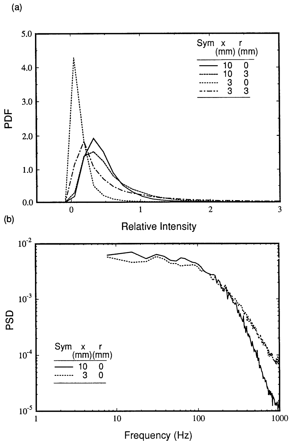
Figure 2. (a) PDF of LIF intensity for various locations in the flame. Each PDF is obtained from 25000 points sampled at 2 kHz. The average beam power used was 1 mW. (b) Normalized PSD of LIF intensity for two axial locations in the flame. Each PSD is obtained from 25000 points sampled at 2 kHz. The PSD is normalized by the mean-square of the LIF intensity fluctuations.
