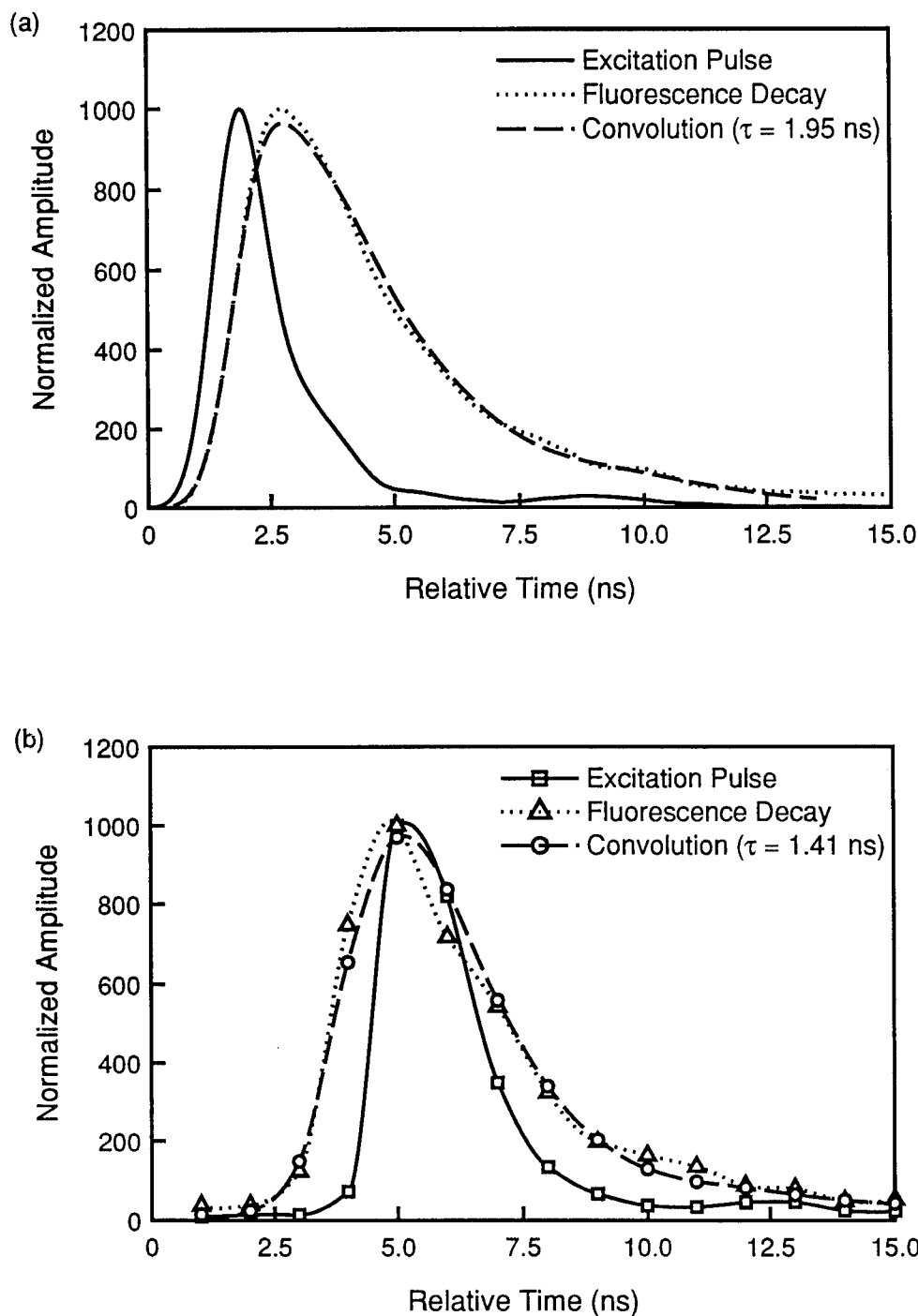
Figure 6. (a) Normalized equivalent-time instrument response and fluorescence decay obtained 5 mm above the center of the Hencken burner at \phi=1.0 . Both of these waveforms were obtained by averaging 500 individual waveforms and smoothing via a digital n-pole Bessel filter with a 900 ps risetime. (b) Similar normalized real-time waveforms obtained 5 mm over the McKenna burner at \phi=1.0 . The convolution of the excitation pulse with the exponential function determined from the convolute-and-compare algorithm is also displayed in both figures.
