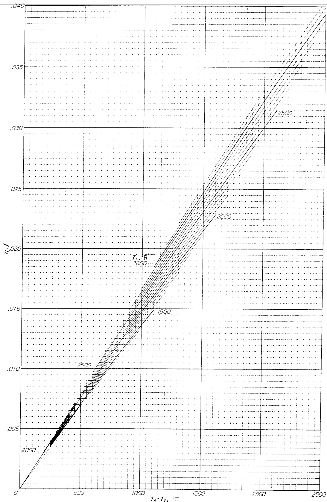
FIGURE 7. - Chart for determining fuel-air ratio for various values of rise in total temperature through combustion chamber and values of combustion-chamber-outlet total temperature. ( k , 18,500 Btu/lb)
