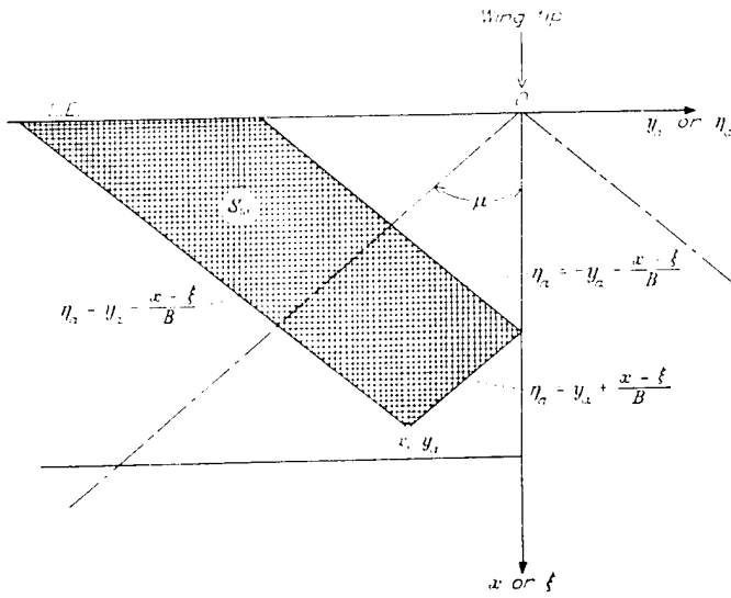
FIGURE 3. Region of integration for obtaining supersonic velocity-potential function for rectangular wing of finite wing span. Region of integration for point (x, y_a) shown cross-hatched; y_a = y - h on right half-wing; y_a = -y - h on left half-wing.
