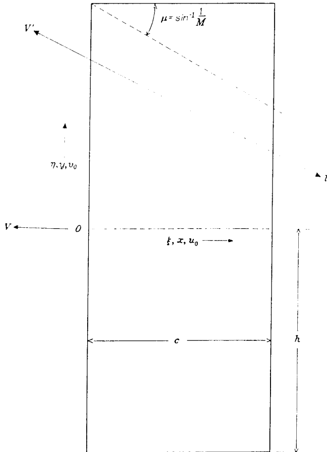
FIGURE 1. Axes and notation used in analysis.
