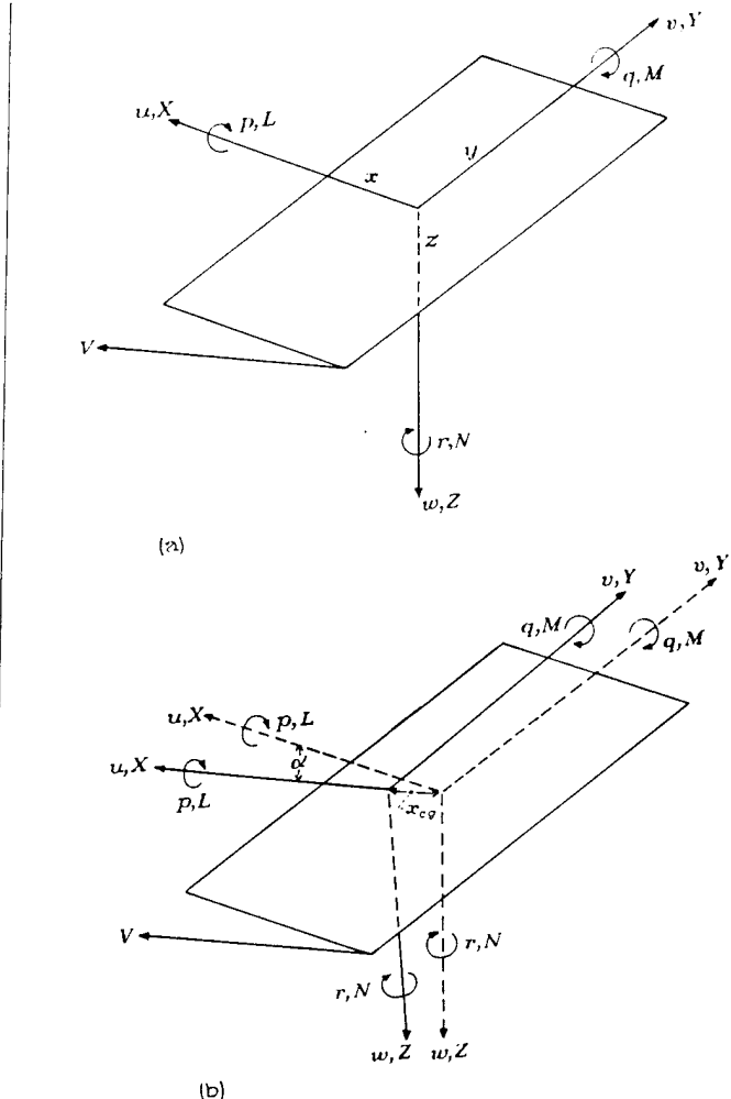
(a) Principal body axes. Origin at center of wing. (b) Stability axes. Origin at point (\frac{c}{2} - l, 0, 0) . Principal body axes dotted for comparison.
