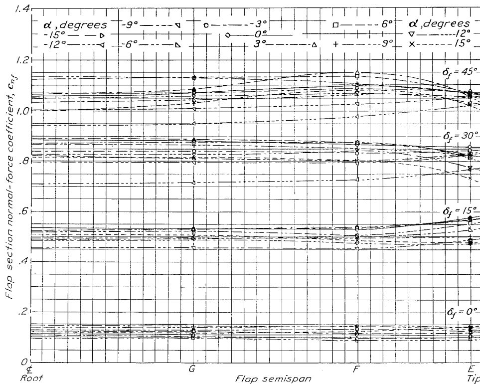
FIGURE 14.—Span load distribution on flap for various flap deflections.
