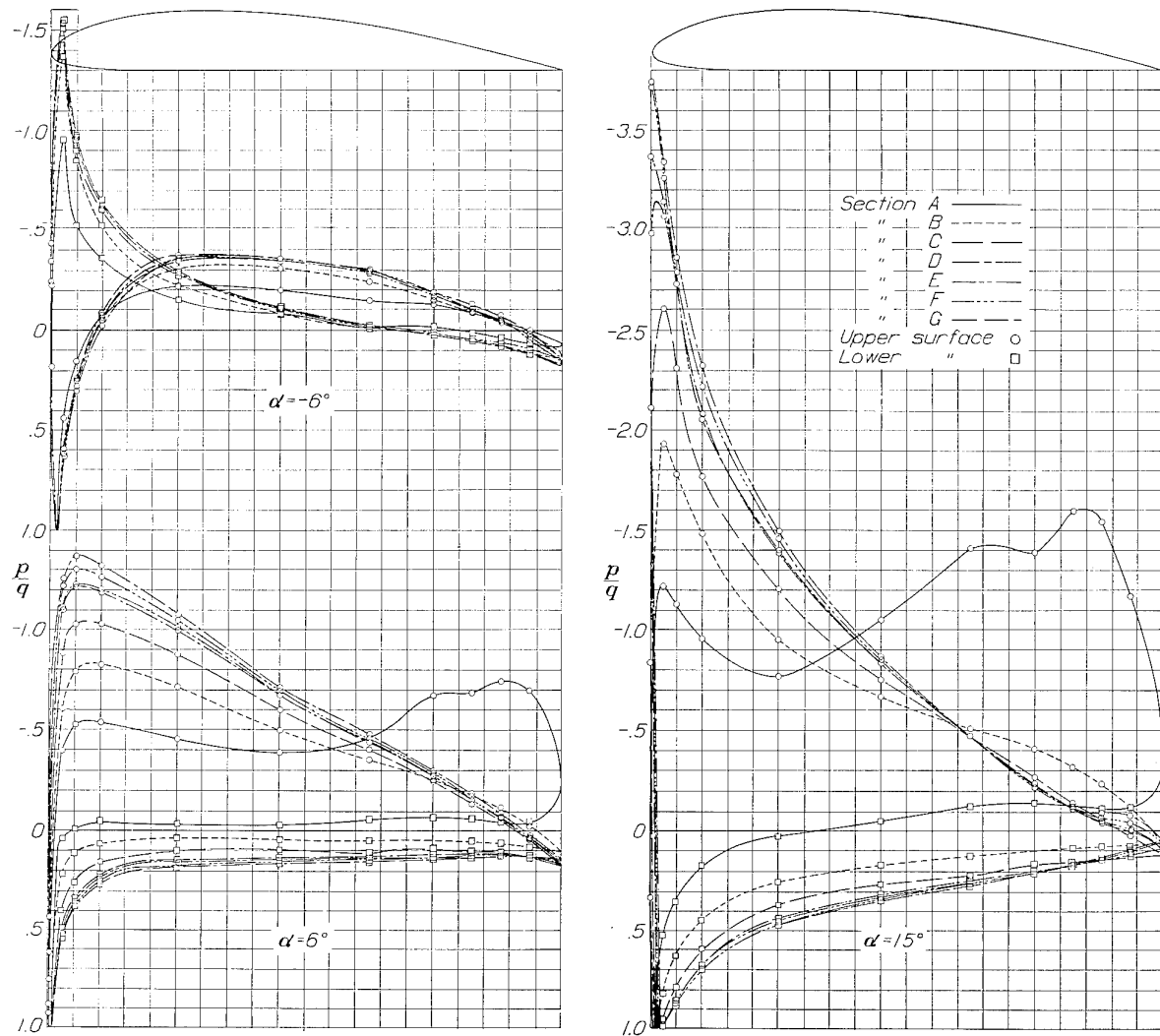
FIGURE 4.—Pressure distribution over airfoil sections at three angles of attack; \delta_1 = 0^\circ .
