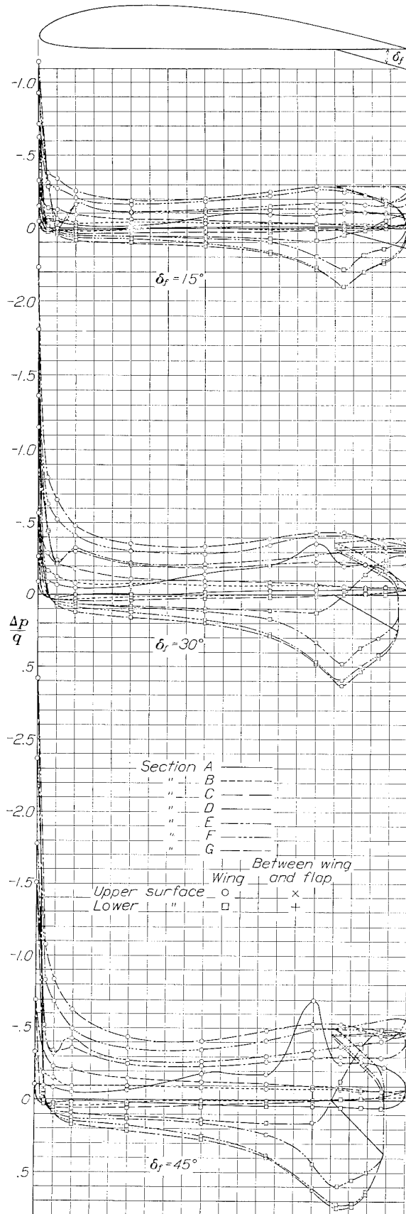
FIGURE 7.—Increments of pressure over airfoil sections at 15^\circ angle of attack with the flap deflected various amounts.
