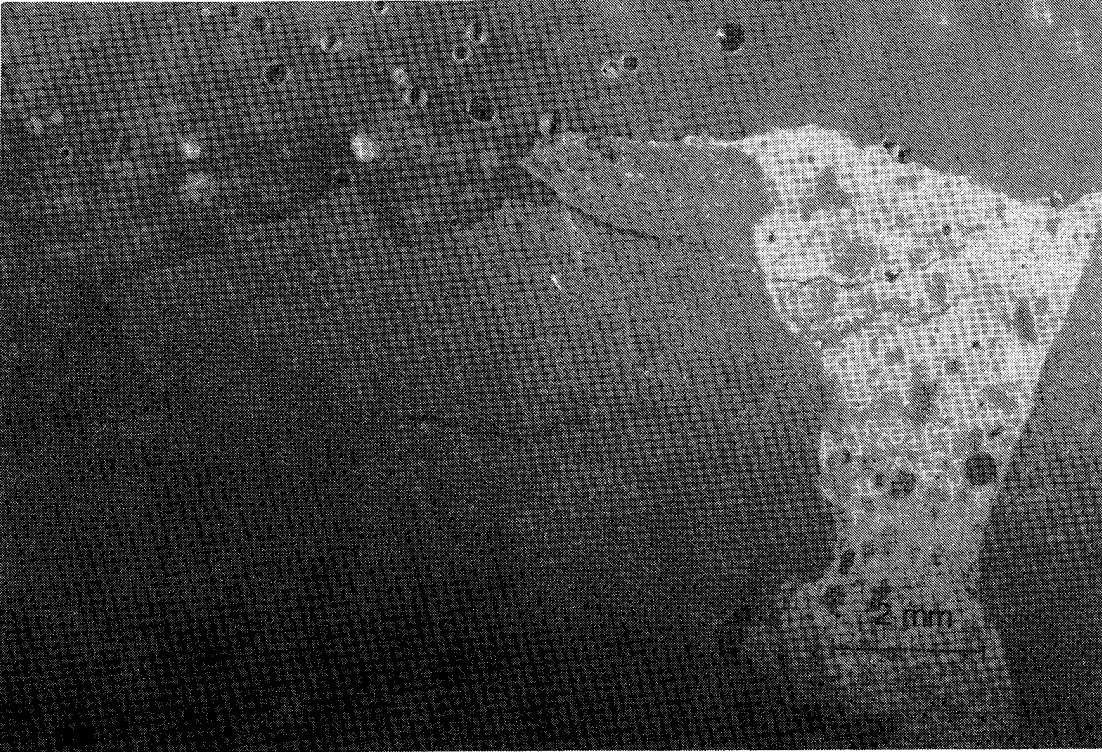
Figure C4. Specimen 940008. Cross-sectional view of surface concrete showing interlocking fractured pieces of aggregate and pieces of paste that may easily be dislodged mechanically. 10X
