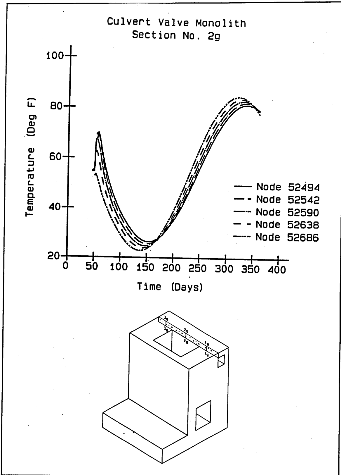
Figure 18. Temperature time-history at section 2g
