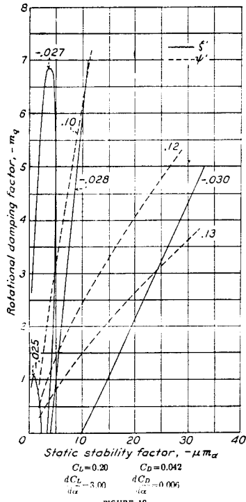
FIGURES 15 TO 20.—Dynamic stability charts.
