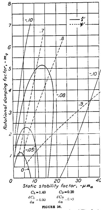
FIGURES 33 TO 38.—Dynamic stability charts.
