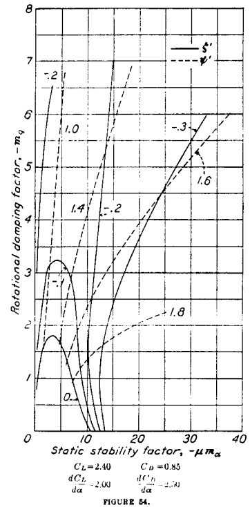
FIGURES 51 to 54.—Dynamic stability charts.
