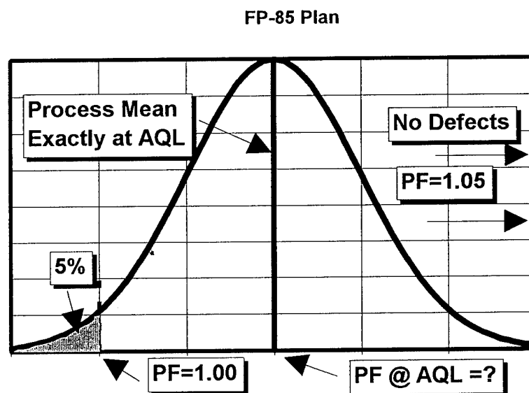
Figure 4-1 Graphical Representation of 5% Risk of Pay Factor < 1.00
