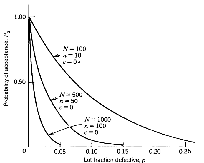
Figure 2-5 Sample as a Percentage of Lot Size [Montgomery, 1991, p 564]
