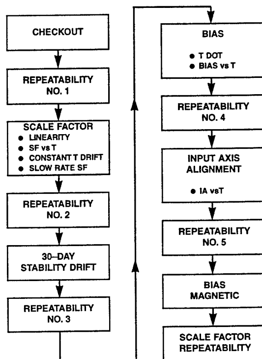
Figure 5. Demonstration Unit Test Sequence
