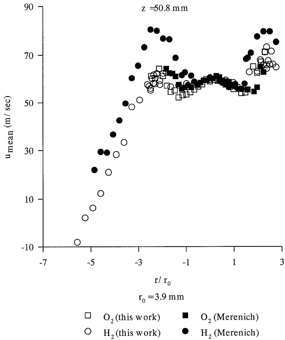
Fig. 19: Hot-Fire Measurements of Mean Velocity at 50.8 mm (2 in.) Axial Location
