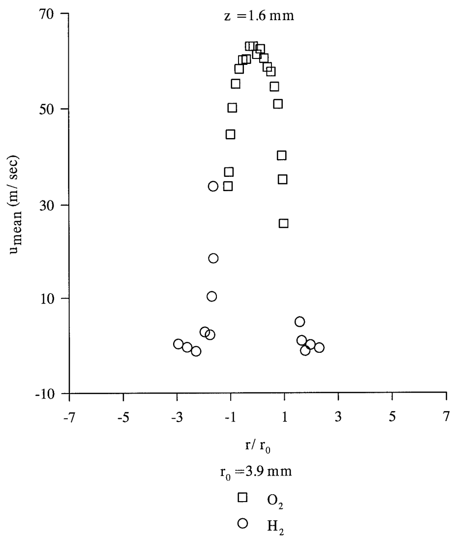
Fig. 28: Hot-Fire Measurements of Mean Velocity at 1.6 mm (0.063 in.) Axial Location
