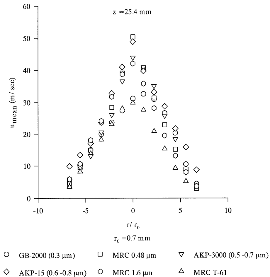
Fig. 10: Cold Flow Measurements of Mean Velocity for 1.4 mm (0.055 in.) Tube at 25.4 mm (1 in.) Axial Location
