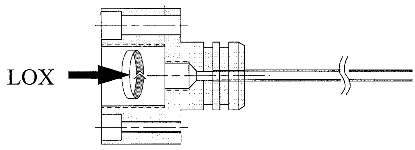
Swirl Coaxial Oxidizer Post (replaces center post above)
