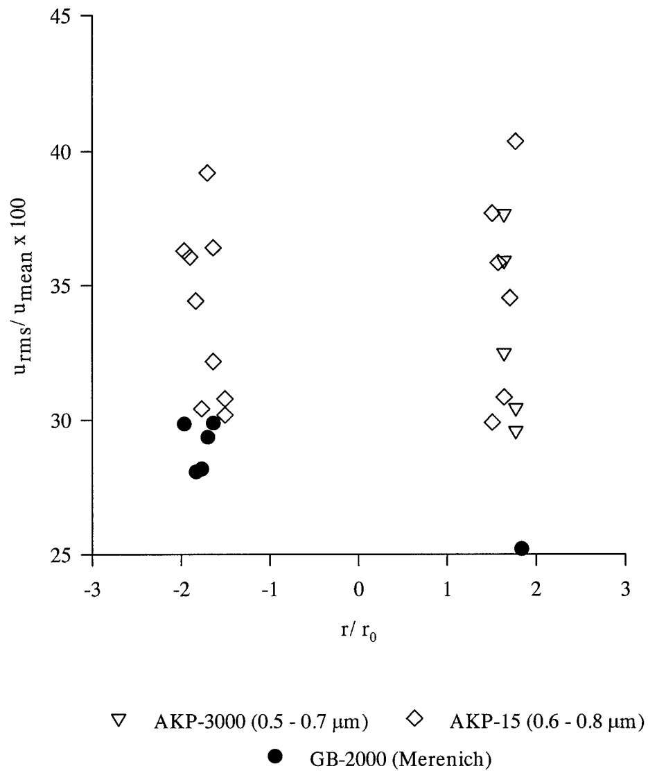
Fig. 18: Turbulence Level at 25.4 mm (1 in.) Axial Location Using AKP-15 (0.6 - 0.8 \mu\text{m} ) and AKP-3000 (0.5 - 0.7 \mu\text{m} )
