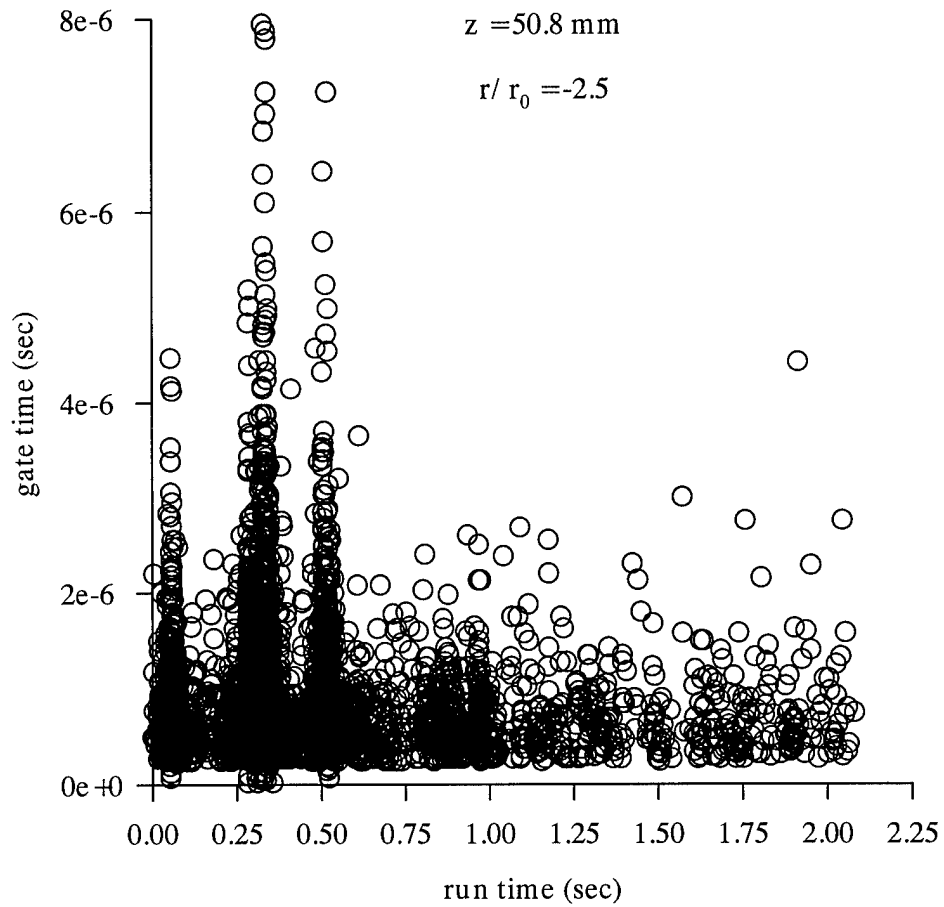
Fig. 38: Merenich Velocity Realization Bursts at 50.8 mm (2 in.) Axial Location, H 2 Seeded, r/r_0 = -2.5
