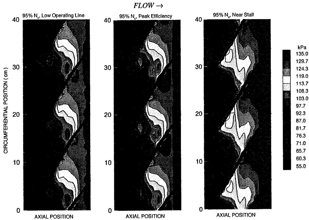
Figure 3.6 Rotor Tip Static Pressure Contours; 95% Design Speed
