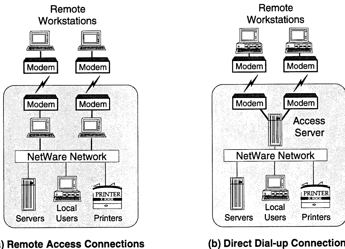
Figure 4-4. Dial-up Connections
