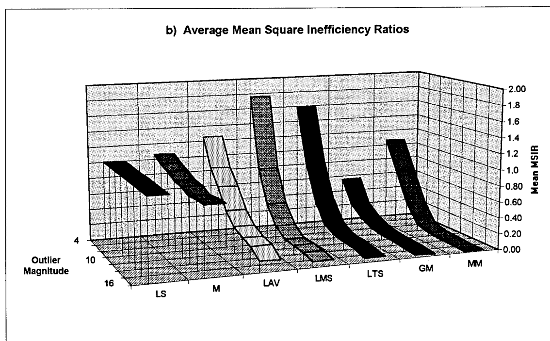
Figure 3.1. Pilot 1 Regression Technique Performance for Interior X-space Outliers in a) AMSEE and b) AMSIR
