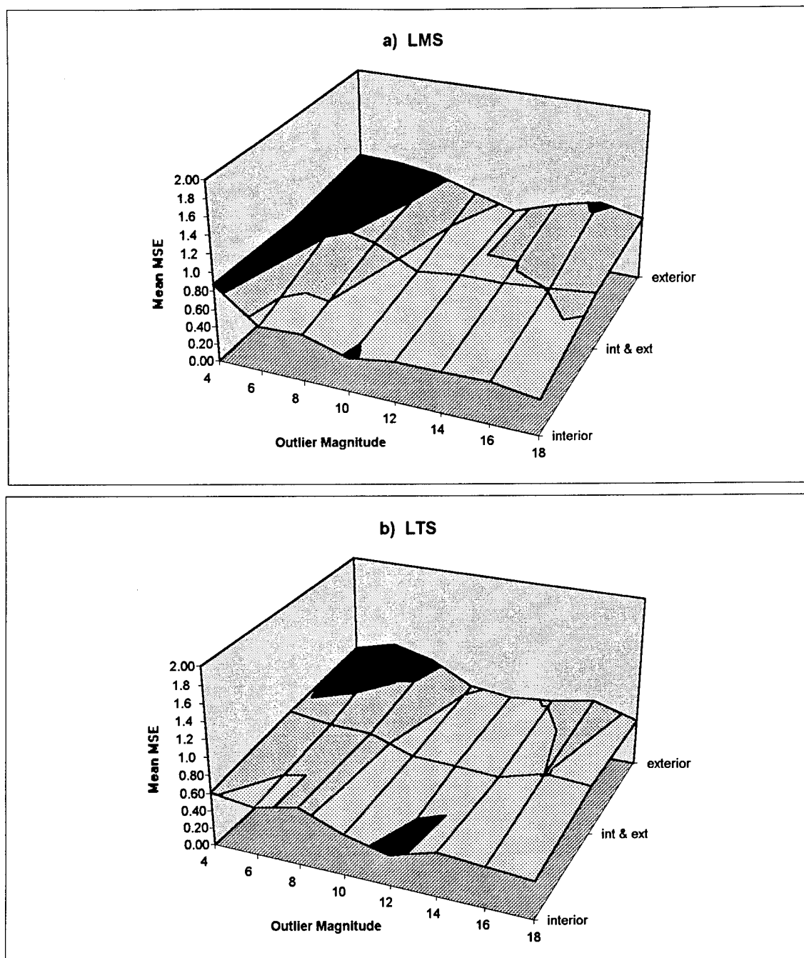
Figure 3.5. Pilot 1 Robust Regression Technique Overall Performance a) LMS and b) LTS
