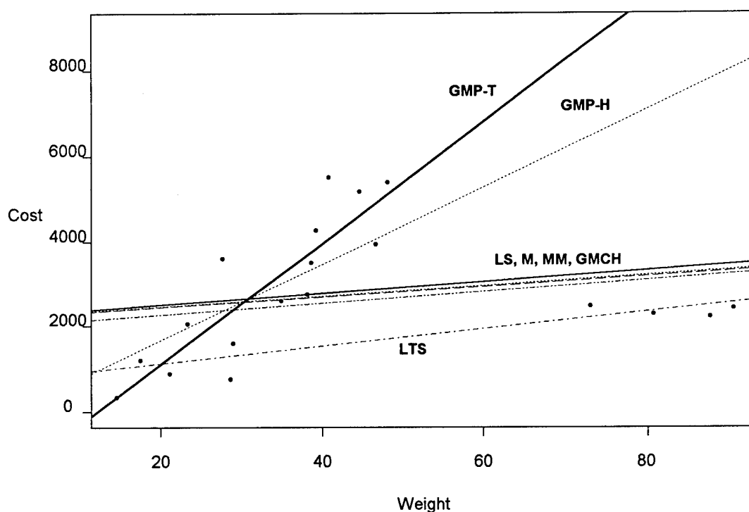
Figure 6.4. Satellite Cost Data with Robust Regression Estimates
