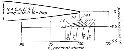
FIGURE 23.—Contours showing variation of Cl_{max}/C_{b_{min}} with flap position. Plain wing Cl_{max}/C_{b_{min}}=109.0 .
