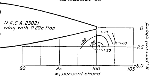
FIGURE 8.—Contours showing variation of C_{l_{max}} with flap position. \delta_f=20^\circ . Plain wing C_{l_{max}}=1.208 .
