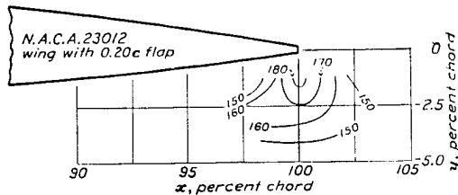
FIGURE 17.—Contours showing variation of Cl_{max}/C_{b_{min}} with flap position. Plain wing Cl_{max}/C_{b_{min}}=109.0 .
