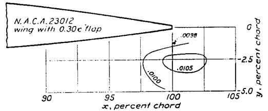
FIGURE 22.—Contours showing variation of Cb_{min} with flap position. Plain wing Cb_{min}=0.0105 .
