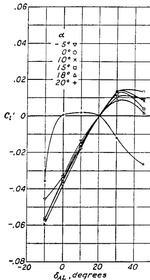
FIGURE 37.— C_l' , N. A. C. A. 23012 wing with external-airfoil flaps and ailerons (0.20 c flap). \delta_f = 20^\circ; \delta_{AR} = 20^\circ ; aileron span = b/4 .
