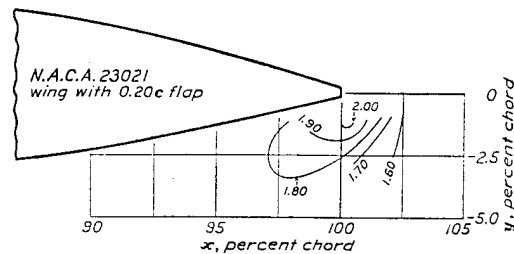
FIGURE 9.—Contours showing variation of C_{l_{max}} with flap position. \delta_f=30^\circ . Plain wing C_{l_{max}}=1.208 .
