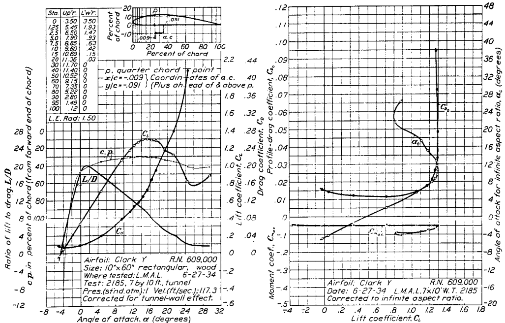
(b) Wooden airfoil
