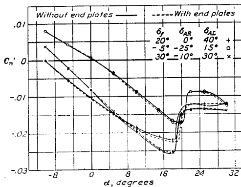
FIGURE 32.— C_n , N. A. C. A. 23012 wing with external-airfoil flaps and ailerons (0.20 c flap). Aileron span = b/4 .
