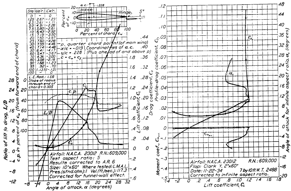
FIGURE 27.—The N. A. C. A. 23012 airfoil with 0.20 c Clark Y flap, \delta_f = 5^\circ .
