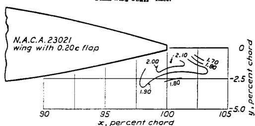
FIGURE 10.—Contours showing variation of C_{l_{max}} with flap position. \delta_f=40^\circ . Plain wing C_{l_{max}}=1.208 .
