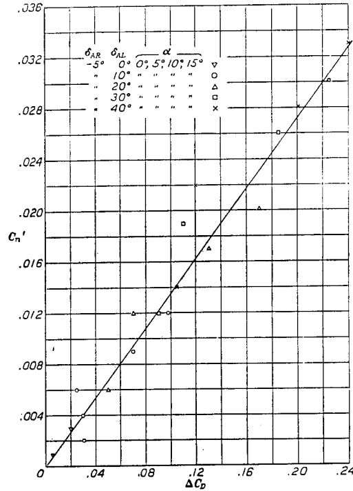
FIGURE 44.— C_n' against \Delta C_D , N. A. C. A. 23012 wing with 0.20 c Clark Y external-airfoil flaps deflected as ailerons. Aileron span = b/2 .
