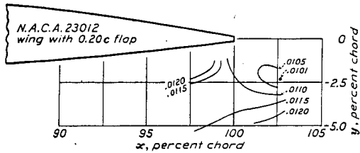
FIGURE 16.—Contours showing variation of Cb_{min} with flap position. Plain wing Cb_{min}=0.0105 .
