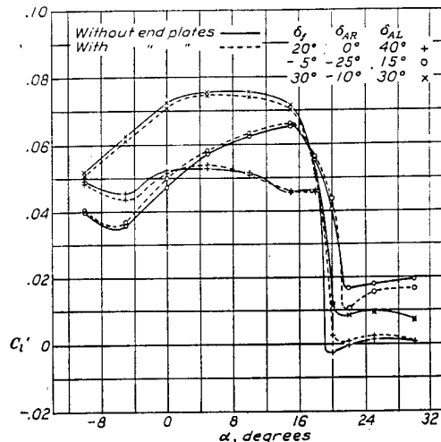
FIGURE 31.— C_l , N. A. C. A. 23012 wing with external-airfoil flaps and ailerons (0.20 c flap). Aileron span = b/4 .
