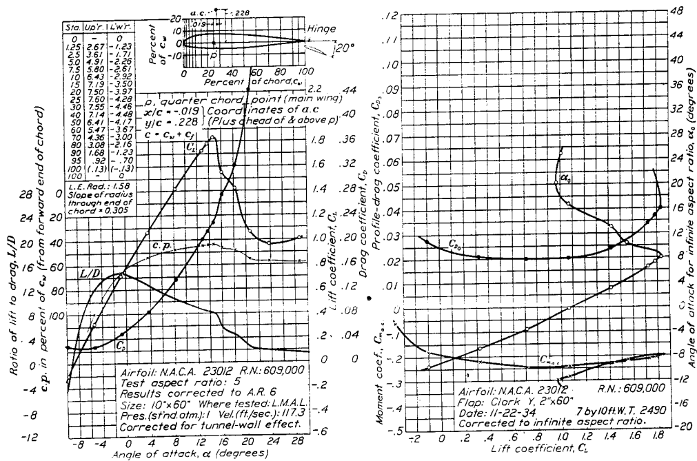
FIGURE 28.—The N. A. C. A. 23012 airfoil with 0.20 c Clark Y flap, \delta_f = 20^\circ .
