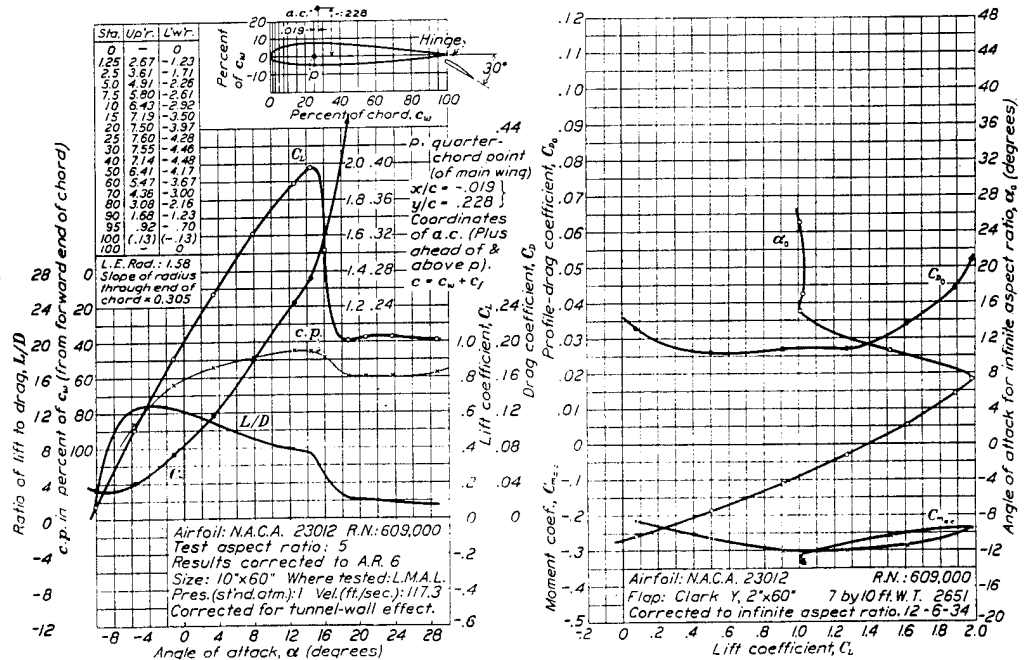
FIGURE 20.—The N. A. C. A. 23012 airfoil with 0.20 c Clark Y flap, \delta_f = 30^\circ .
