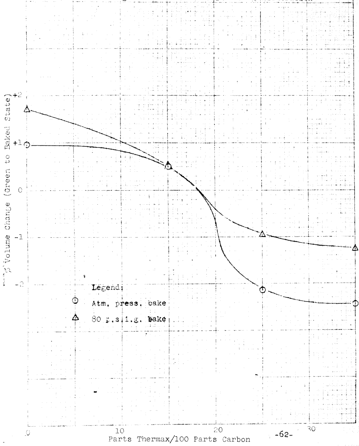
% Volume Change as a Function of Thermax Concentration
