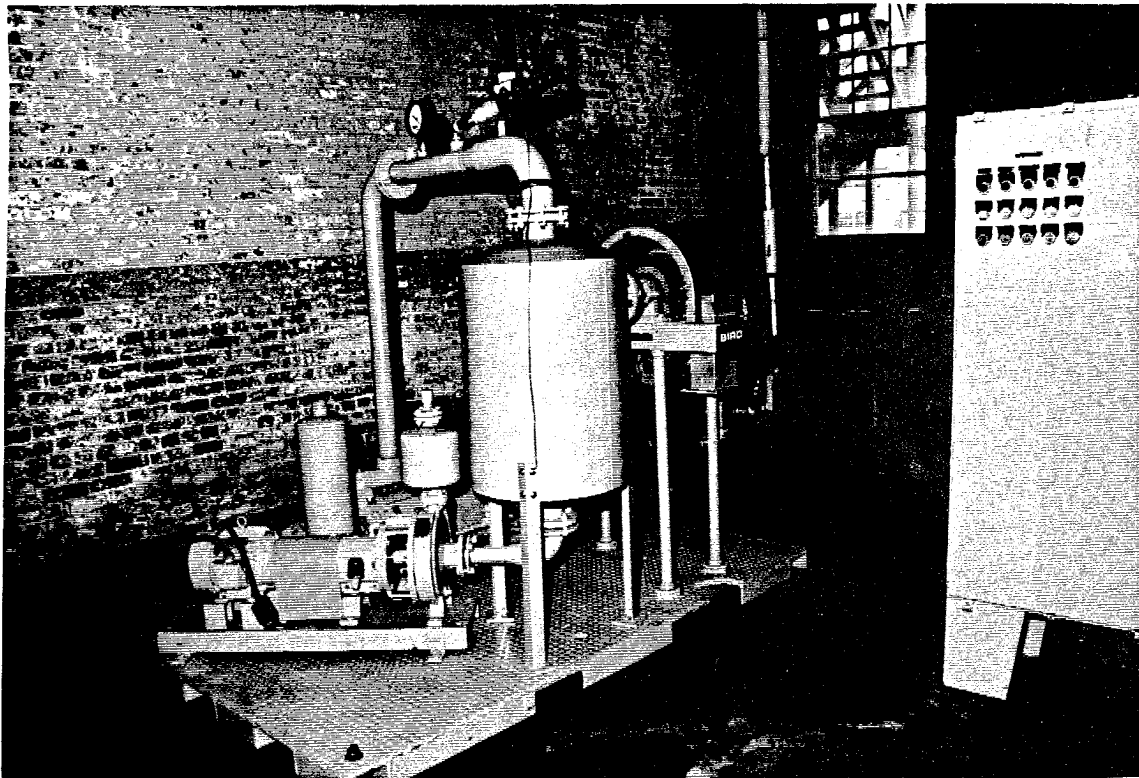
Figure 21. Pumps and tanks associated with the Bird rotary vacuum filter.
