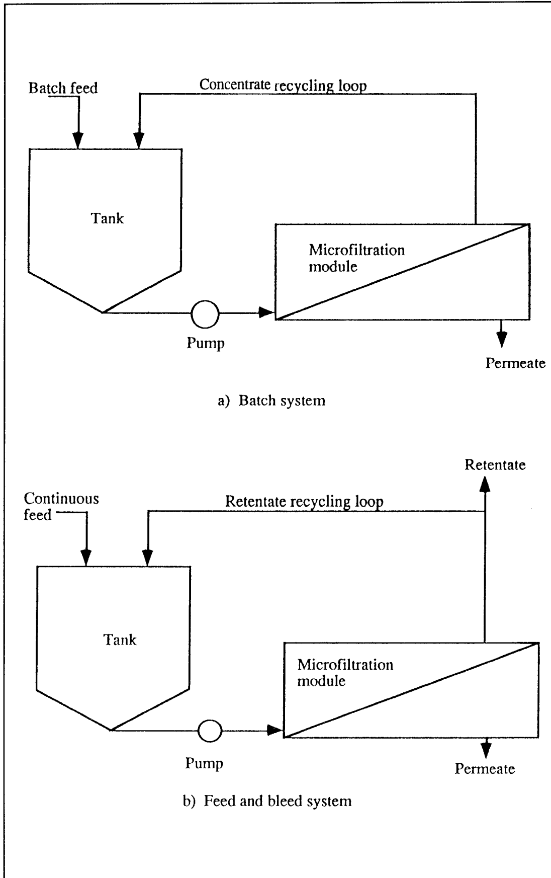
Figure 2. Types of filtration systems.
