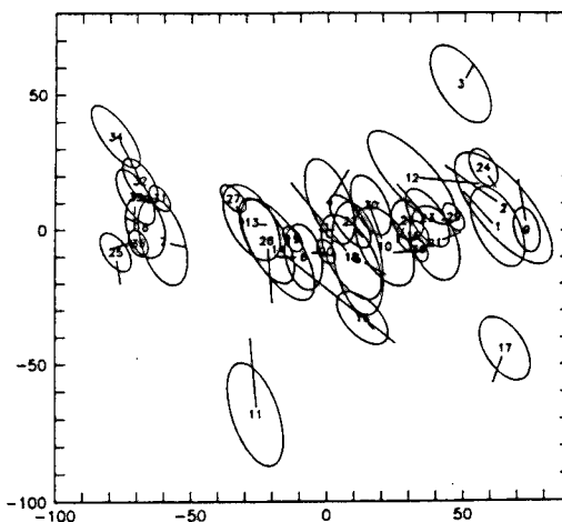
Fig. 3b. Relative locations of earthquakes on the western portion of the St. Paul's transform (ISC locations west of 29^\circ\text{W} ).
