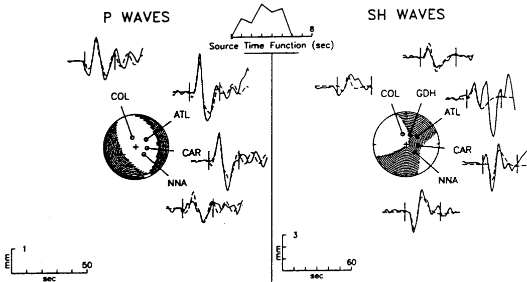
Fig. A14. Observed P and SH waveforms from the earthquake of September 21, 1977, compared with synthetic waveforms generated from the best fitting point source model found from body waveform inversion. See Figure A1 for further details.
