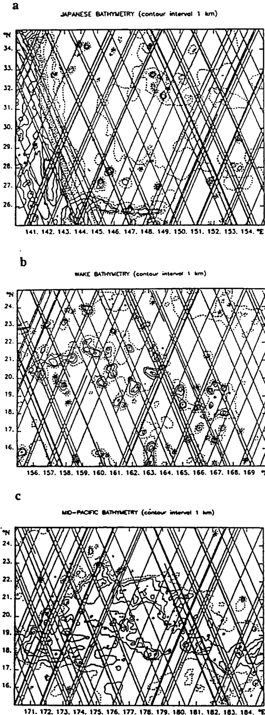
Fig. 3. Seasat tracks over the Darwin Rise. Dashed contours show depths equal to and below 5 km. (a) Japanese Seamounts. (b) Wake Guyots. (c) Mid-Pacific Mountains.
