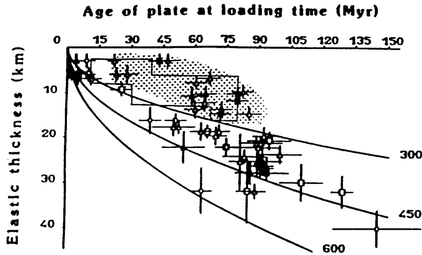
Fig. 1. Figure adapted from Calmont and Cazanave [1987]. Elastic plate thicknesses from volcanoes in the Atlantic (squares), Pacific (triangles), and Indian (diamonds) oceans plotted against estimated age at the time of loading. Isotherms calculated from Parsons and Sclater [1977]. Stippled area outlines the superswell volcanoes. The polygon represents the range of values derived from modeling shipborne gravity over the Japanese and Wake seamounts.
