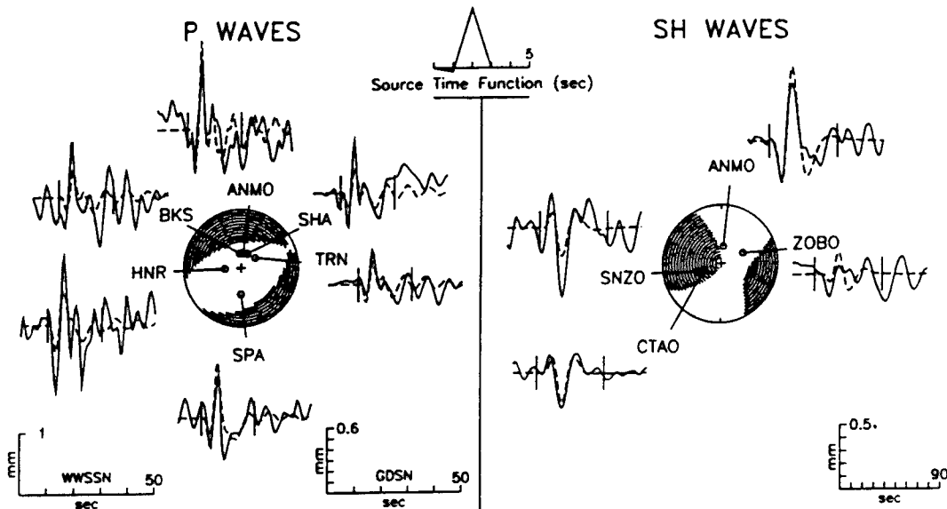
Fig. A13. Observed P and SH waveforms from the earthquake of May 15, 1987, compared with synthetic waveforms generated from the best fitting point source model found from body waveform inversion. CTAO and ANMO are GDSN stations. See Figure A1 for further details.
