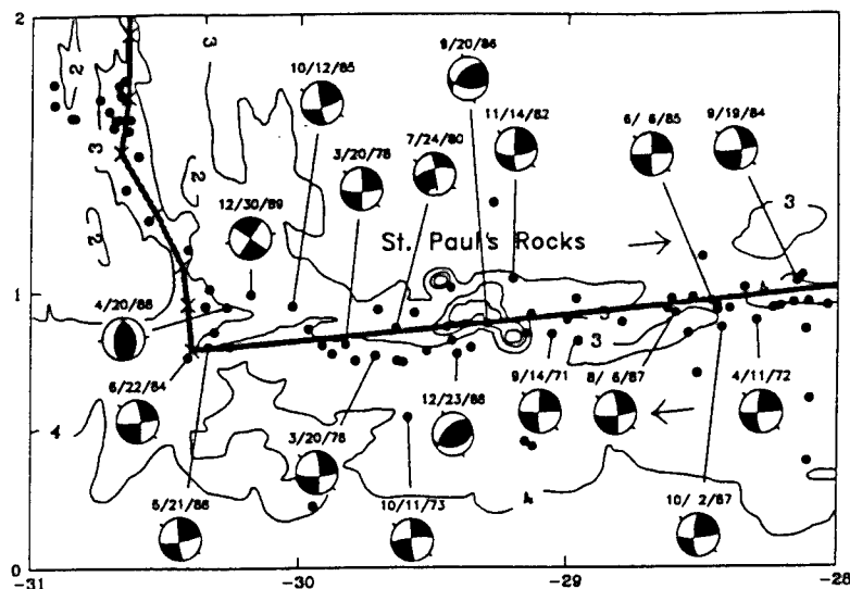
Fig. 5. Earthquake locations and mechanisms along the western portion of the St. Paul's transform. Bathymetric contours are from the General Bathymetric Chart of the Oceans (GEBCO) Digital Atlas, as supplied by the British Oceanographic Data Centre, Bidston, England, March 1992; 1-km contour interval, Mercator projection. The location of the December 30, 1989, event is from the ISC. Mechanisms of earthquakes on October 11, 1973; November 14, 1982; October 12, 1985; September 20, 1986; April 20, 1988; and December 23, 1988, are from this study. Mechanisms of the events on September 14, 1971, and April 11, 1972, are from Engeln et al. [1986]. Mechanisms of other events are taken from the Harvard CMT catalogue. Crosses show the location of the Mid-Atlantic Ridge and its intersection with the St. Paul's transform, as given by J.-G. Schilling (Lamont-Doherty Earth Observatory, unpublished cruise report, 1987). The transform boundary is taken as a small circle about the South American-African Euler vector [DeMeis et al., 1990]. See Figure 4 for further details.
