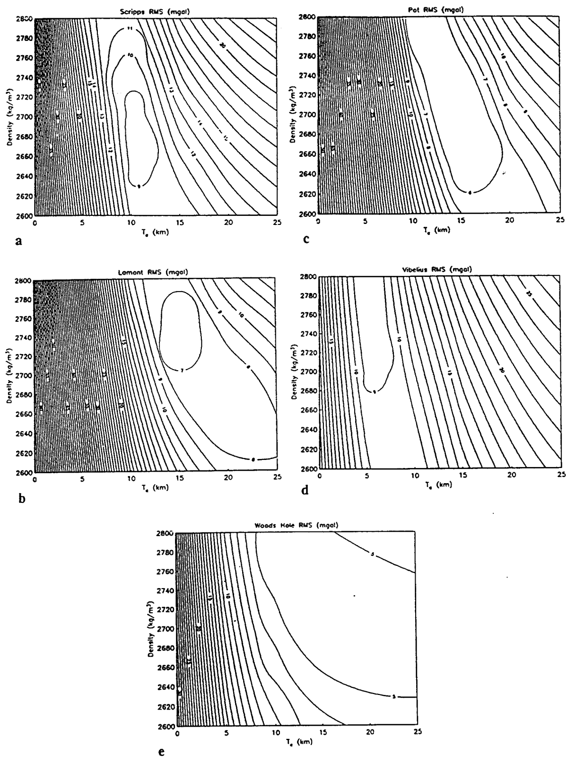
Fig. 11. Contour maps of RMS misfit between real and synthetic gravity lines gridded against the parameters of elastic plate thickness and density for five seamounts in the Wake group. (a) Scripps. (b) Lamont. (c) Pot. (d) Vibelius. (e) Woods Hole.
