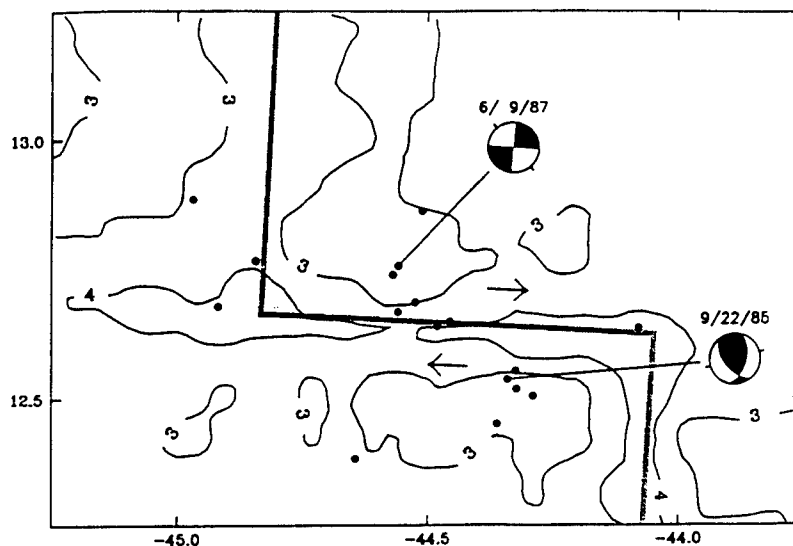
Fig. 6. Earthquake locations and mechanisms along the Marathon transform. Bathymetry is from Collette et al. (1984); 1-km contour interval, Mercator projection. The mechanism of the September 22, 1985, earthquake is from this study. The June 9, 1987, mechanism is from the Harvard CMT catalogue. The transform boundary is taken as a small circle about the South American-African Euler vector [DeMets et al. , 1990]. See Figure 4 for further details.
