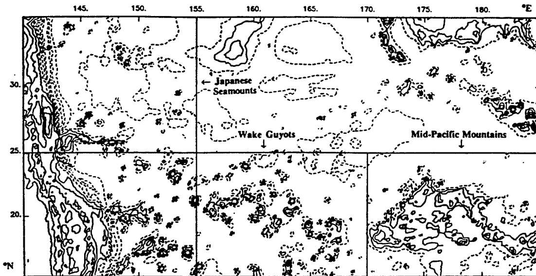
Fig. 2. Bathymetry of the Darwin Rise, taken from dbdh5 data, showing the location of the Japanese Seamounts, Wake Guyots, and Mid-Pacific Mountains. Contour interval is 1 km. Dashed contours show depths equal to and below 5 km.
