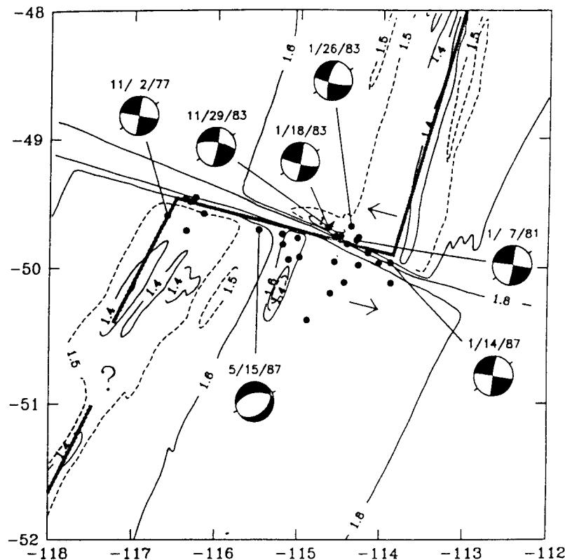
Fig. 9. Earthquake locations and mechanisms along the Menard transform. Bathymetry is adapted from Mammerickx et al. [1975]; contours are in thousands of fathoms, with a 100-fathom contour interval and the 1500-fathom contour dashed. The mechanism of the May 15, 1987, earthquake is from this study. Other earthquake mechanisms are from the Harvard CMT catalogue. The transform boundary is taken as a small circle about the Pacific-Antarctic Euler vector [DeMets et al. , 1990]. See Figure 4 for further details.
