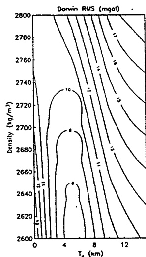
Fig. 12. Contour map of RMS misfit between real and synthetic gravity lines gridded against the parameters of elastic plate thickness and density for Darwin seamount in the Mid-Pacific group.
