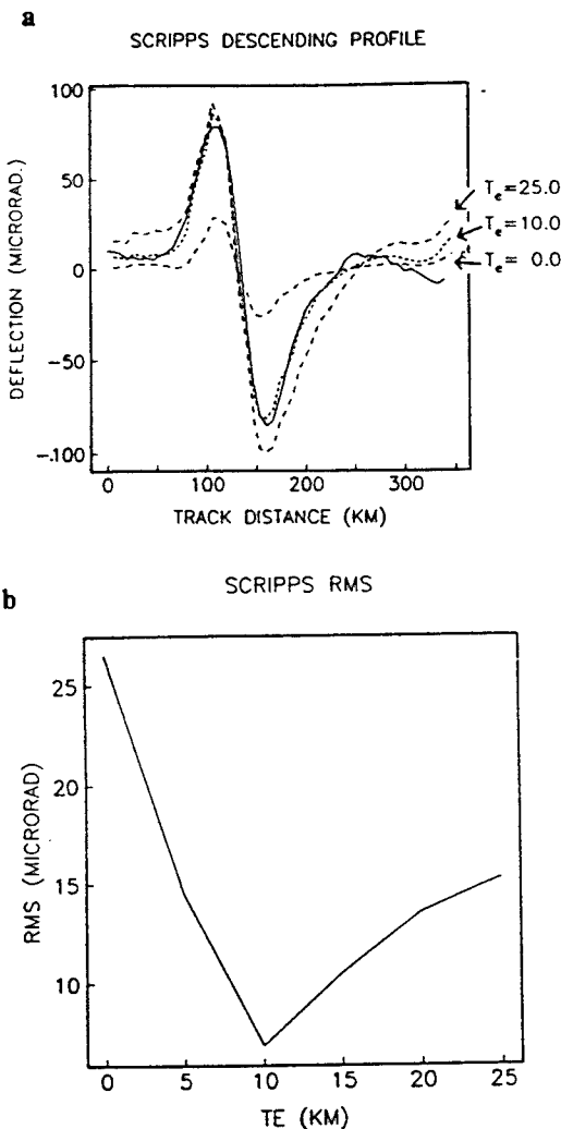
Fig. 5. (a) Deflection of the vertical over Scripps seamount. Descending Seast track is shown as a straight line. Synthetics for T_e = 0, 10 , and 25 km are shown as dashed lines. (b) RMS misfit between observed and calculated deflection of the vertical plotted against the elastic plate thickness parameter.
