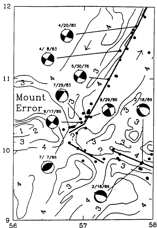
Fig. 4. Earthquake locations and mechanisms along the southwestern portion of the Owen transform. Bathymetry is adapted from Cochran [1988]: 1-km contour interval. Mount Error is at about 10.3°N, 56.2°E and reaches depths of < 1 km. The southeastern portion of Error Ridge includes both Mount Error and the elongate high at about 11°N, 56.2°E. Suggested plate boundary geometry is shown as a stippled line; question marks show portions of the boundary where the geometry is poorly constrained. The northeastern transform boundary is taken as a small circle about the African-Indian Euler vector, and arrows denote relative plate motion directions [DeMets et al. , 1990]. Epicenters (solid circles) are of relocated events from January 1964 to March 1989. The mechanisms of the earthquakes of July 29, 1983, and July 7, 1986, are from this study. All other mechanisms are from the Harvard CMT catalogue. Tick marks denote the azimuth of the maximum compressive horizontal stress, under the assumption that the P axis and T axis correspond to the axes of maximum and minimum principal stress, respectively. This assumption may not always be valid [McKenzie, 1969].
