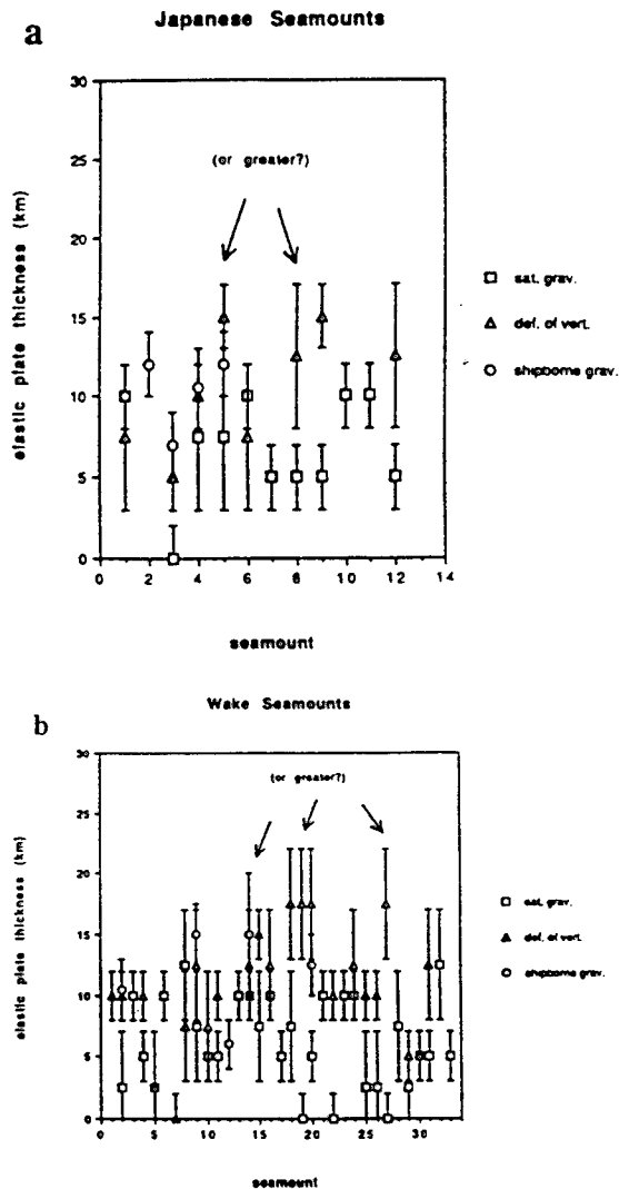
Fig. 6. Elastic plate thicknesses of Darwin Rise guyots obtained from the study of satellite gravity, satellite deflection of the vertical, and shipborne gravity. See Table 2 for locations of seamounts plotted in figures. (a) Japanese Seamounts, including those surveyed on Roundabout leg 10: 1, Takuyo-Daini and Seiko; 2, Winterer; 3, Stout and Thomas Washington; 4, Isakov; and 5, Makarov. (b) Wake Guyots, including those surveyed on Roundabout leg 10: 2, Scripps; 9, Lamont; 12, Vibelius; 14, Woods Hole; and 20, Fox. (c) Mid-Pacific Mountains, including Darwin (2), surveyed on Roundabout leg 10.
