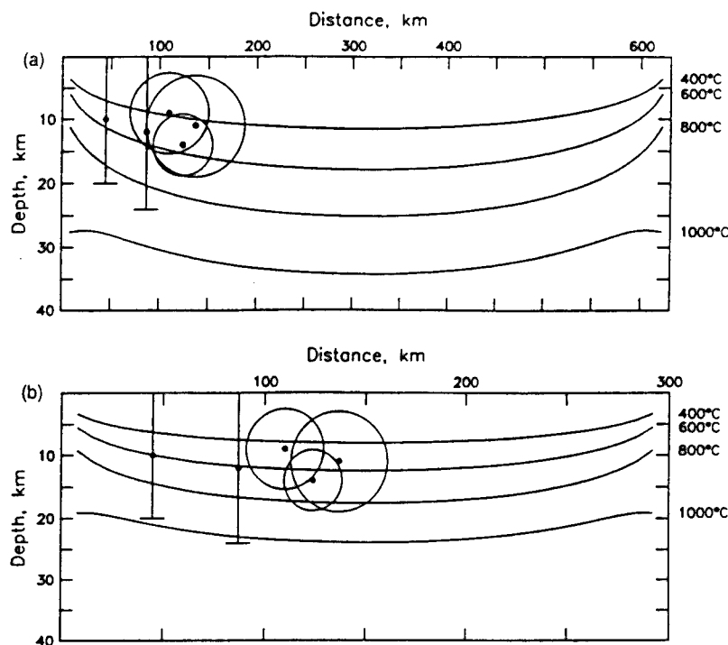
Figure 11. Centroid depths of earthquakes along the St. Paul's transform. (a) Thermal model derived for an offset of 630 km and an age difference of 39 Ma. (b) Thermal model derived for an offset of 300 km and an age difference of 19 Ma. Circles denote the areal extent of faulting for a circular fault model. Vertical bars denote a depth extent of faulting that is twice the centroid depth. See text for further details.
